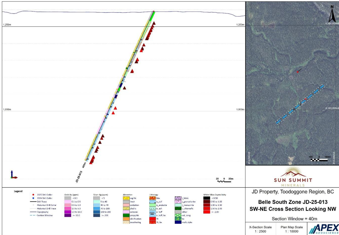
Figure 10.11 Cross Section JD-25-013
