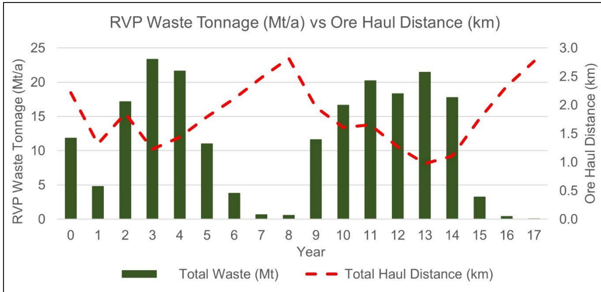
Figure 1.7: Weight Averaged Haul Distances – Total Mine Waste
