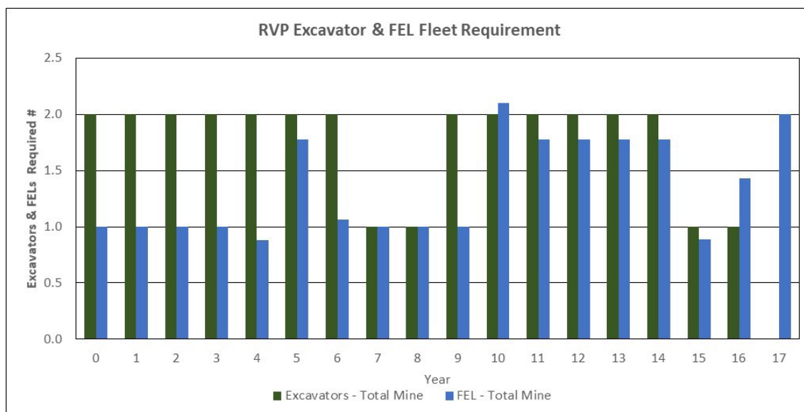
Figure 1.6: LOM Excavator and FEL Fleet
