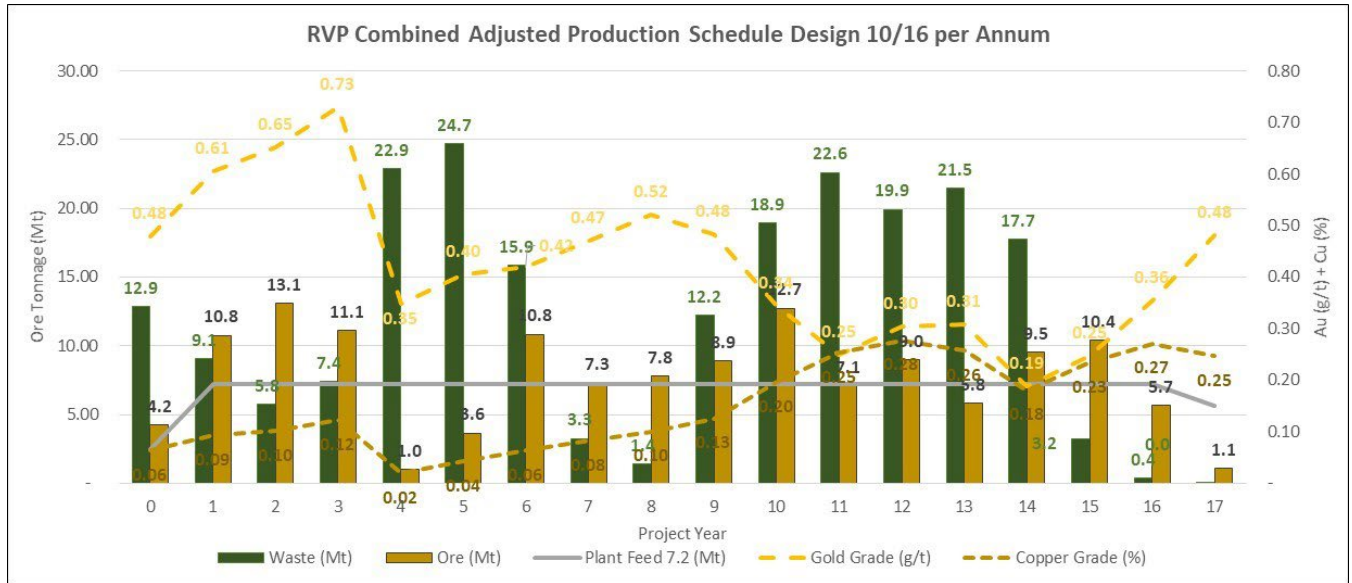
Figure 1.5: Total Project Material Movements for LOM
