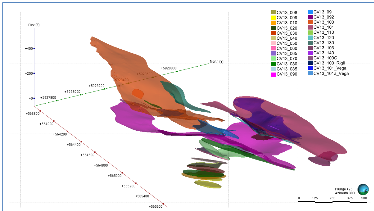
Figure 14.5: Mineralized Zones of CV13
