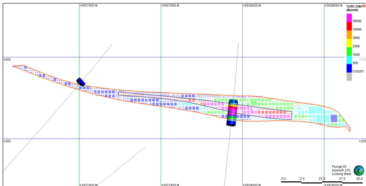
Figure 14.15: CV13 Comparison (composites vs block model \text{Cs}_2\text{O} ; CV13_100 with Rigel Cs-enriched zone)
