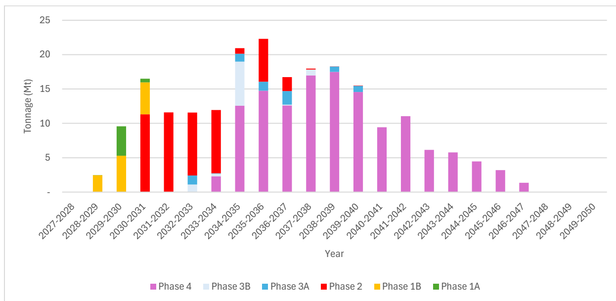
Figure 16.17: Open Pit Mining Schedule by Phase (without stockpile reclaim)
