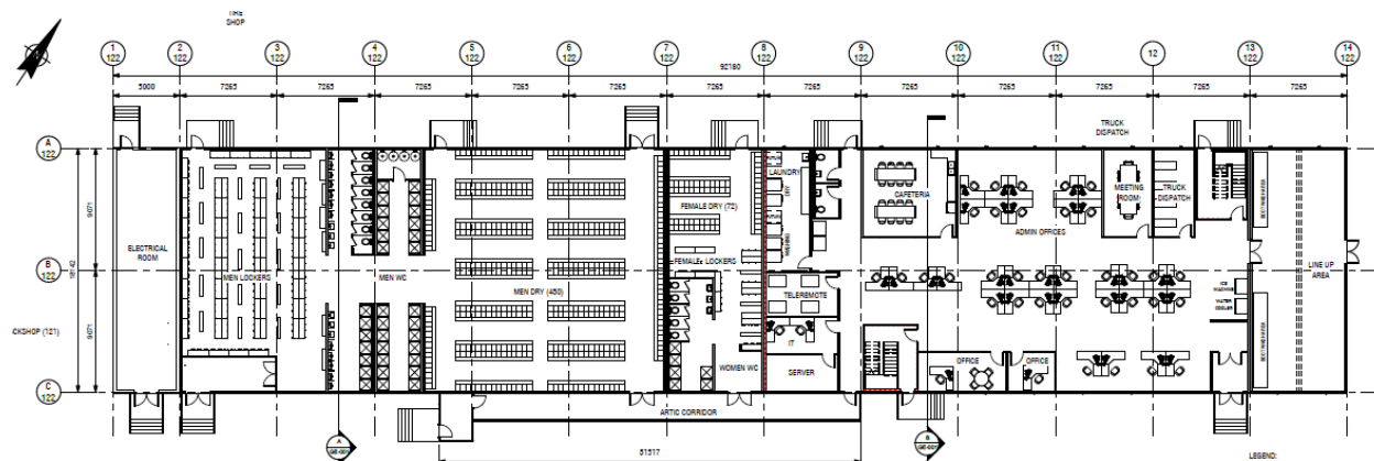
Figure 18.15: Dry & Mine Administrative Building - Plan View
