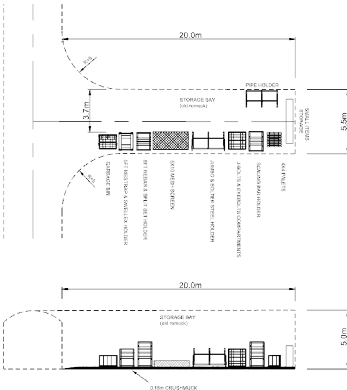
Figure 16.66: Typical Layout of Underground Storage (utilizing an existing excavation)
