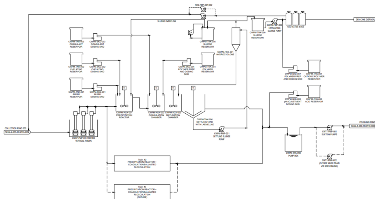
Figure 18.44: General Process Flow Diagram
