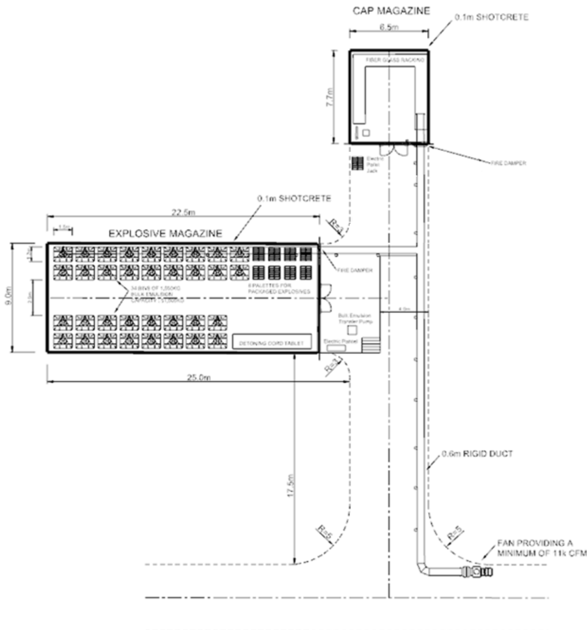
Figure 16.68: Typical Explosives Storage and Handling Facilities
