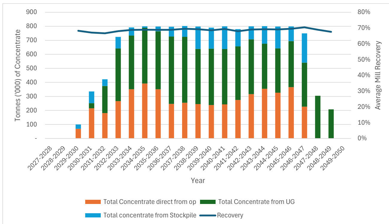
Figure 16.76: Spodumene (5.5%Li 2 O) Concentrate Production
