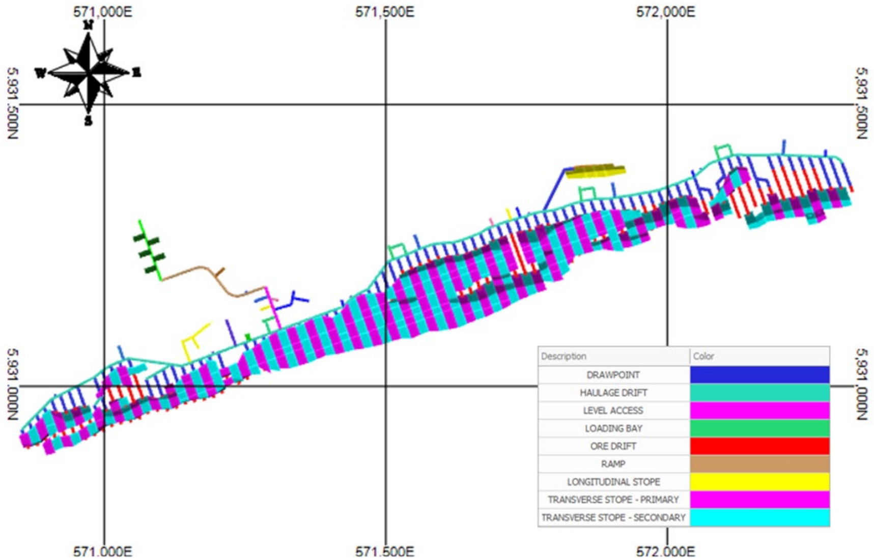
Figure 16.37: Typical Larger Level - Plan View
