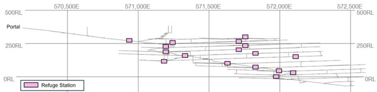
Figure 16.72: Underground Refuge Stations Location – Section Looking North
