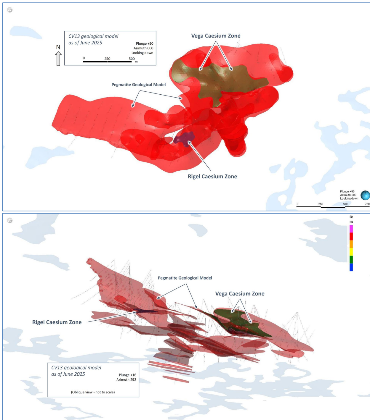
Figure 7.20: Plan View of CV13 Pegmatite Geological – All Lenses (top); Oblique View of CV13 Pegmatite Geological Model – All Lenses (bottom)
