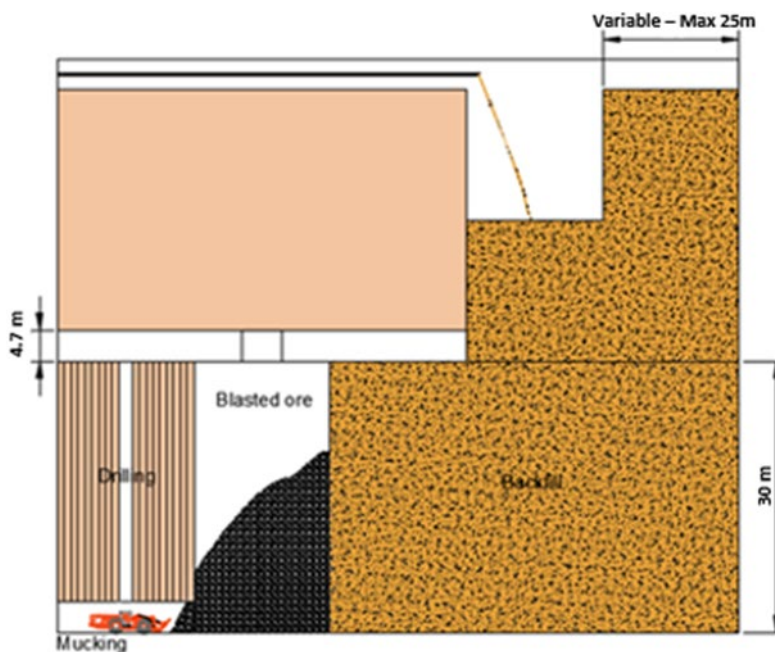
Figure 16.30: Representation of Longitudinal Mining Method
