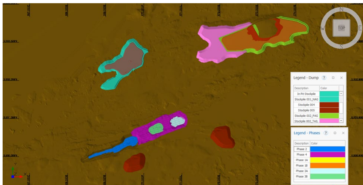
Figure 16.22: Mine Development End of Q2 2033 – Plan View
