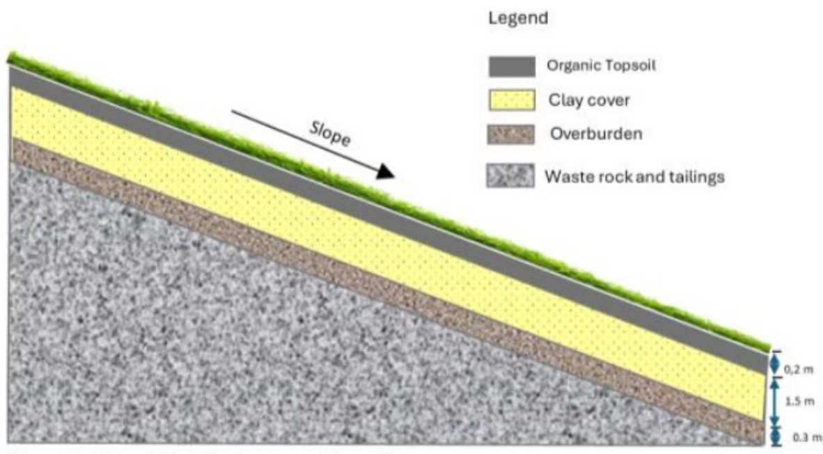
Figure 20.2: Stockpile 002 Closure Configuration
