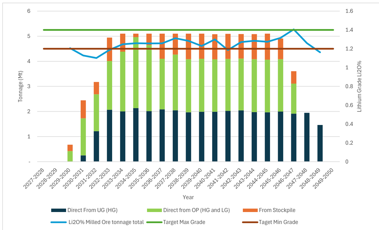
Figure 16.75: Ore Processing by Source Material
