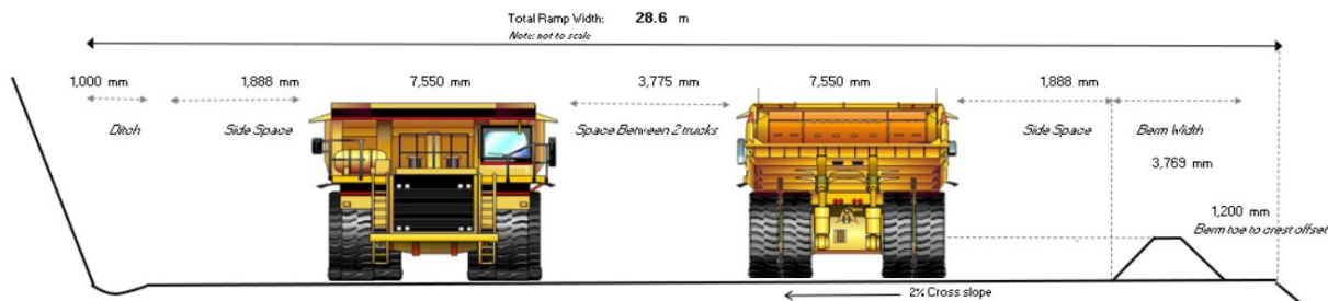
Figure 15.7: Double-Lane Ramp Design Criteria
