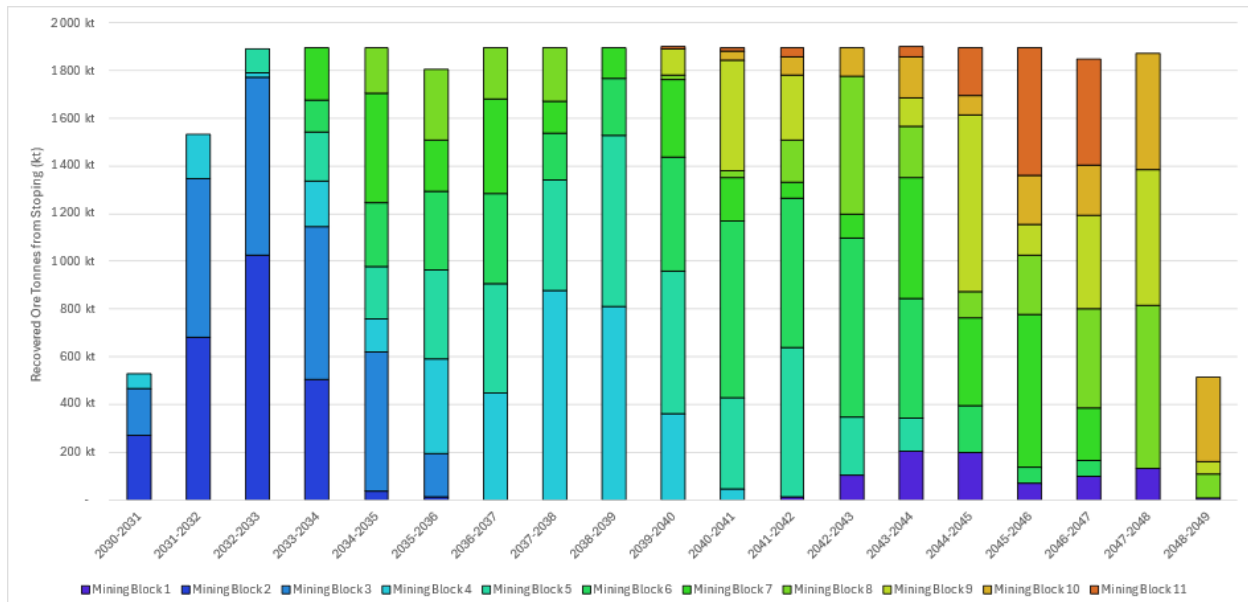
Figure 16.52: Underground Mine Recovered Ore Tonnes from Stopping Split by Mining Block
