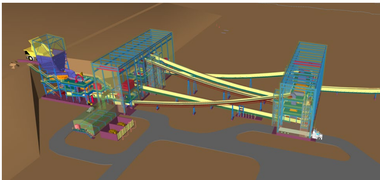
Figure 18.22: Primary Crushing, Secondary and Tertiary Crushing, Screening Buildings
