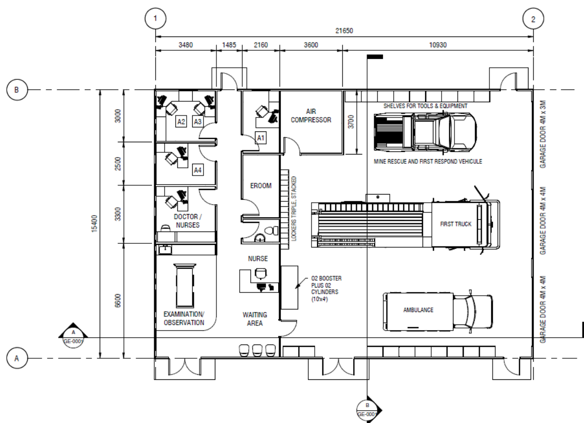
Figure 18.8: Fire Hall & Clinic, Plan View
