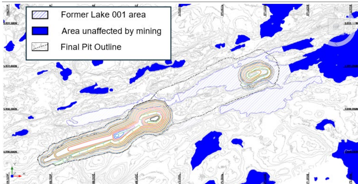
Figure 16.11: Phase 3A Open Pit Design – Plan View
