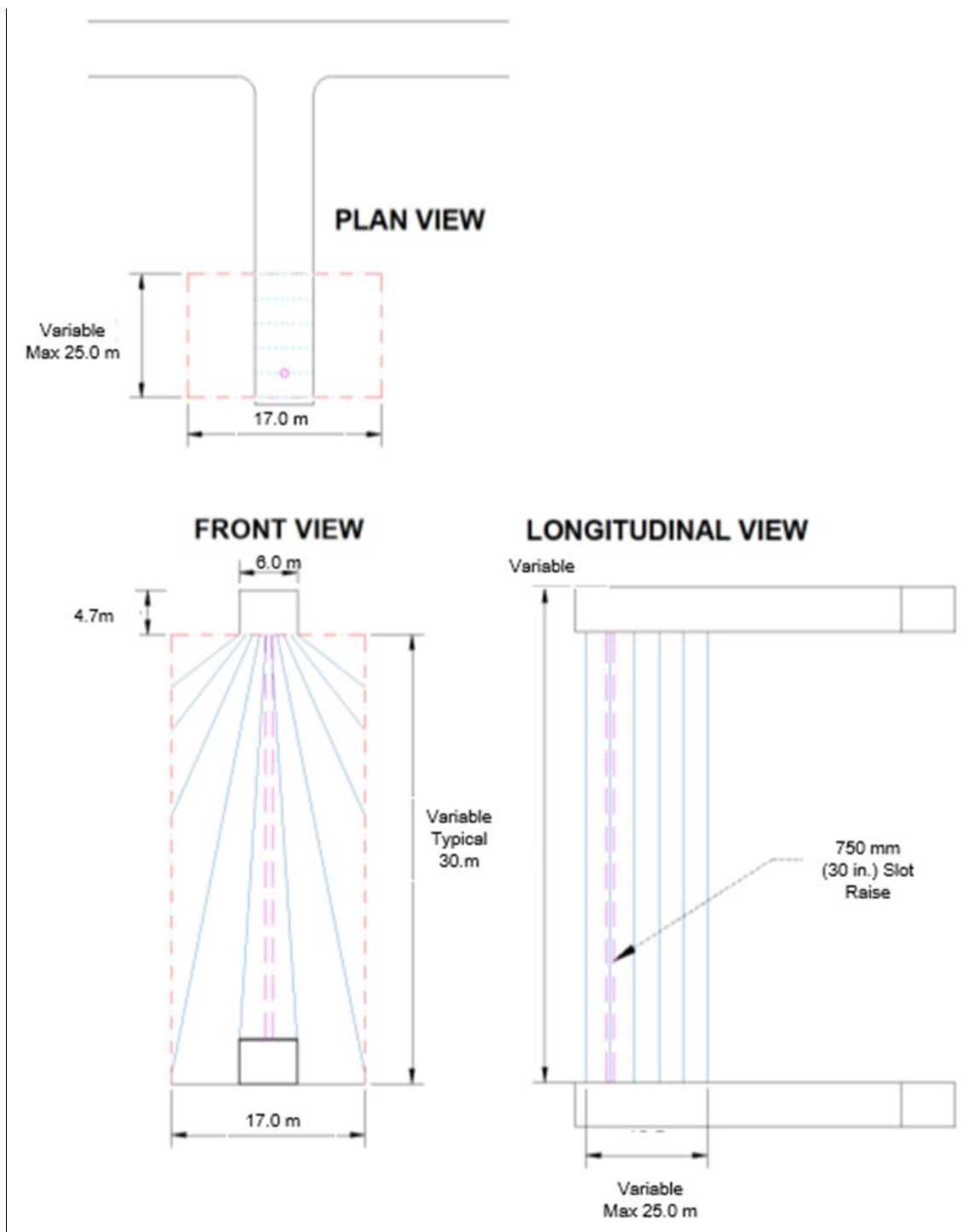
Figure 16.50: Typical Drilling Section for Underground Stopping
