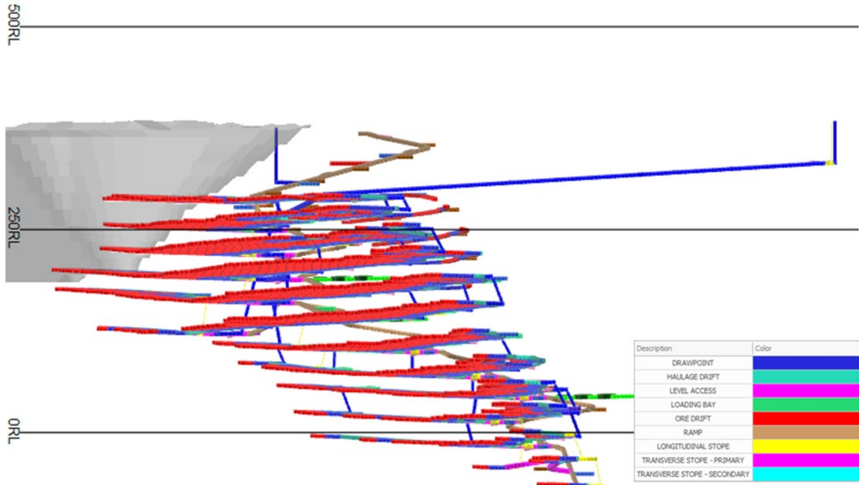
Figure 16.39: Mine Development Longitudinal View - Looking West
