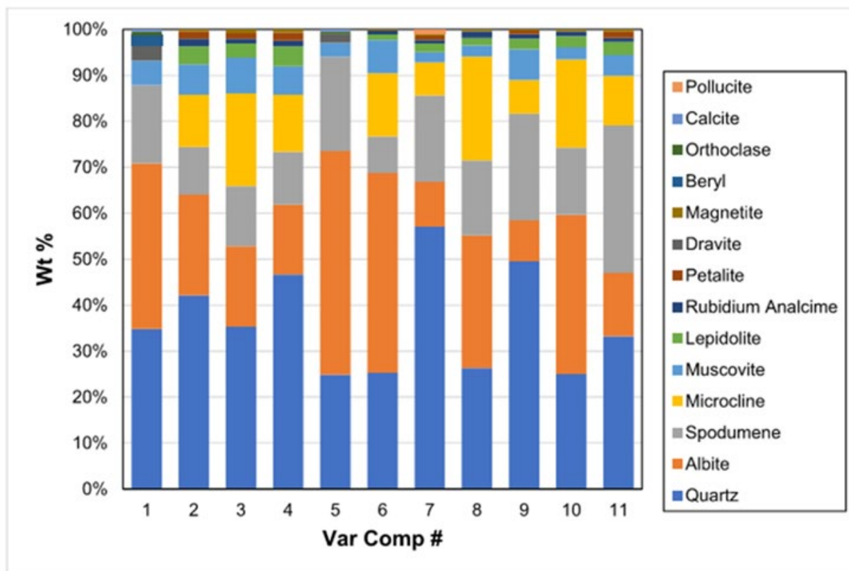
Figure 13.4: XRD Results on Variability Composite Samples
