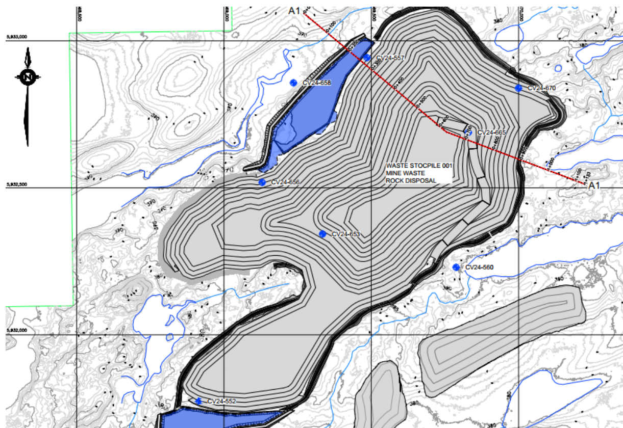
Figure 18.33: Layout of Critical Sections for Slope Stability Analysis – Waste Rock Stockpile 001 Cross Section A1-A1
