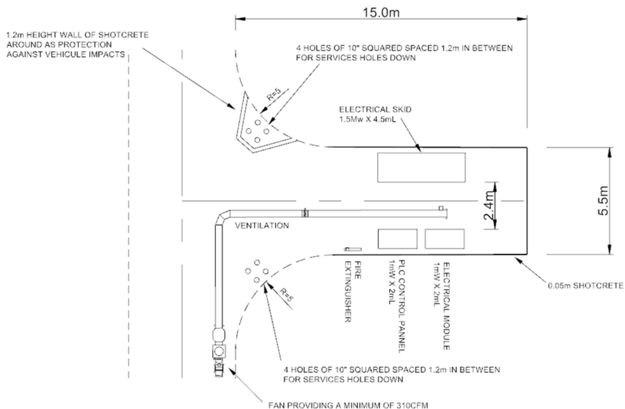
Figure 16.60: Typical Plan View of Electric Bay
