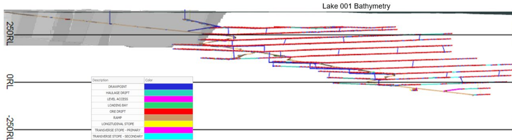
Figure 16.40: Underground Mine Development Longitudinal View - Looking North
