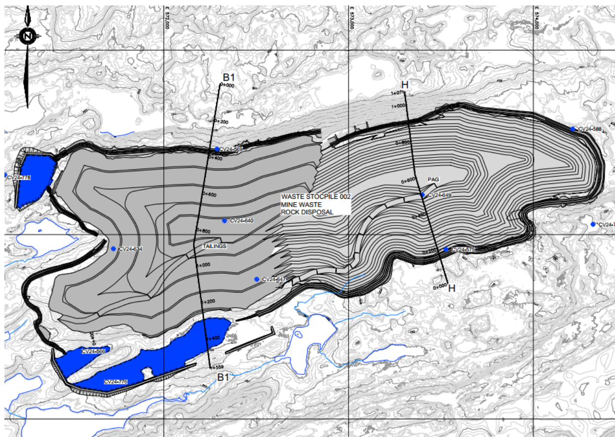
Figure 18.30: Stockpile 002 Critical Sections for Stability Analysis
