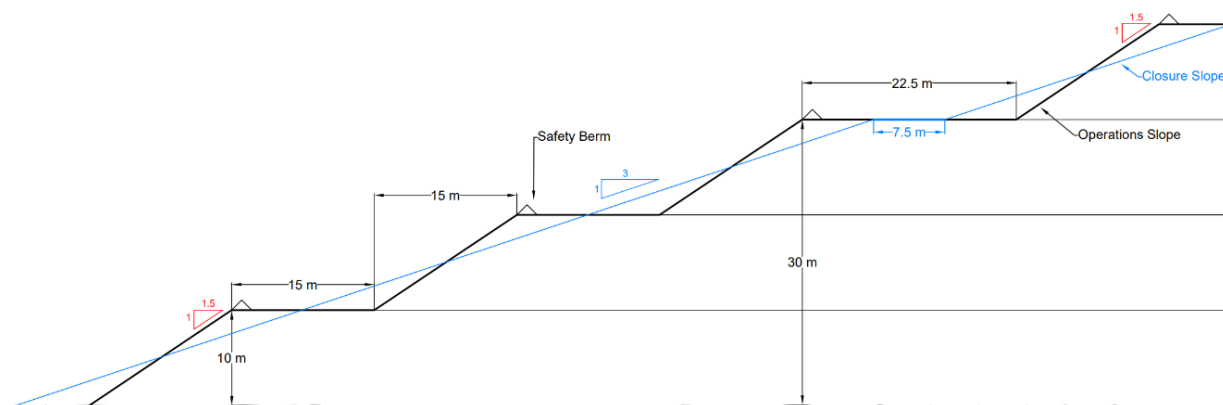
Figure 18.31: Typical Section for Waste Rock in Stockpiles 001 and 002 Showing Intermediate Benches for Both Operation and Closure Stages
