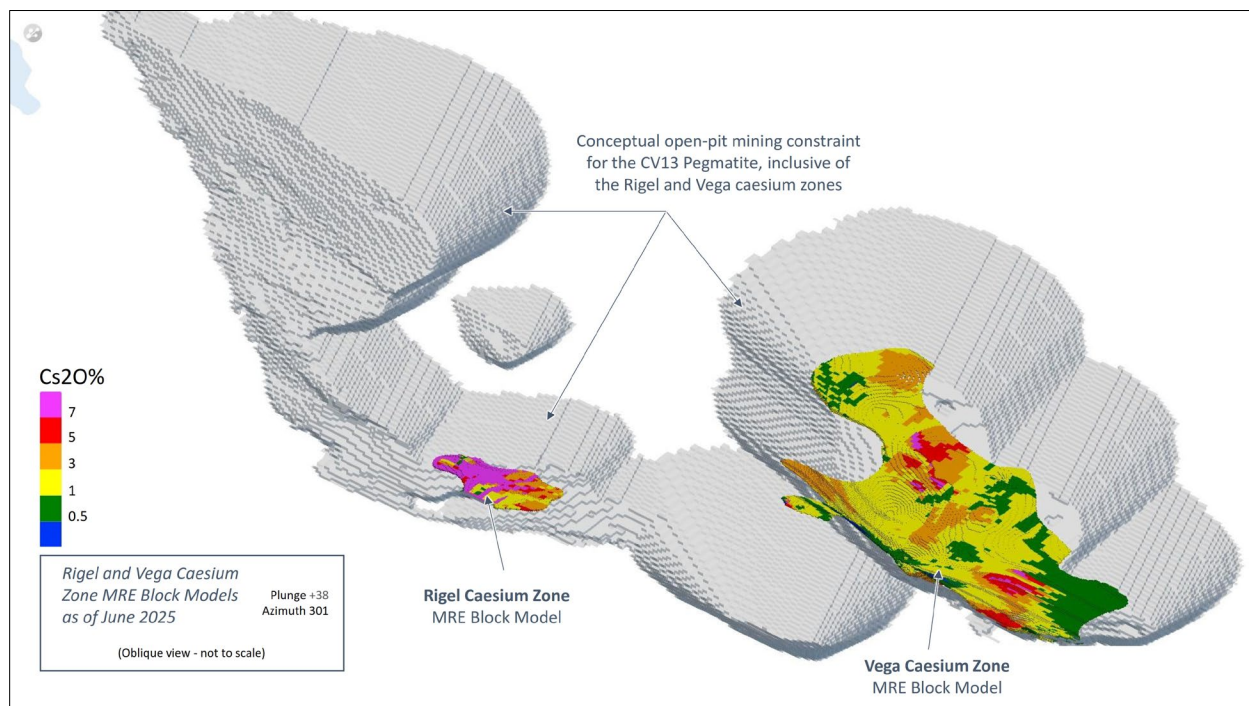
Figure 14.11: CV13 Open Pit Constraint to Rigel and Vega Caesium Zone MRE Block Model
