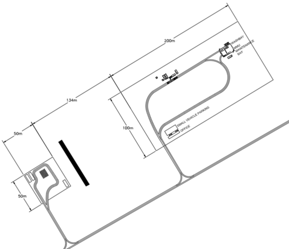
Figure 18.19: Explosive Storage Area
