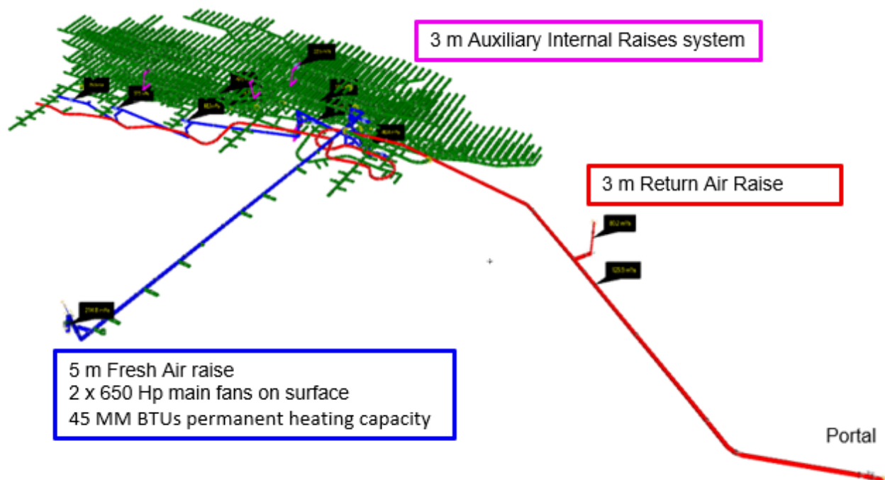
Figure 16.58: Underground Mine Ventilation Network – Permanent Set-up – Isometric View from North-West
