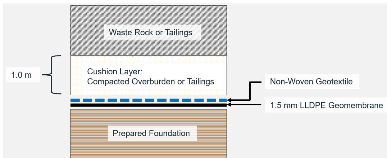
Figure 18.27: Typical Lined Base Stockpile 002
