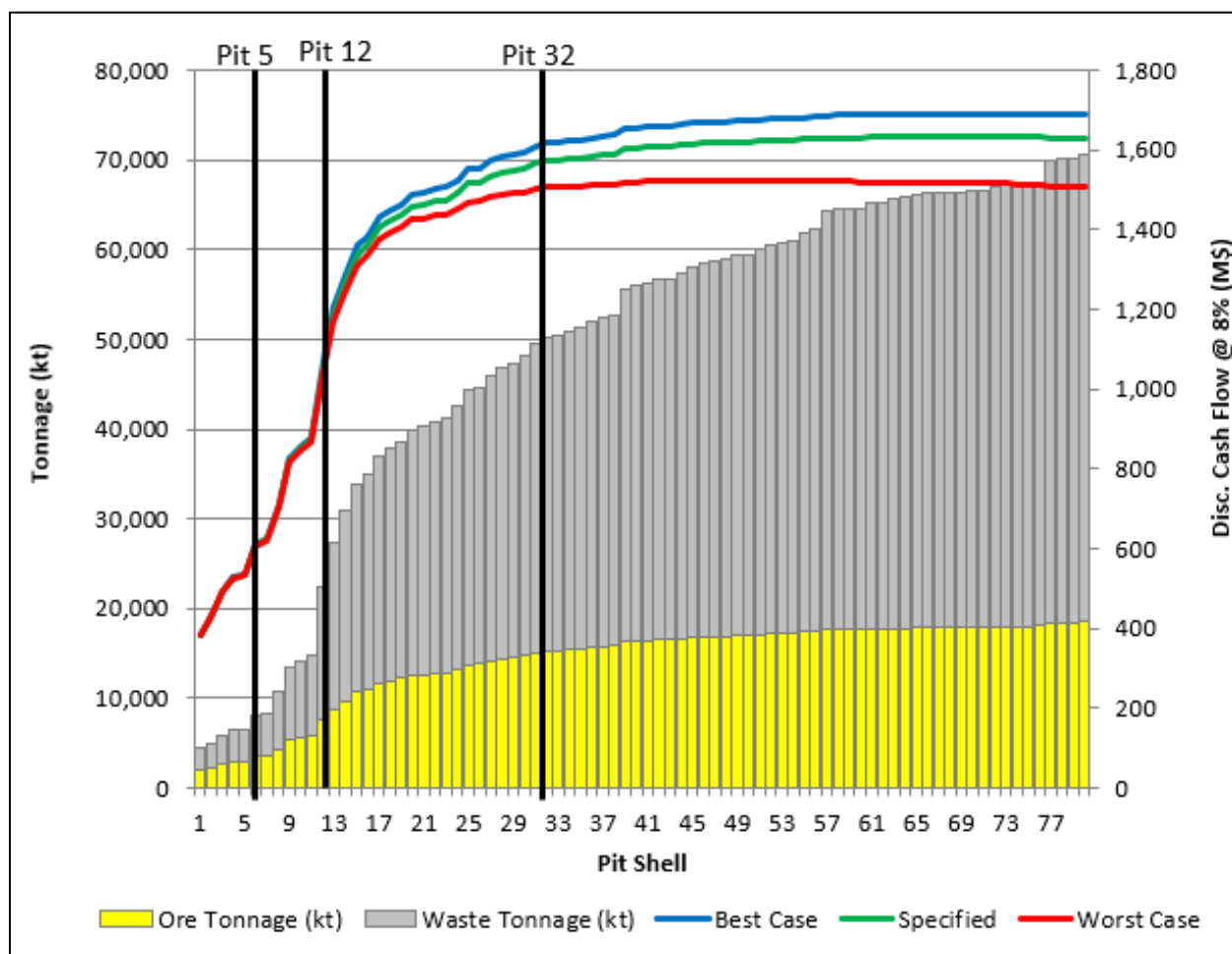
Figure 15.3: M&I Pit by Pit Results @ USD 1,303/t Conc.
