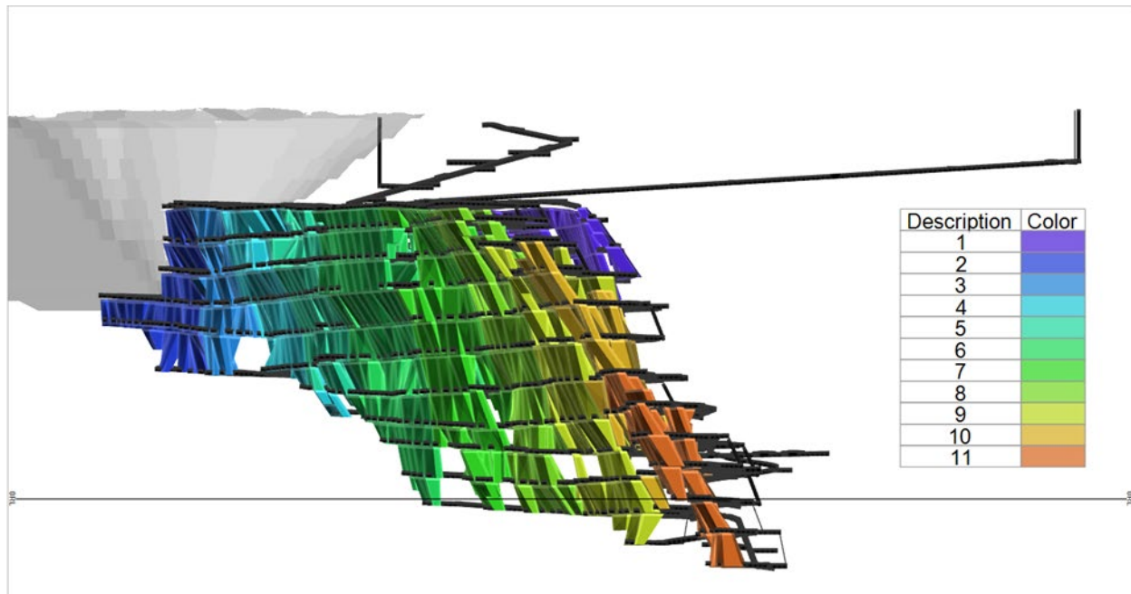
Figure 16.45: Underground Mine Longitudinal View by Mining Blocks - Looking West
