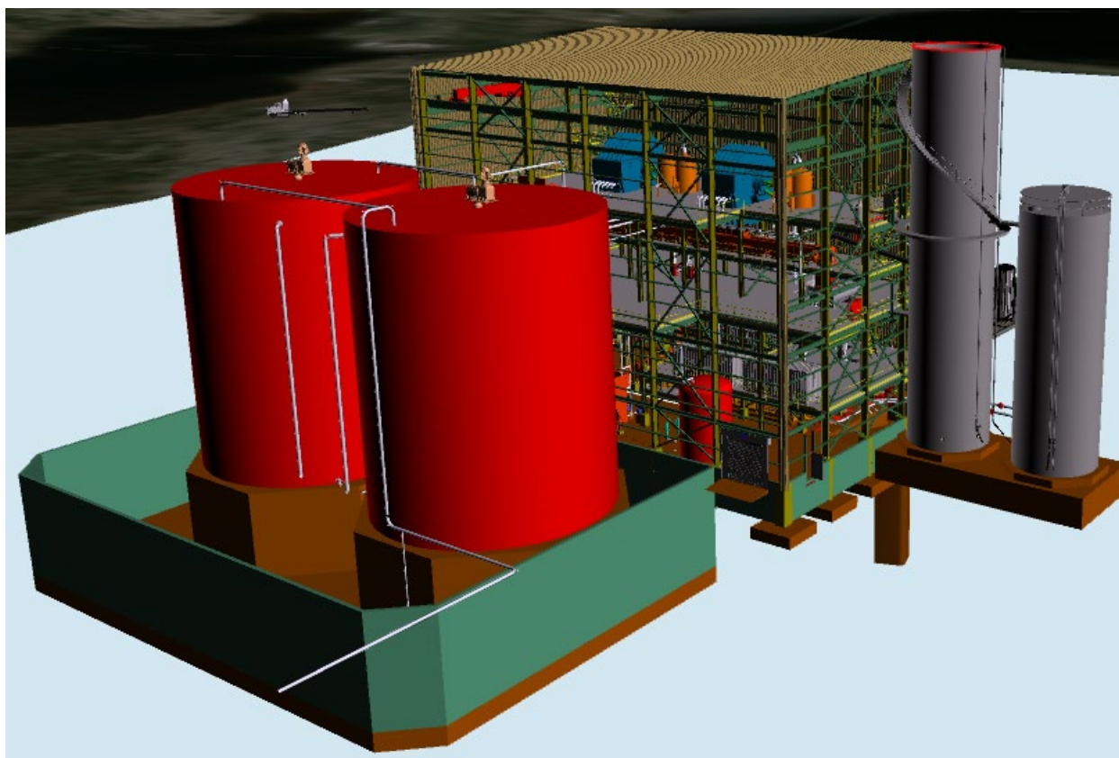
Figure 18.26: Paste Plant Area
