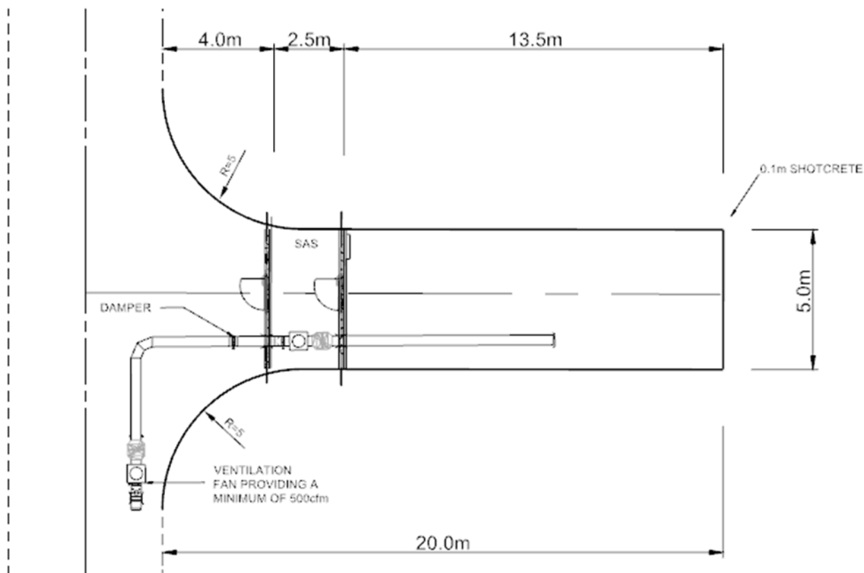
Figure 16.73: Typical Permanent Refuge Station I
