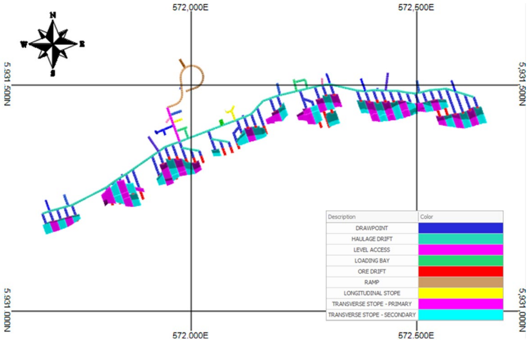
Figure 16.38: Typical Smaller Level - Plan View
