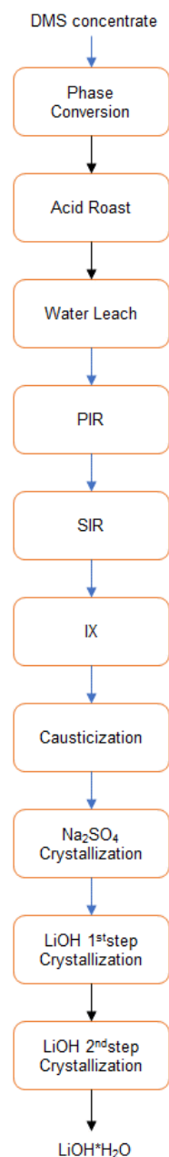
Figure 13.18: Lithium Conversion Testwork Flowsheet
