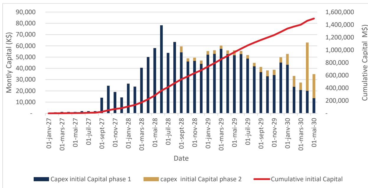
Figure 22.8: Initial CAPEX by Month
