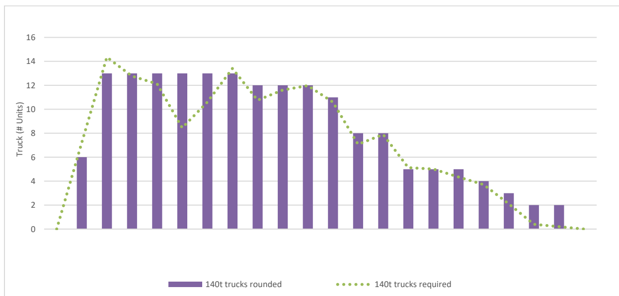
Figure 16.26: Open Pit Truck Requirements
