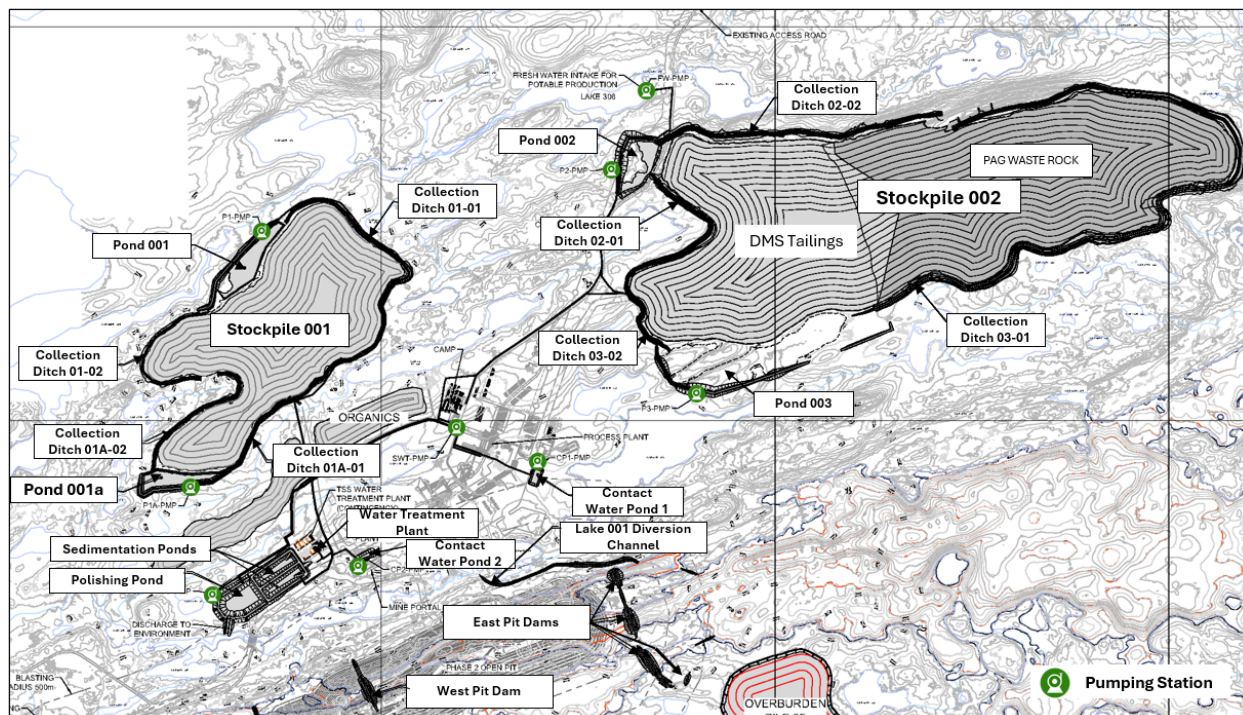
Figure 18.34: Site-Wide Projected Water Management Infrastructures
