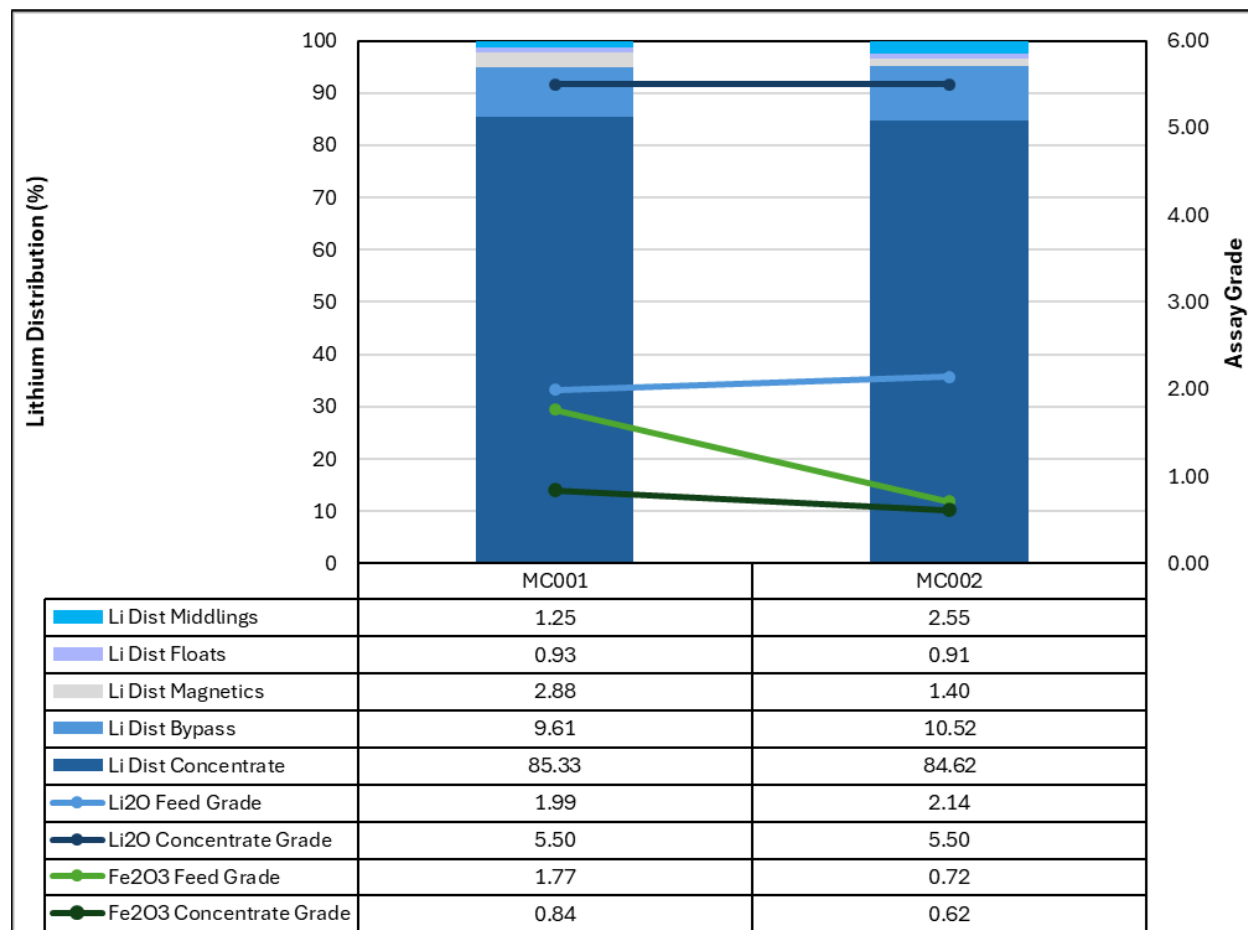
Figure 13.8: HLS Testwork Results
