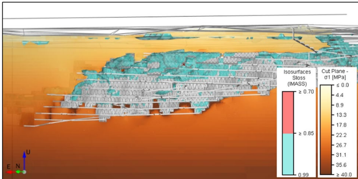
Figure 16.6: Major Principal Stress ( \sigma_1 ) and Damage Indicator (SI loss ) Surrounding the Mined Stopes at Year 2049 From 3D Model
