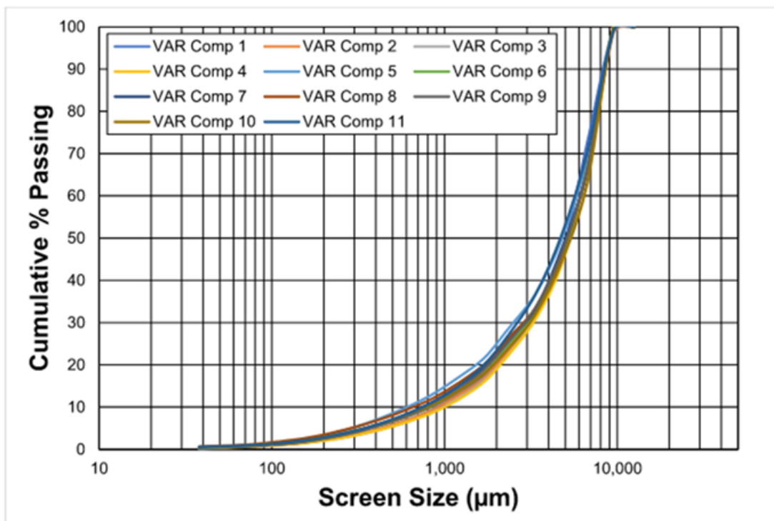
Figure 13.5: Particle Size Distributions for Variability Composite Samples
