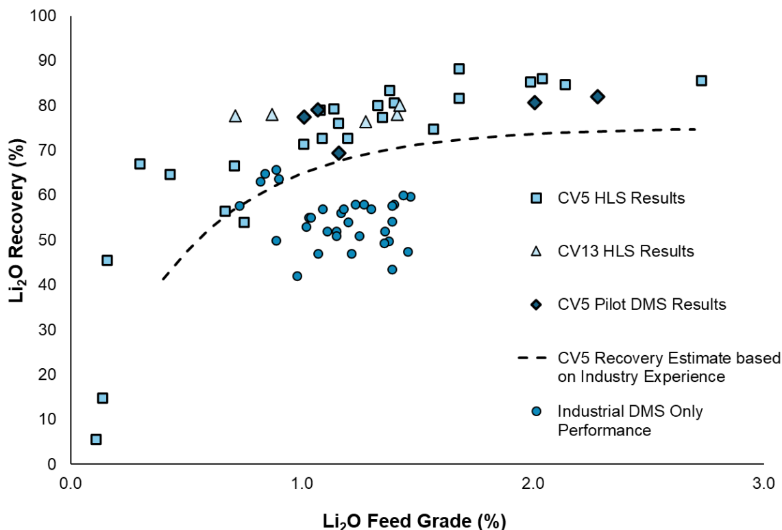
Figure 13.20: Metallurgical Testwork Recovery Results and Industry-based Recovery Estimates for 3x Size Range DMS Process Plant
