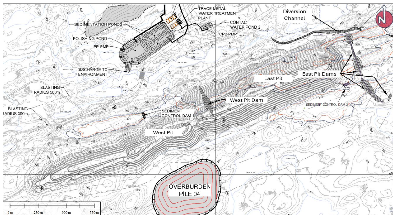
Figure 18.39: Lake 001 Diversion Channel and Cut-off Dams
