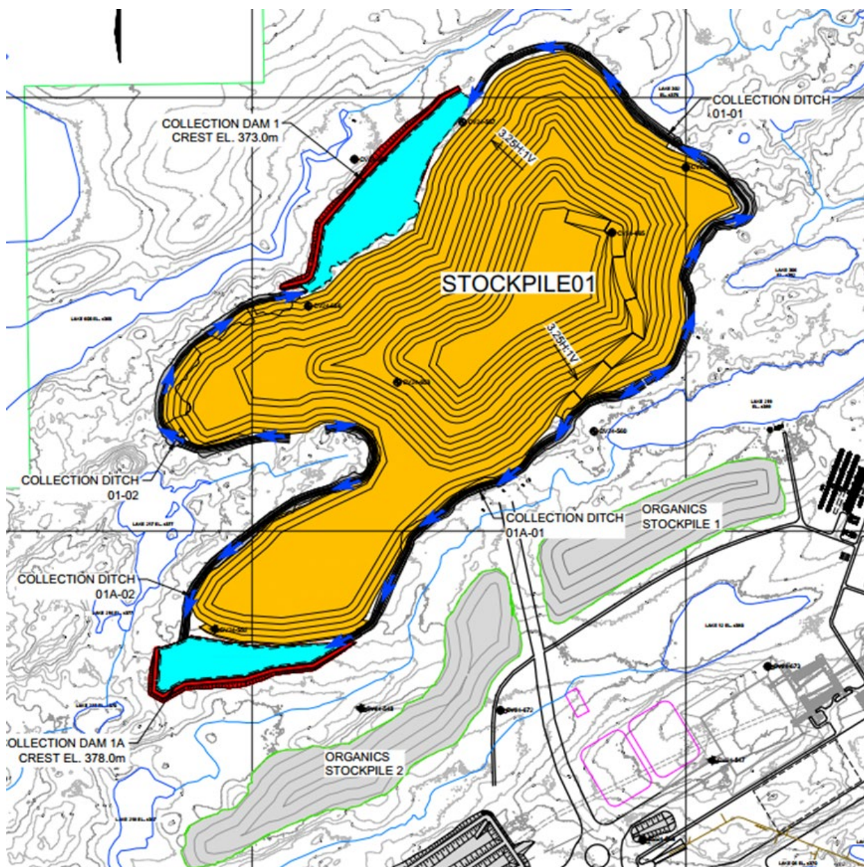
Figure 18.32: Stockpile 01 and Associated Water Management Infrastructure
