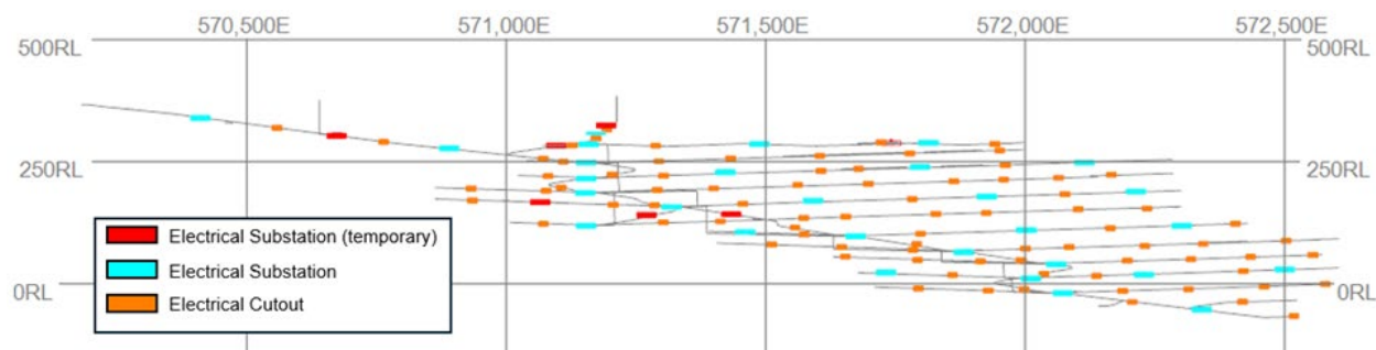
Figure 16.61: Underground Electrical Distribution Network – Looking North
