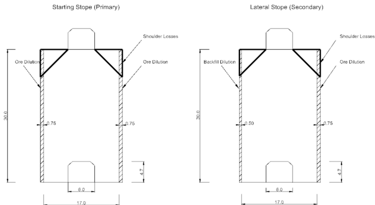
Figure 16.33: Ore Losses During Drilling & Blasting Operations - Section View
