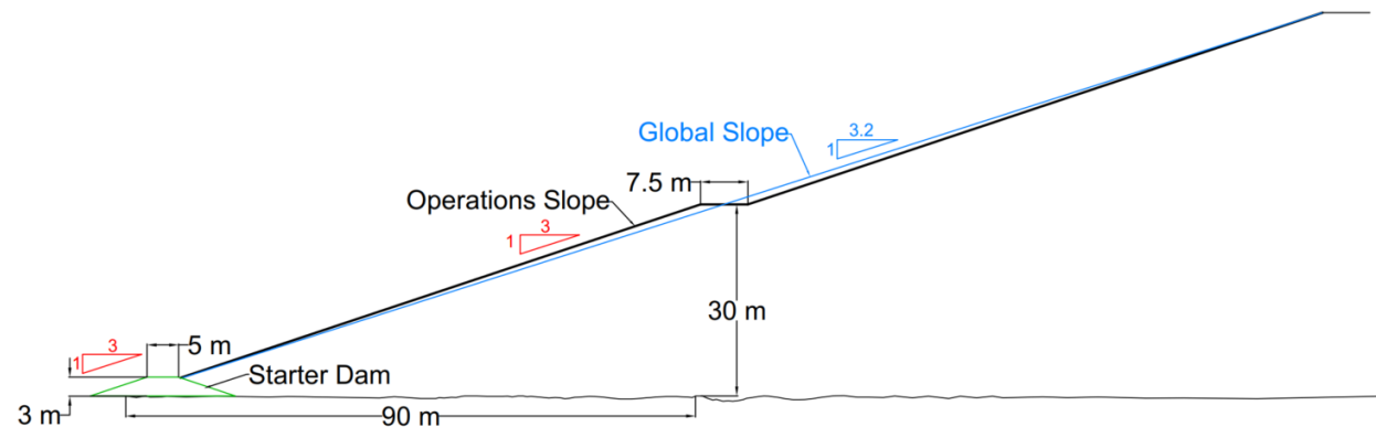
Figure 18.28: Typical Section for Tailings in Stockpile 002 Showing Intermediate Benches for Both Operation and Closure Stages
