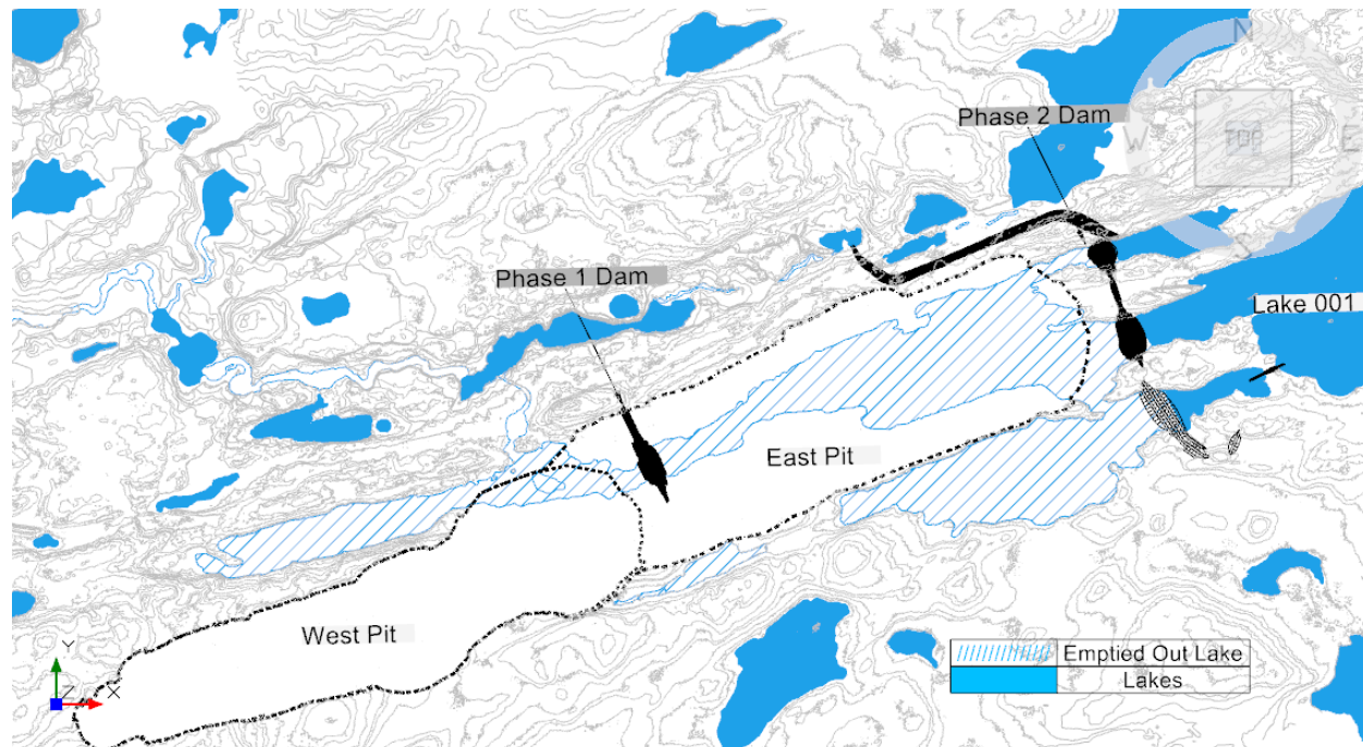
Figure 15.2: West and East Pits Delimitation
