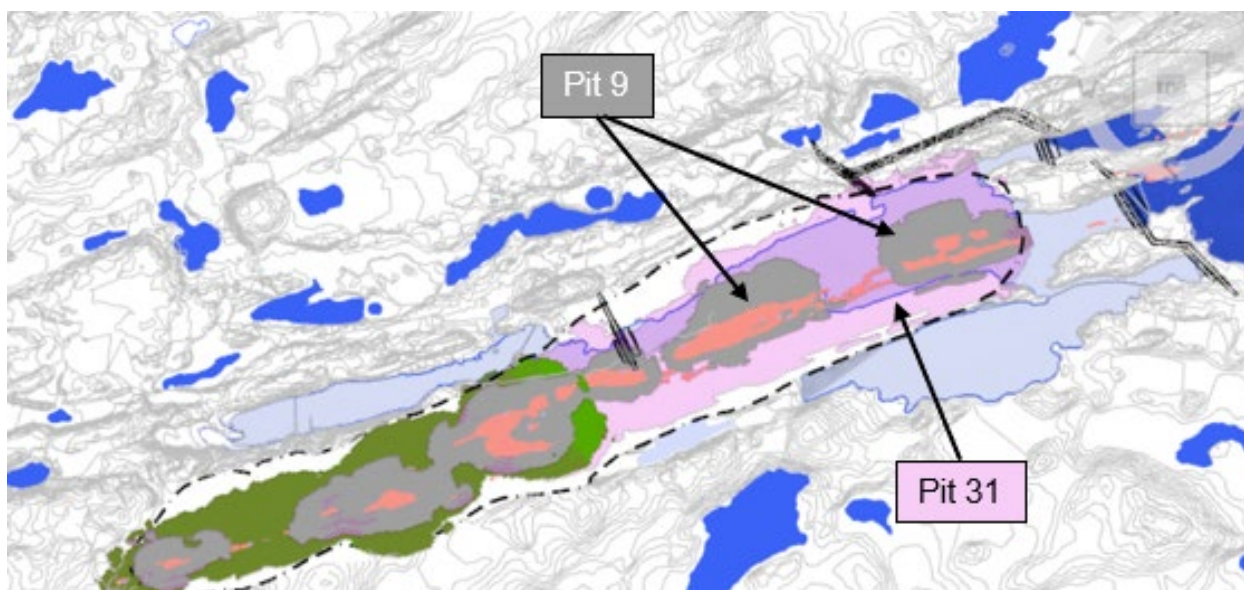
Figure 15.6: East Pit Phasing
