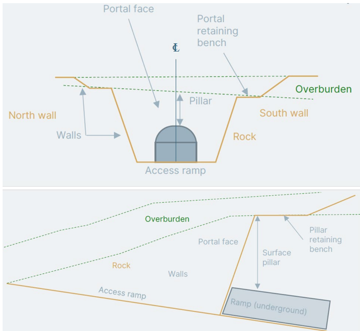
Figure 16.70: Schematic Section View of UG Mine Portal
