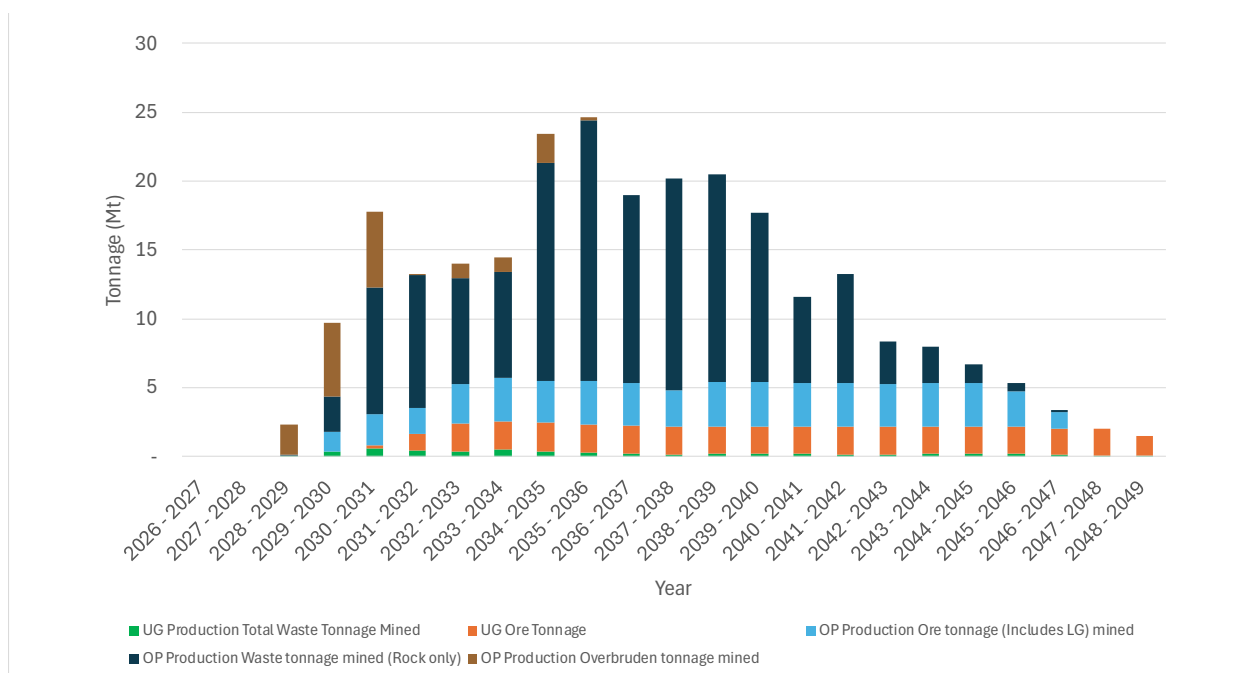
Figure 16.16: Open Pit and Underground Mined Tonnes
