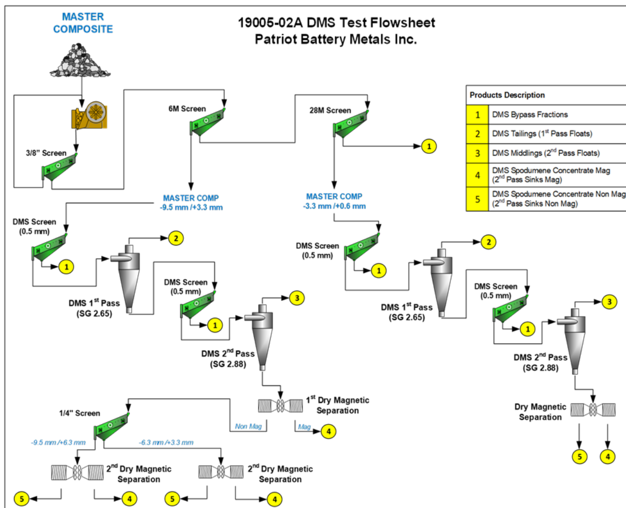
Figure 13.12: DMS Testwork Flowsheet
