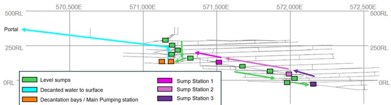
Figure 16.64: Underground Pumping Network – Looking North
