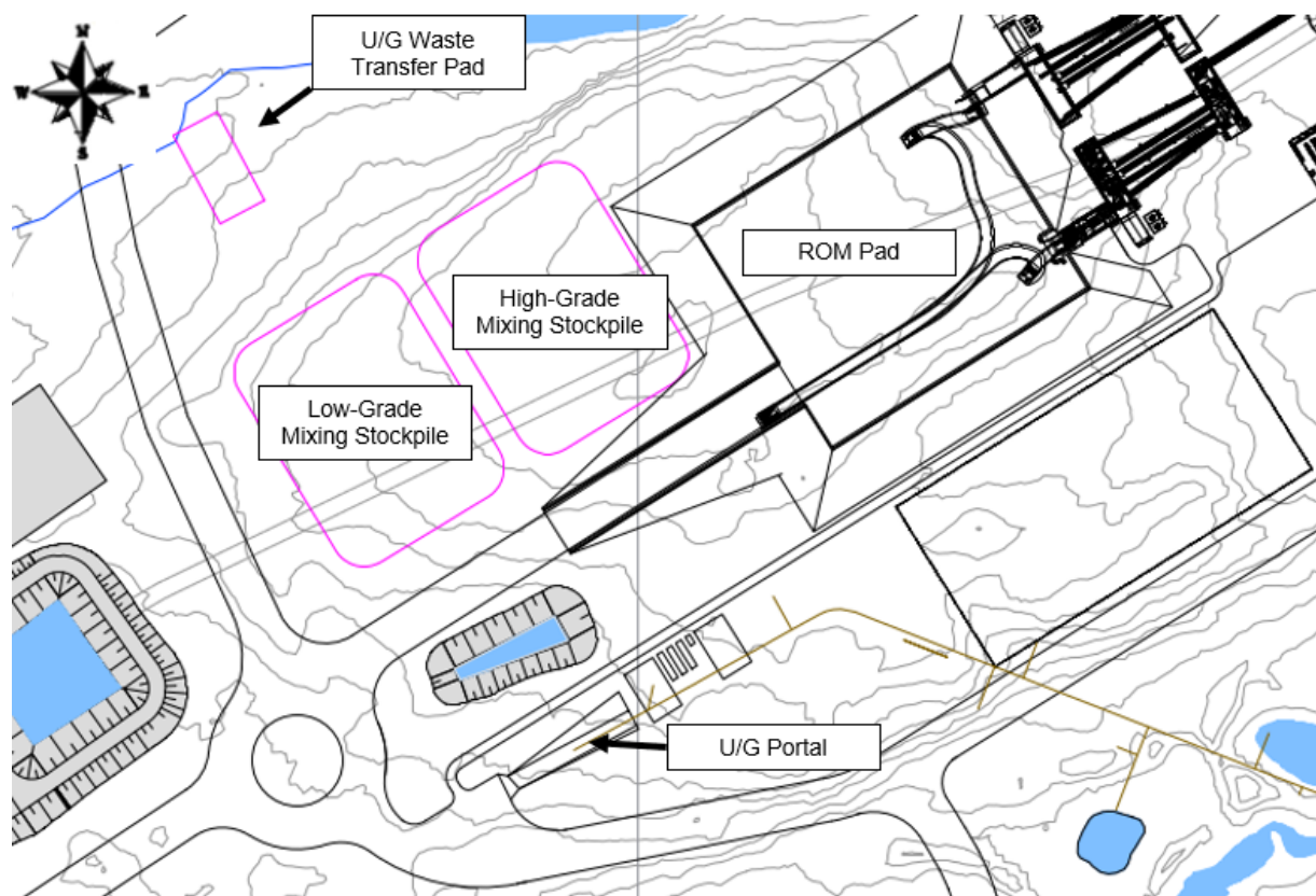
Figure 16.15: Ore Stockpile Location – Plan View
