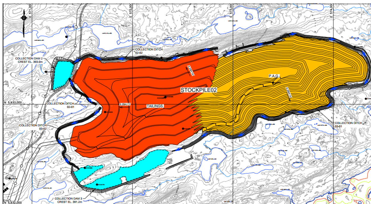
Figure 18.29: Stockpile 002 (Tailings and Waste Rock) and Related Infrastructure
