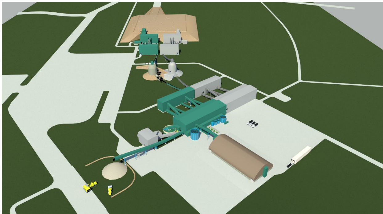
Figure 18.24: Phase 1 (Green) and Phase 2 (Grey) Structures
