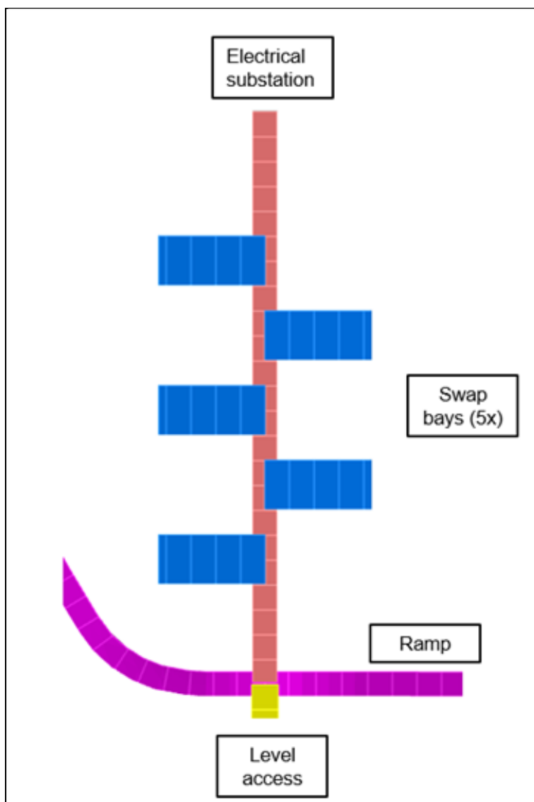
Figure 16.54: Charging Bays Layout
