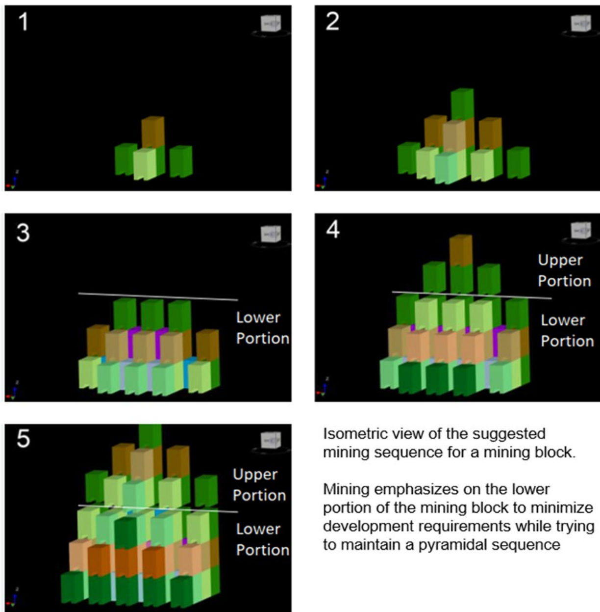
Figure 16.32: Typical Transverse Stoping Sequence
