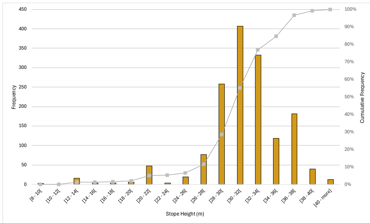
Figure 16.47: Stope Height Histogram
