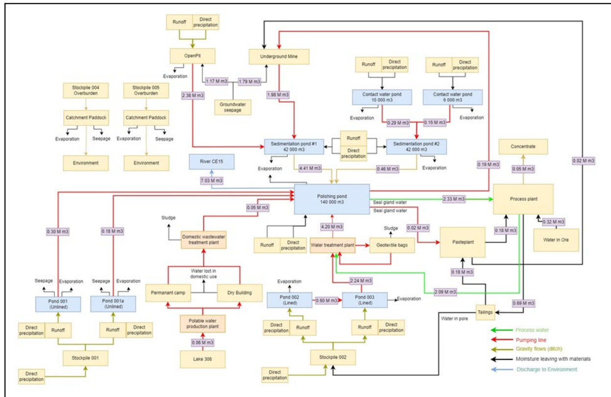
Figure 18.38: Site Water Management Flow Diagram (including annual flow rates during average climate condition)
