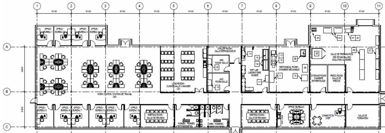
Figure 18.20: Mill Office Plan View
