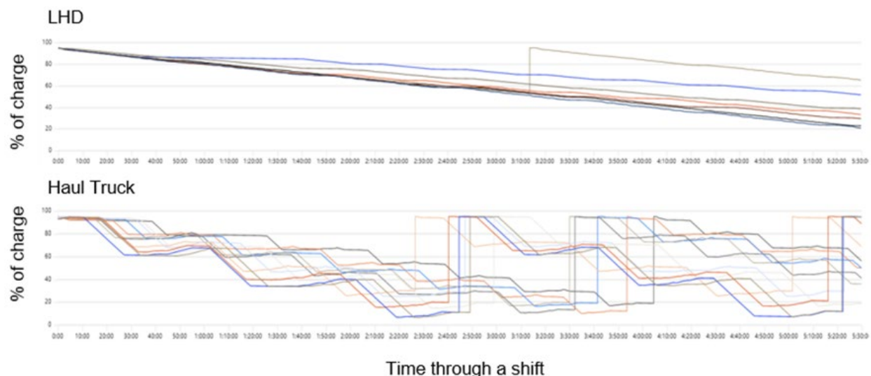
Figure 16.55: BEVs Haul Trucks and LHDs Modelled Battery Charging Cycles Through Shift
