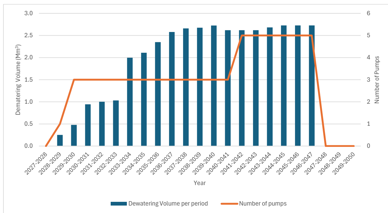
Figure 16.27: Open Pit Dewatering Volumes and Quantity of Pumps Over Time
