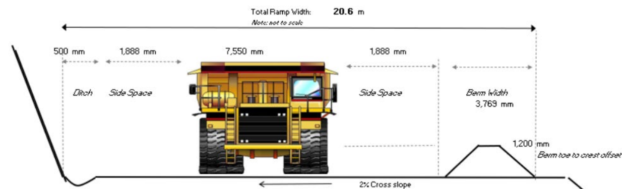
Figure 15.8: Single-Lane Ramp Design Criteria
