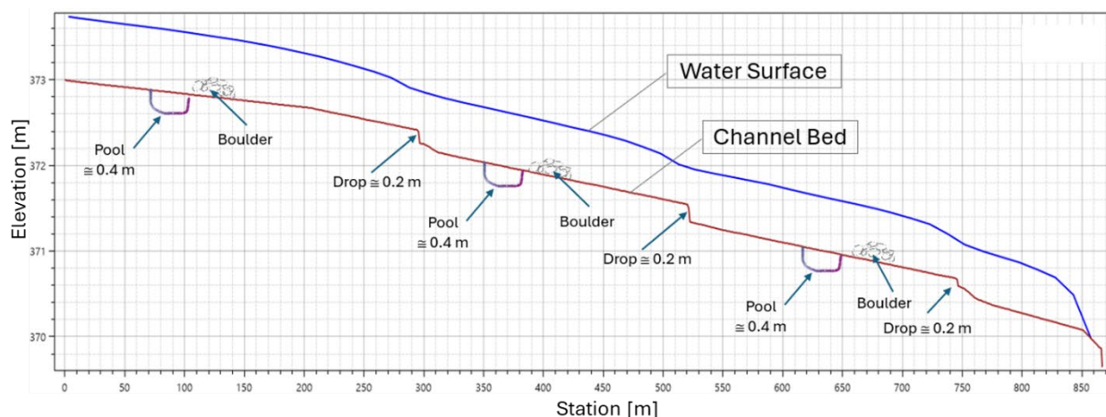
Figure 18.40: Profile of Diversion Channel with Proposed Fish Habitat / Passage
