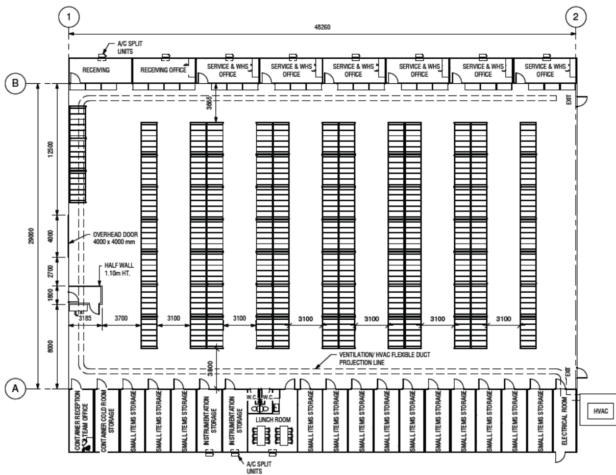
Figure 18.17: Warehouse Plan View
