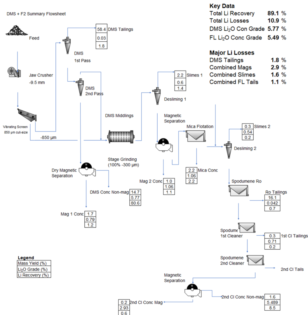
Figure 13.14: Combined DMS and Flotation Testwork Flowsheet
