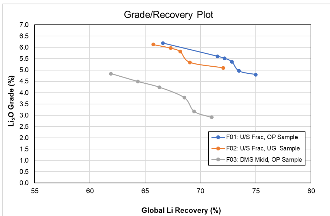
Figure 13.15: 19005-10 Spodumene Flotation Testwork Results
