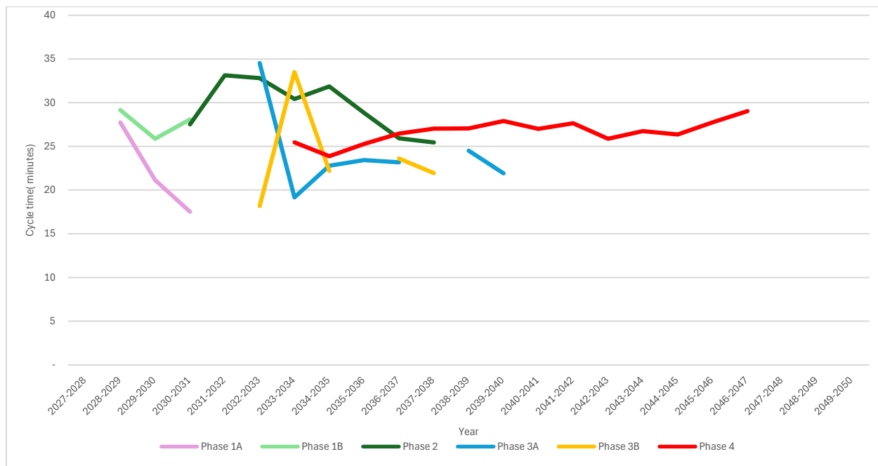
Figure 16.25: Open Pit Average Haulage Cycle Times by Phase
