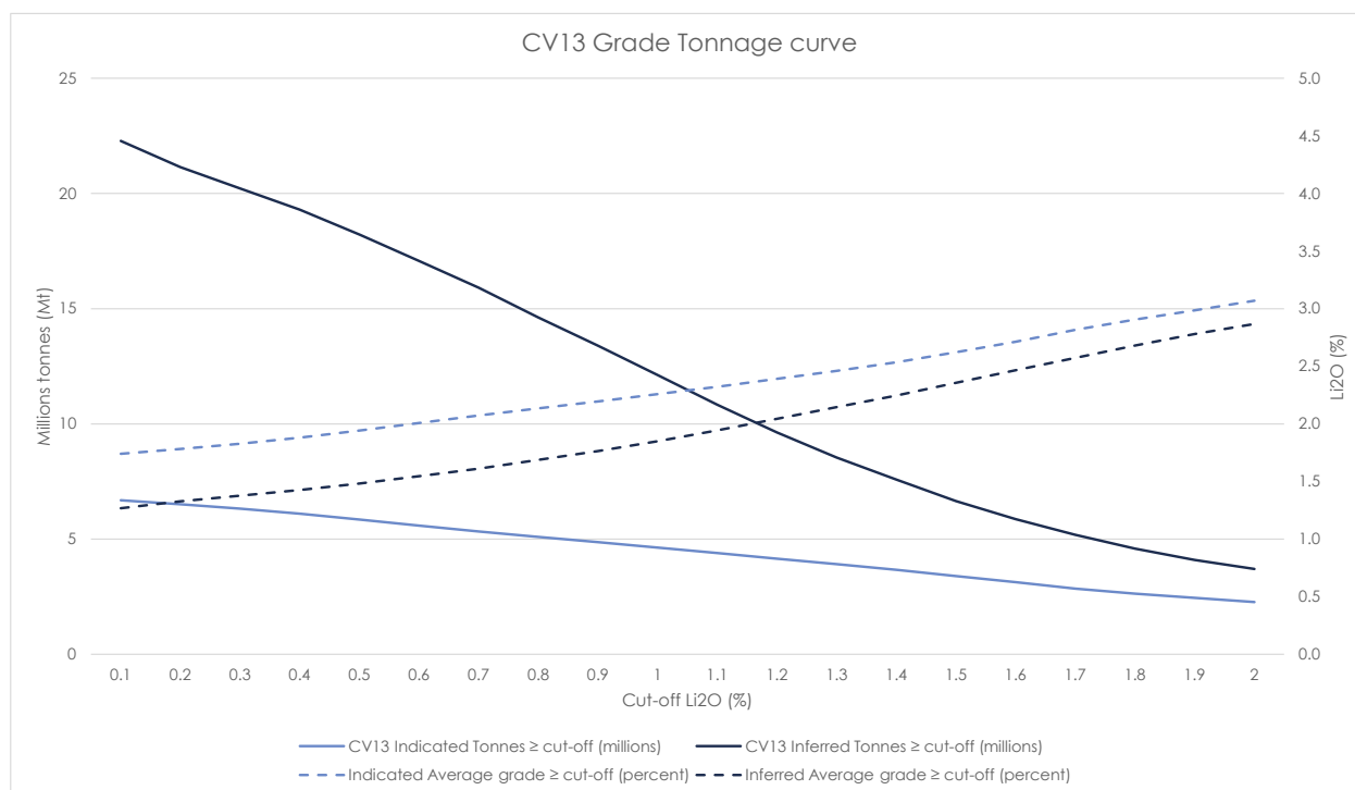
Figure 14.21: Shaakichiuwaanaan Mineral Resource Grade-Tonnage Curves for CV13
