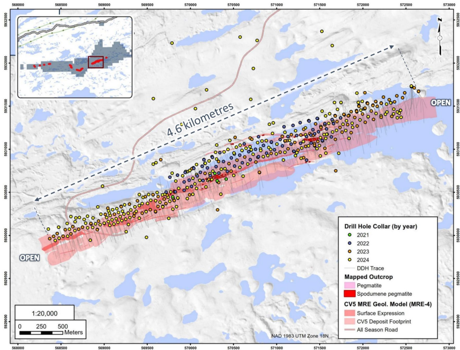
Figure 10.2: Drill Holes and Channels Completed at CV5 LCT Pegmatite Through 2024
