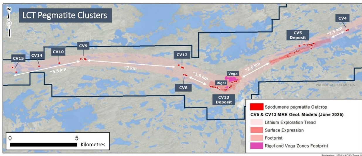
Figure 7.5: LCT Pegmatite Clusters at the Property
