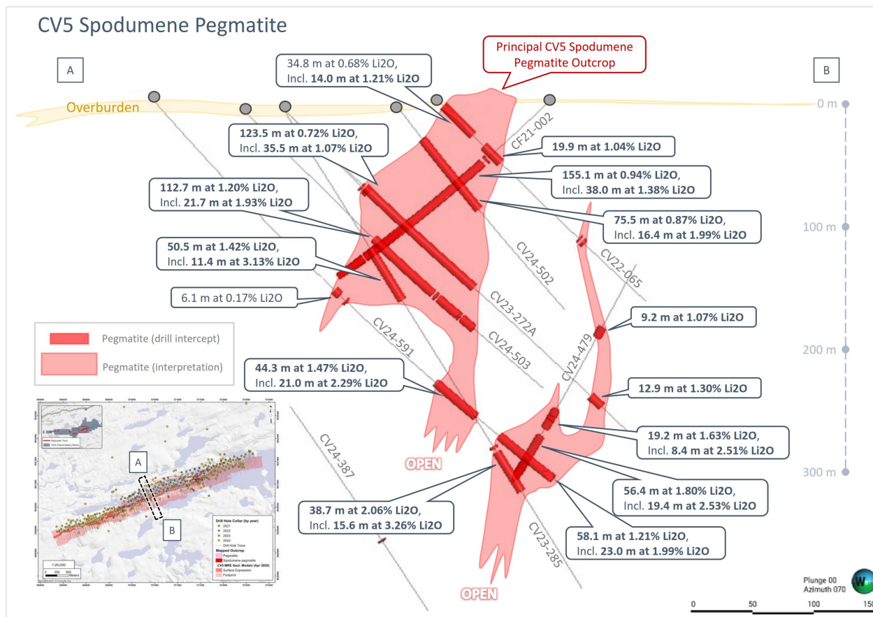
Figure 7.16: Simplified Cross-Section of CV5 Pegmatite Geological Model
