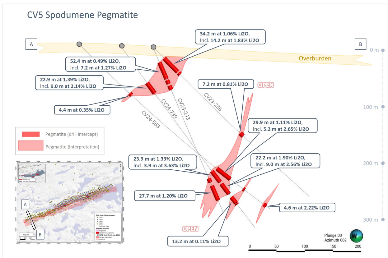
Figure 7.17: Simplified Cross-Section of CV5 Pegmatite Geological Model
