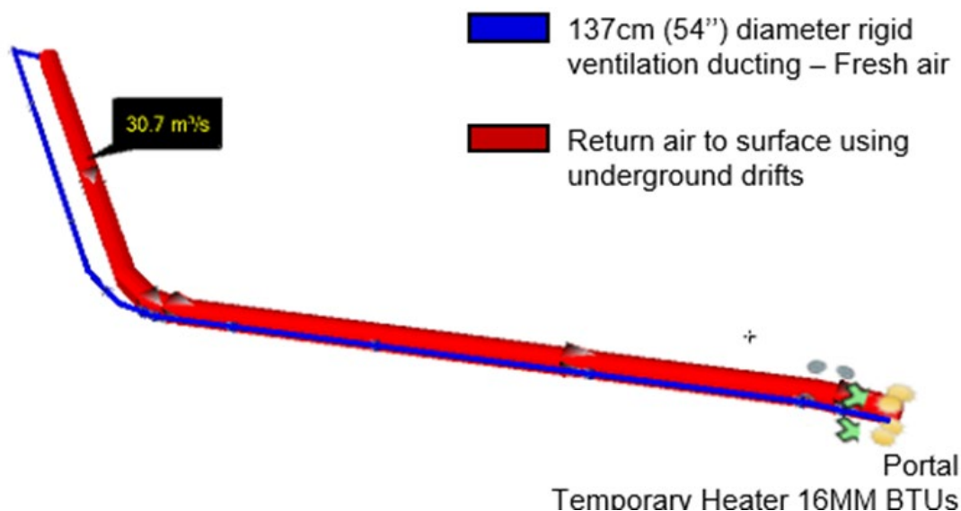
Figure 16.56: Underground Mine Ventilation Network – Stage 1 – Temporary Ventilation Set-up – Isometric View from North-West
