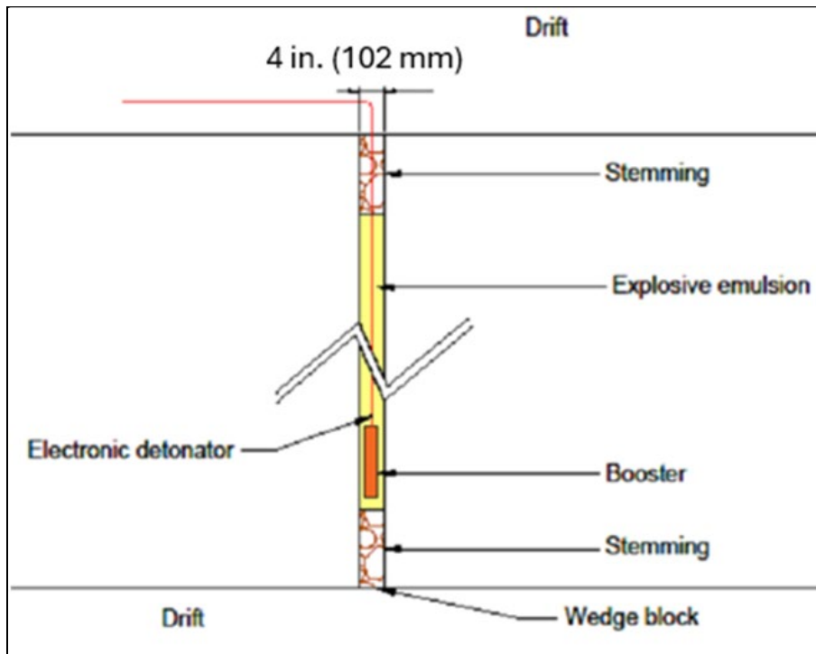
Figure 16.51: Typical Production Hole Loading Specifications
