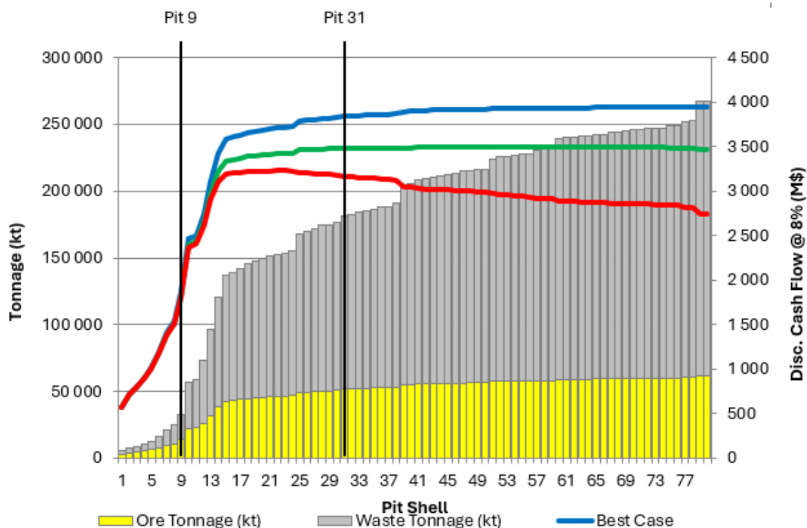
Figure 15.5: M&I Pit by Pit Results @ USD 1,303/t Conc.
