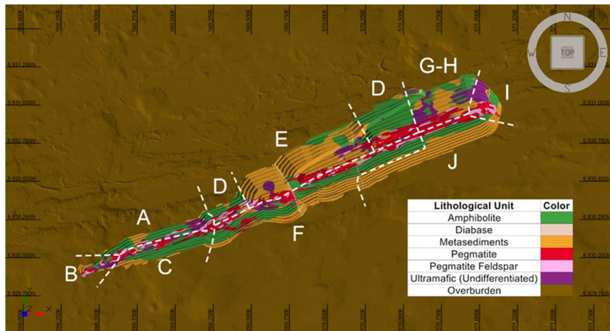
Figure 16.3: Open Pit Design Sectors
