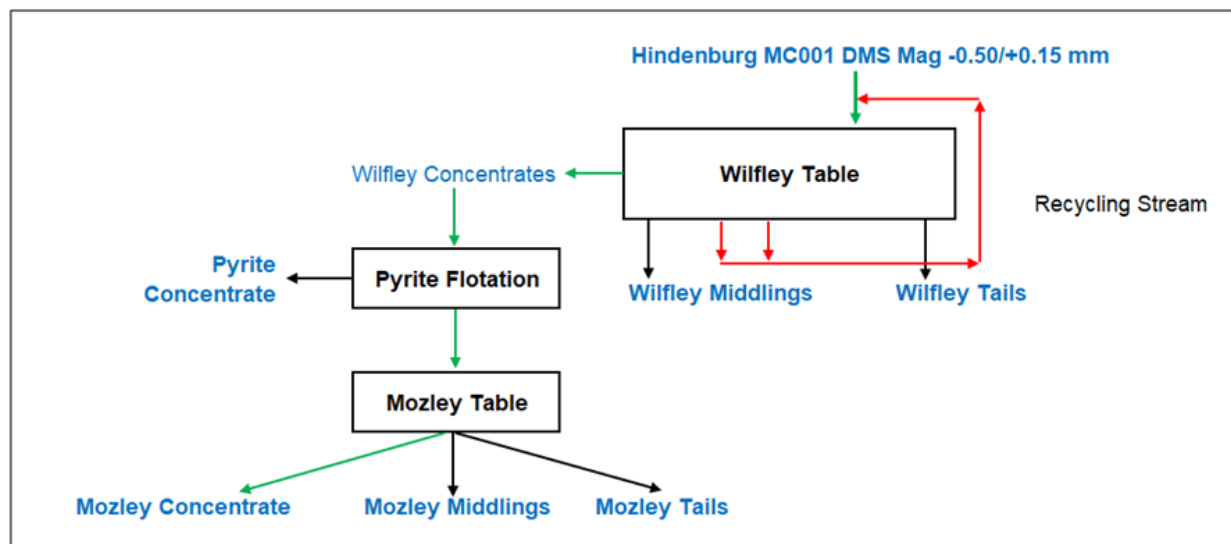
Figure 13.17: SGS Gravity Separation Flowsheet
