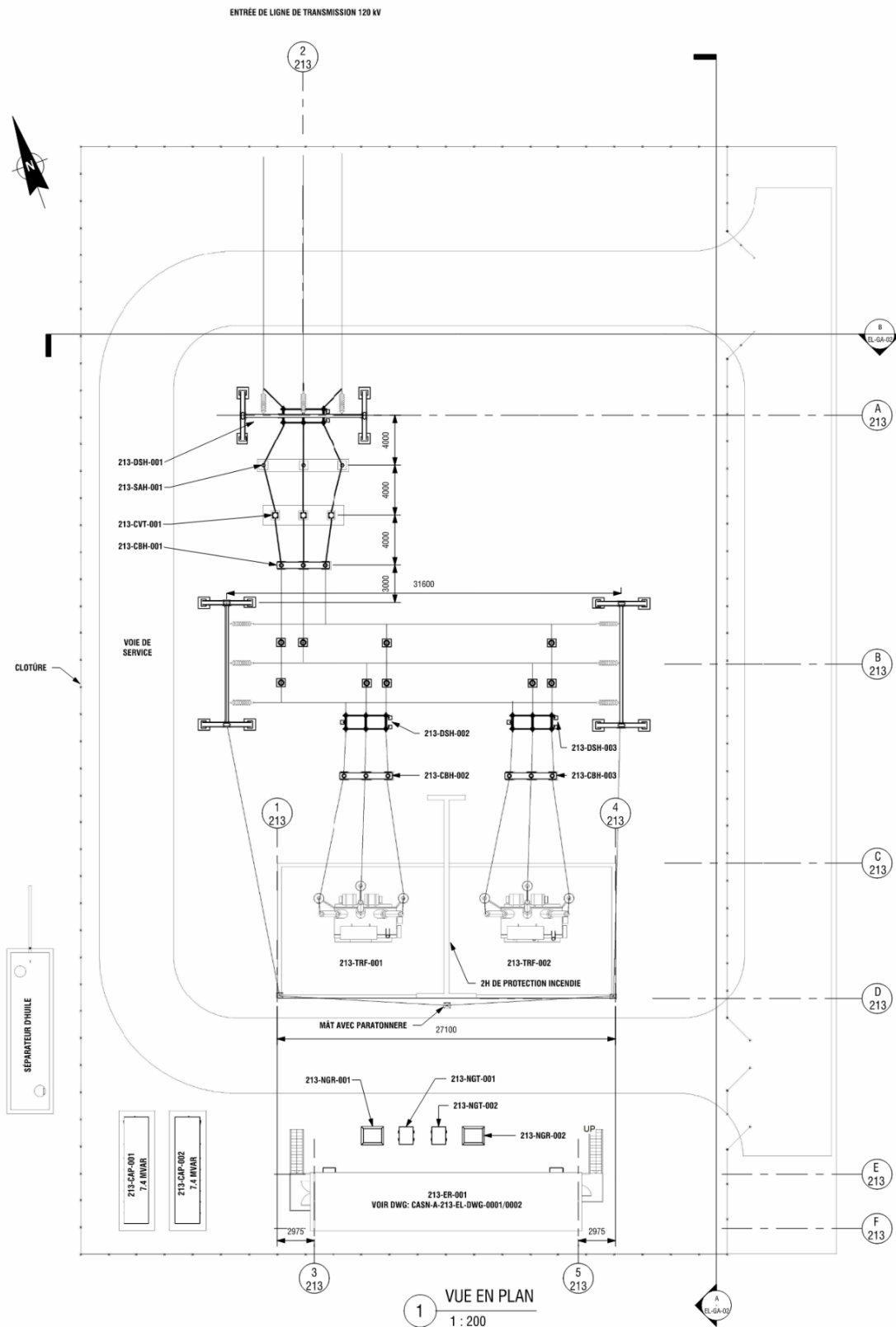
Figure 18.46: Site Main Substation
