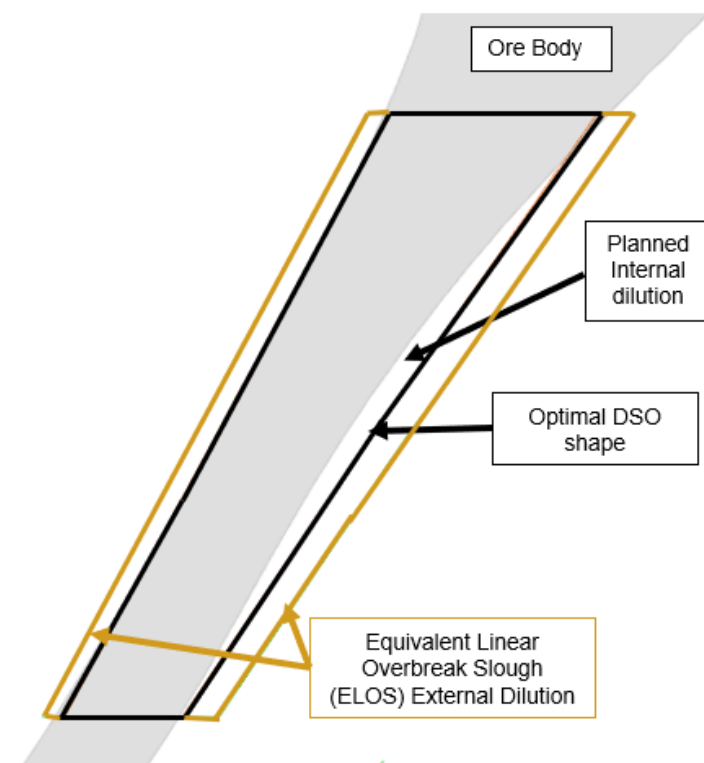
Figure 15.9: Equivalent Linear Overbreak Slough (ELOS) Schematic
