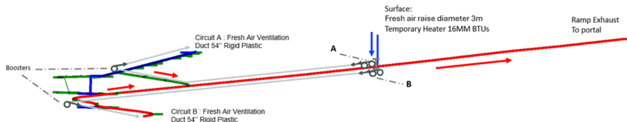
Figure 16.57: Underground Mine Ventilation Network – Stage 2 – Temporary Ventilation Set-up – Isometric View from North-West
