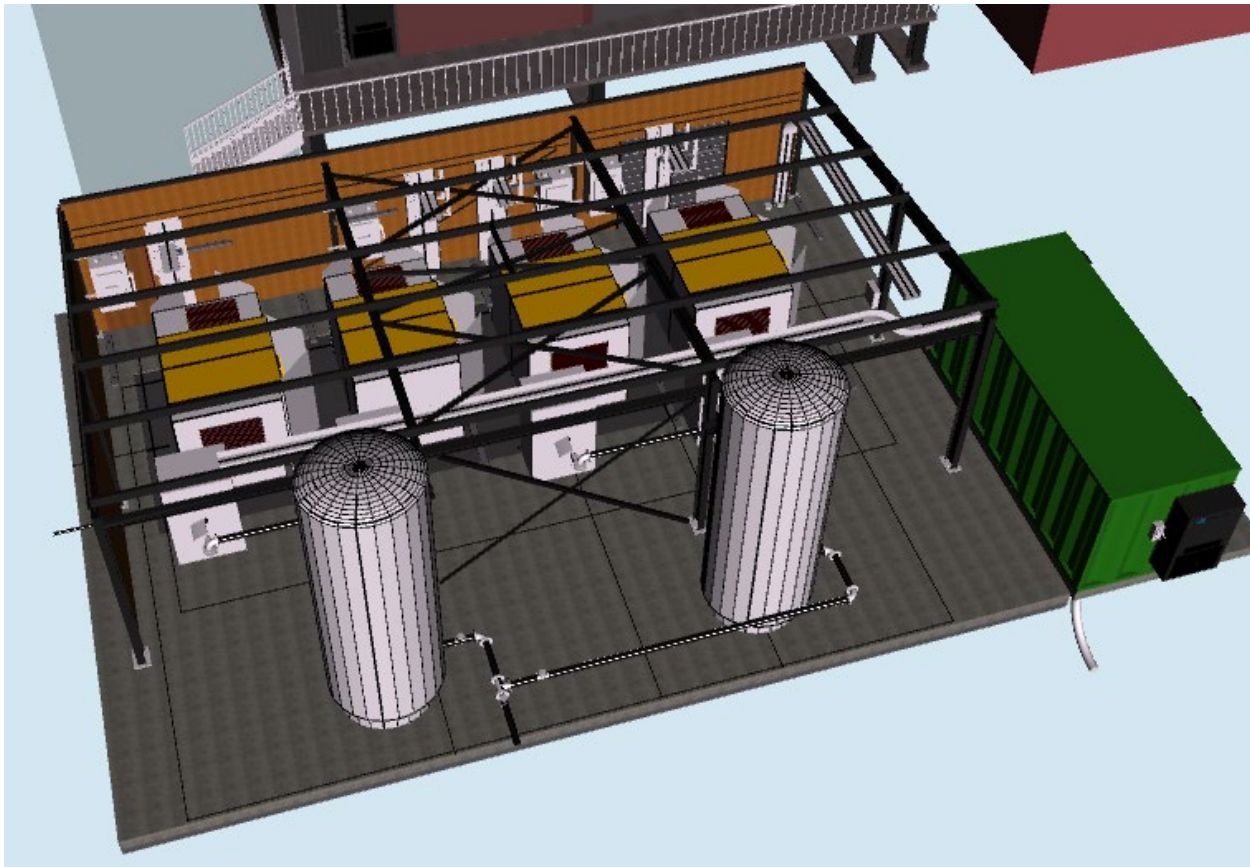
Figure 18.12: Compressor Building
