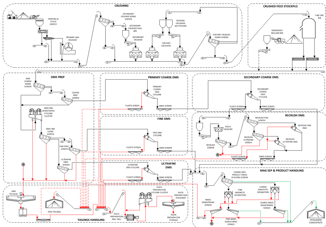
Figure 17.3: Mineral Processing Facility Simplified Process Flow Diagram
