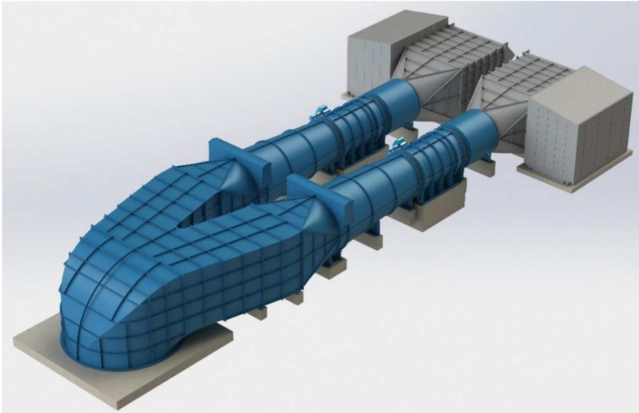
Figure 18.11: Underground Mine Main Ventilation Set-up
