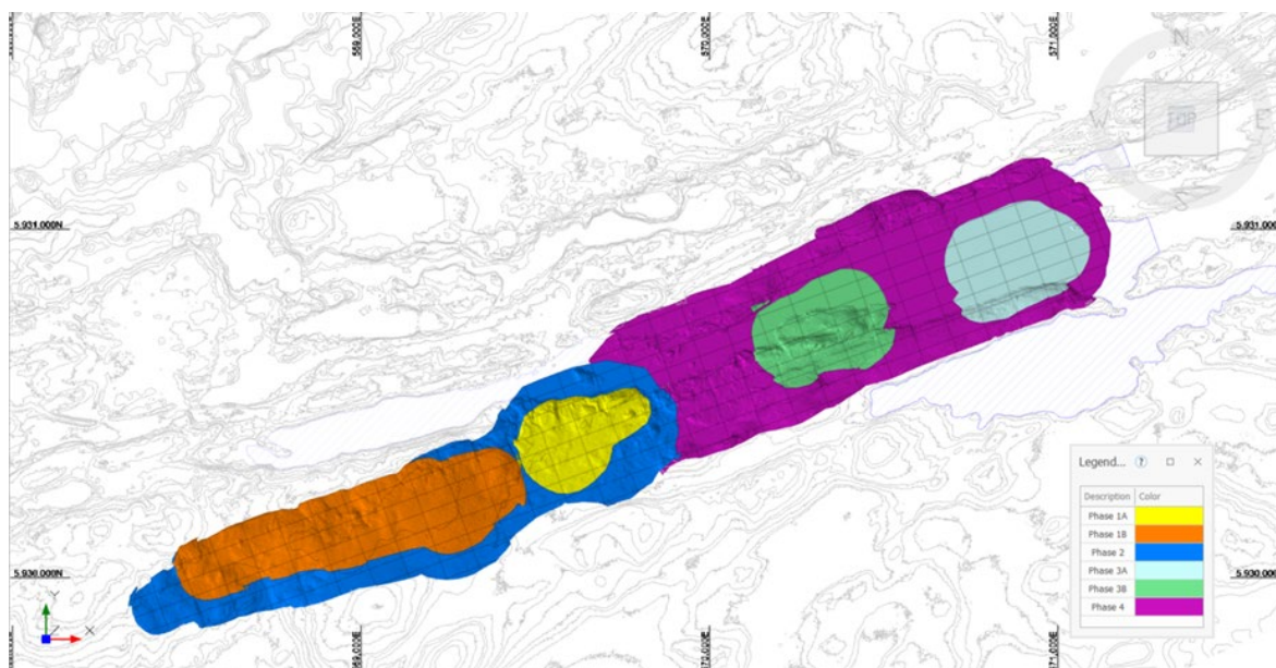
Figure 16.7: Open Pit Phase Limits - Plan View
