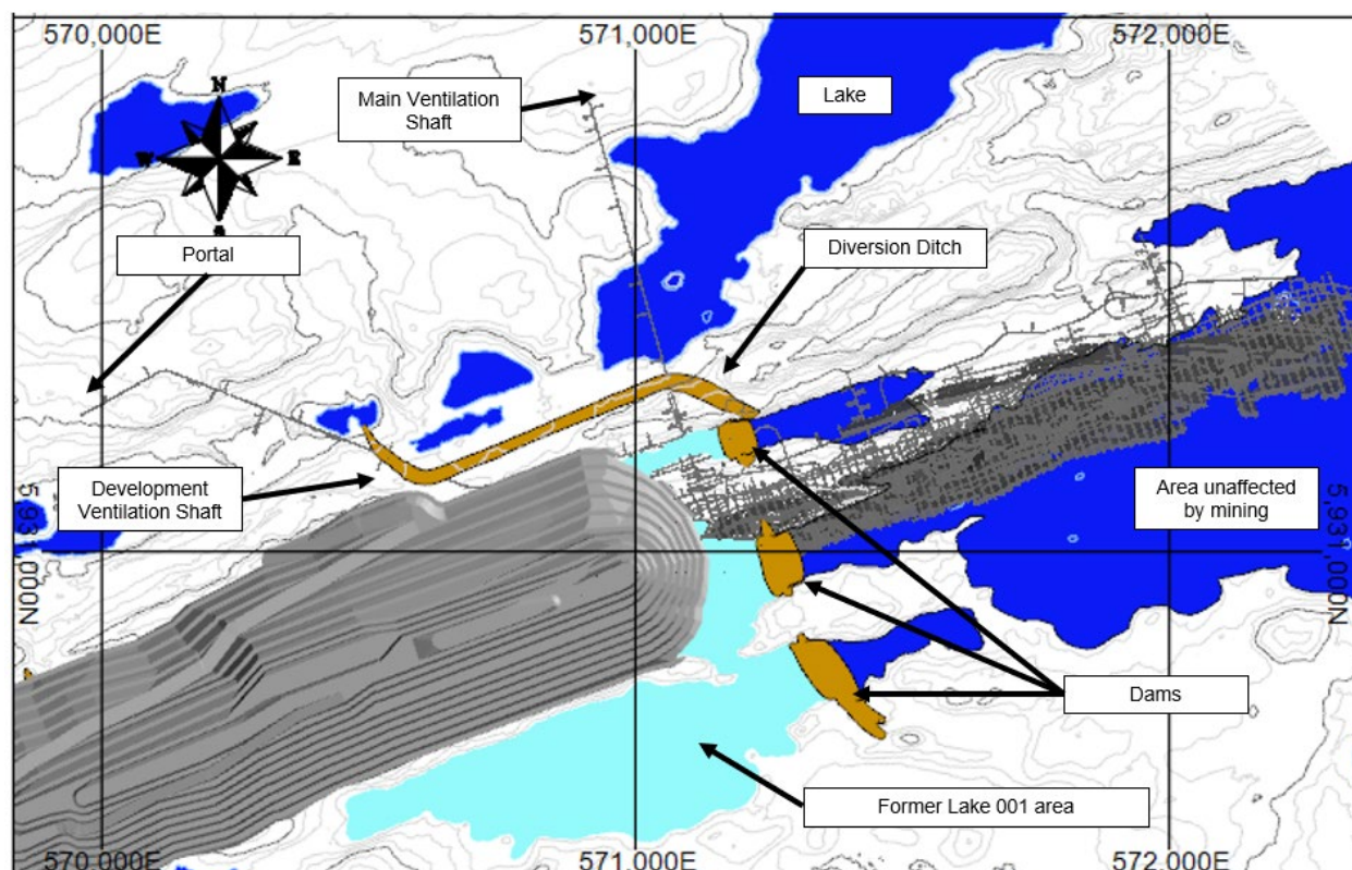
Figure 1.5: Underground Mine and Surfaces Constraints – Plan View
