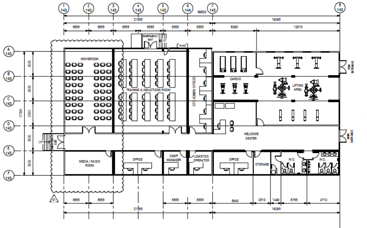
Figure 18.6: Camp Office and Welcome Centre, Plan View
