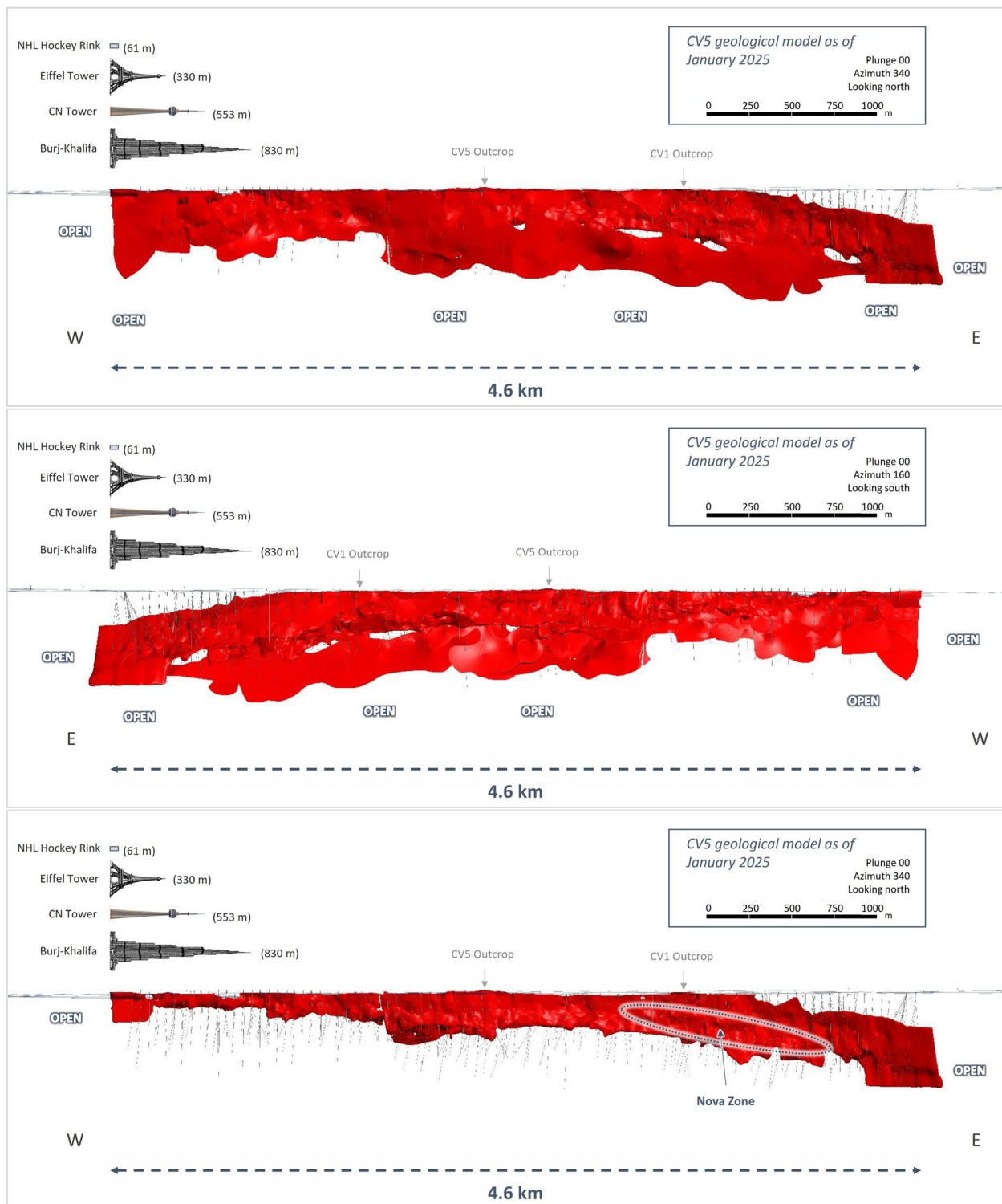
Figure 7.14: Side View of CV5 Geological Model
