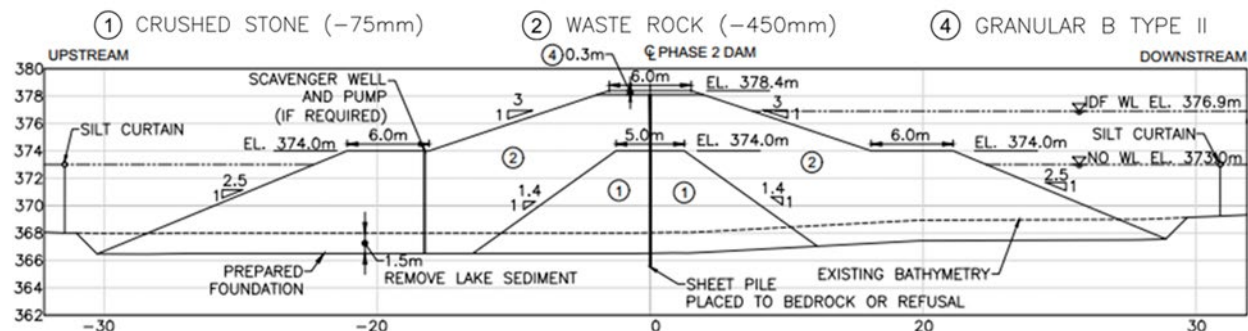
Figure 18.41: Typical Cross-Section for Cut-Off Dam (critical section)
