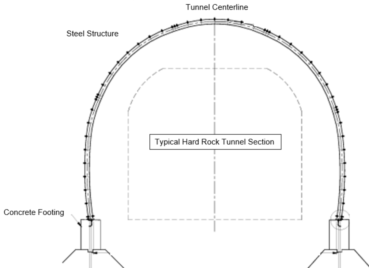
Figure 18.10: Typical Deep-Corrugated Galvanized Steel Plates Portal
