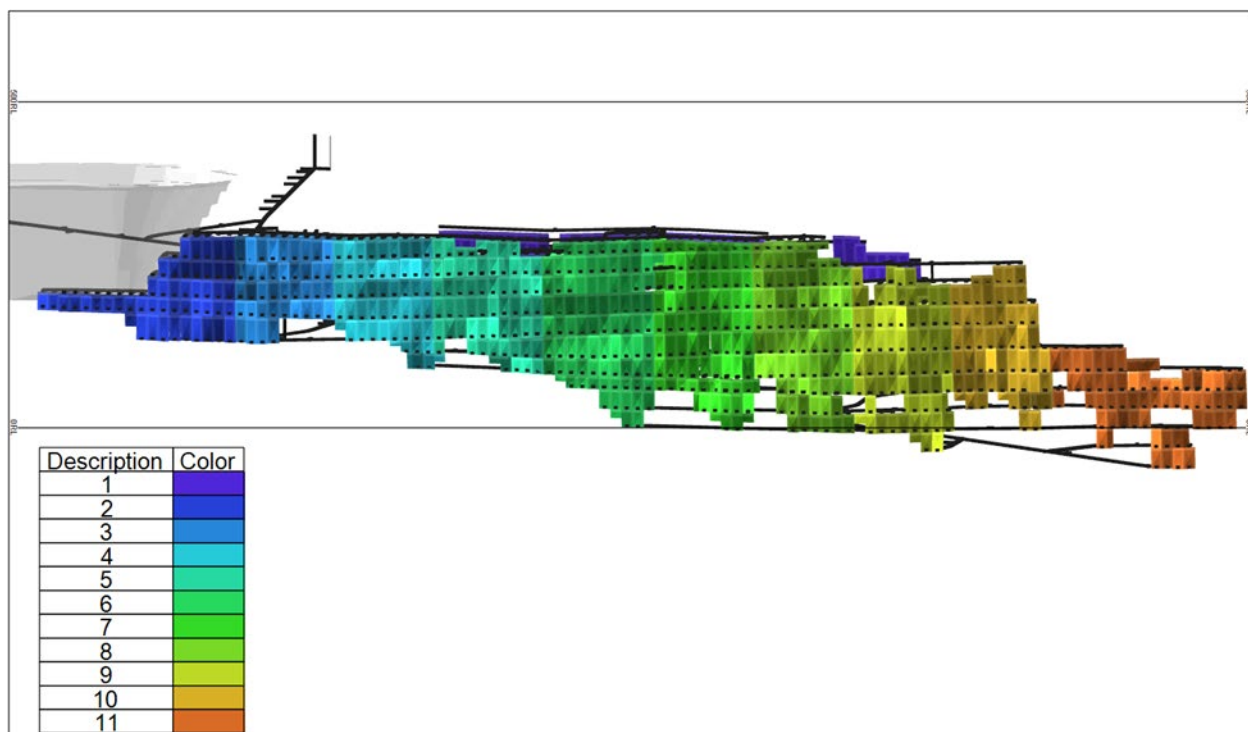
Figure 16.46: Underground Mine Longitudinal View by Mining Blocks - Looking North
