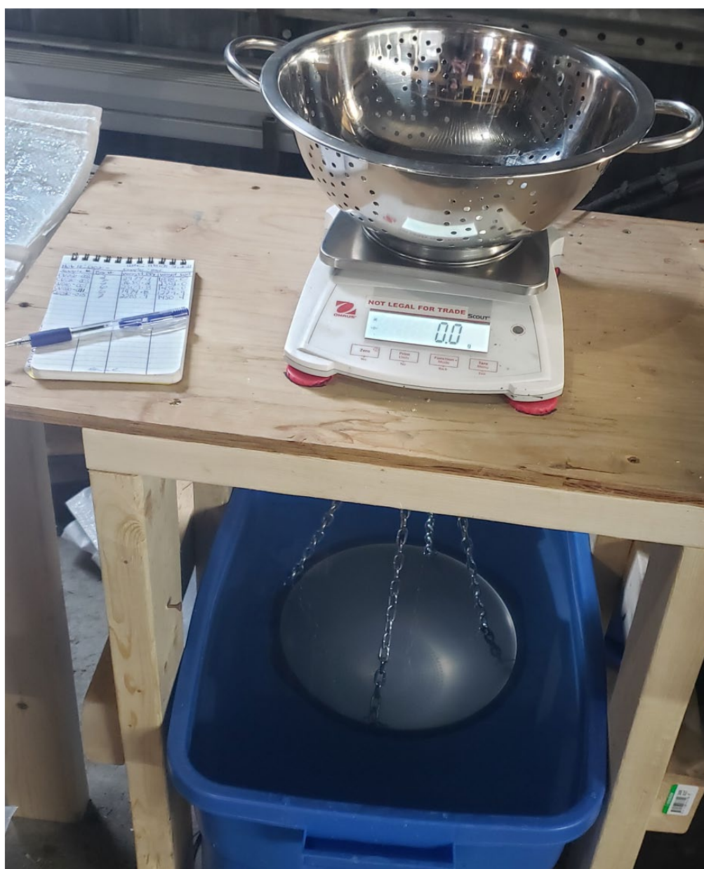
Figure 14.1: SG Measurement Setup Employed by PMET Resources
