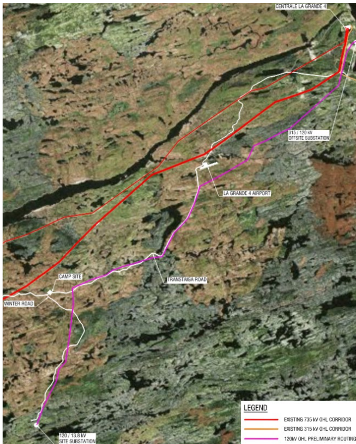
Figure 18.45: Transmission Route
