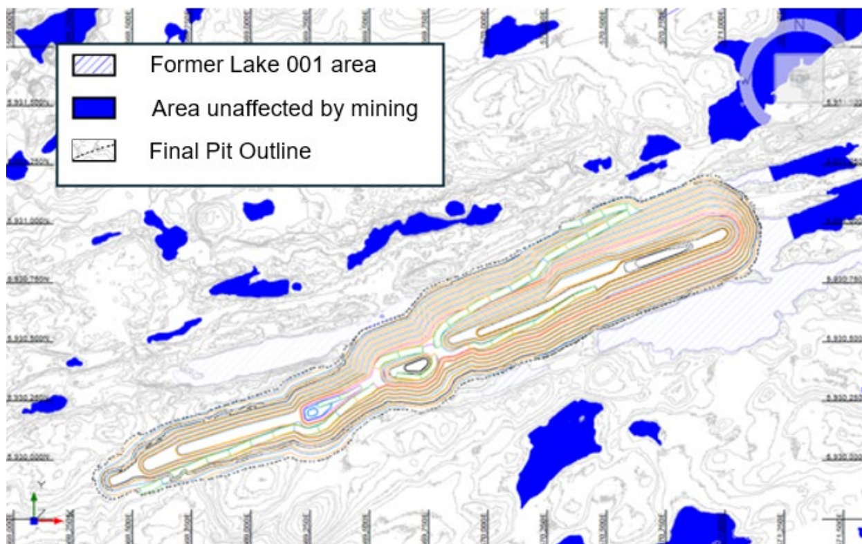
Figure 16.13: Phase 4 (Final Open Pit Design) – Plan View
