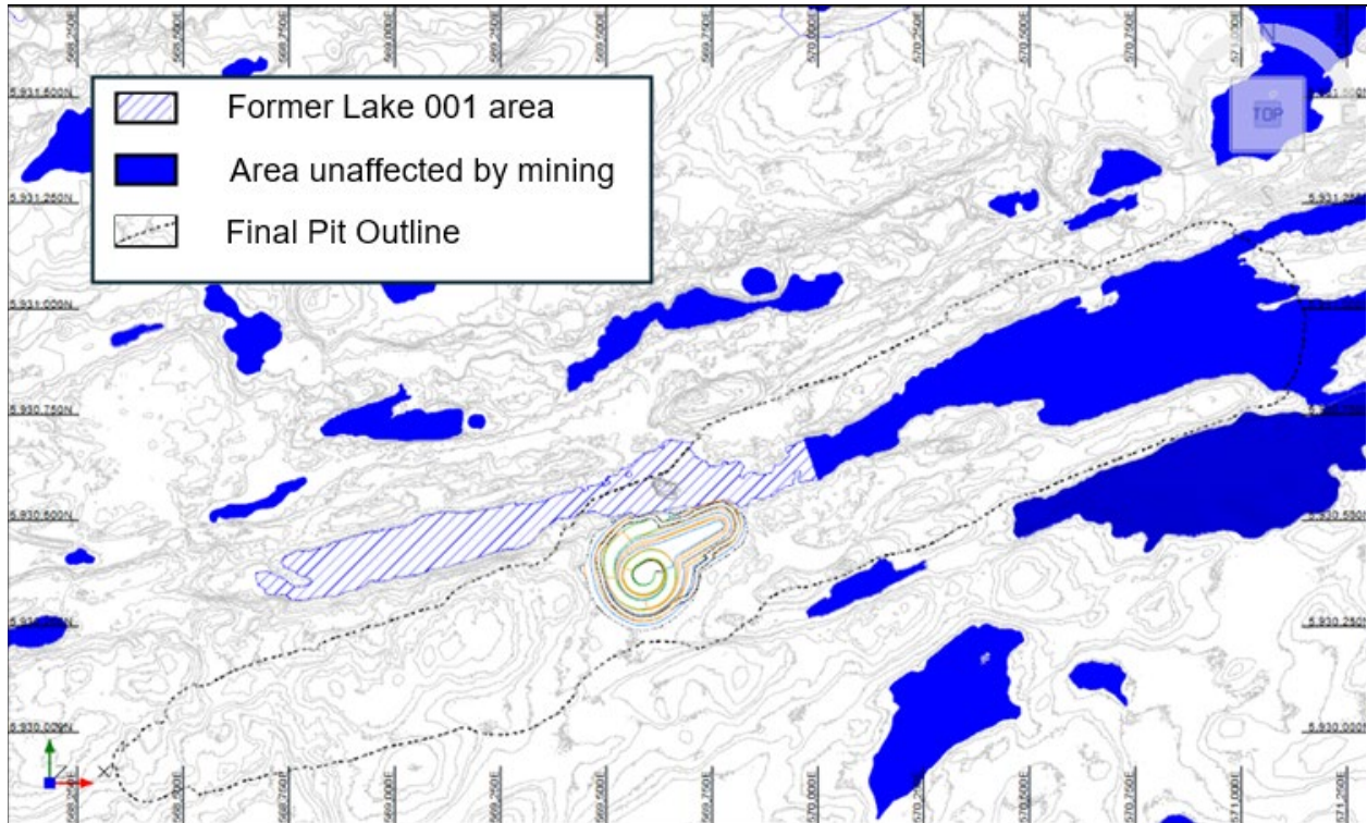
Figure 16.8: Phase 1A Open Pit Design – Plan View
