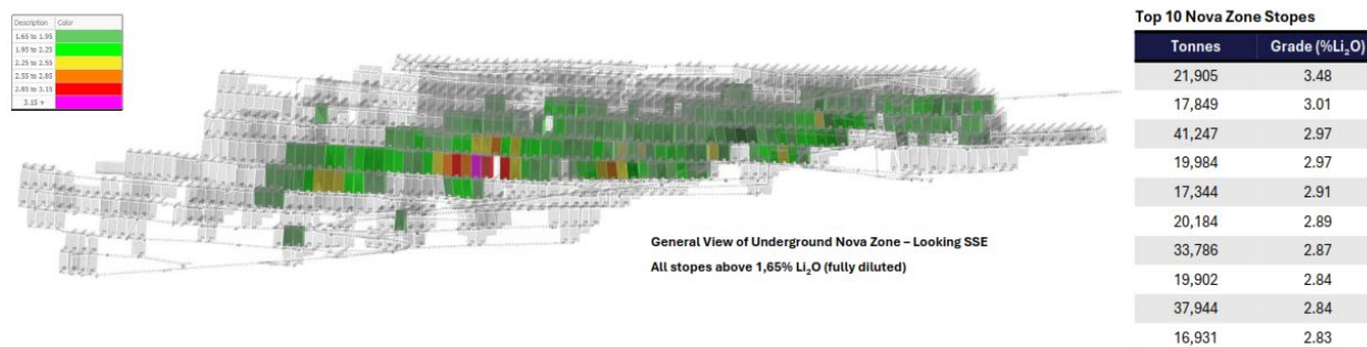
Figure 24.2: General View of Underground Nova Zone – Looking SSE
