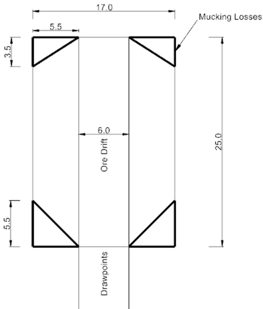
Figure 16.34: Ore Losses During Mucking Operations - Plan View
