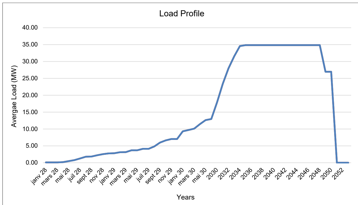
Figure 18.48: Load Profile
