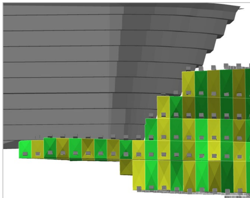
Figure 16.49: Open Pit and Underground Mine Interaction Close-Up – Looking North
