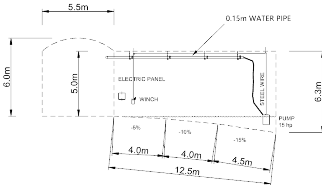
Figure 16.62: Typical Sump Located in Level Access
