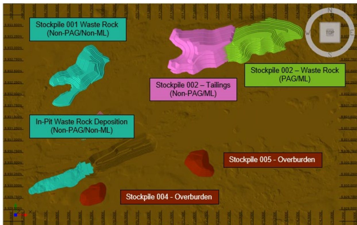
Figure 16.14: Waste Storage Facility – Plan View
