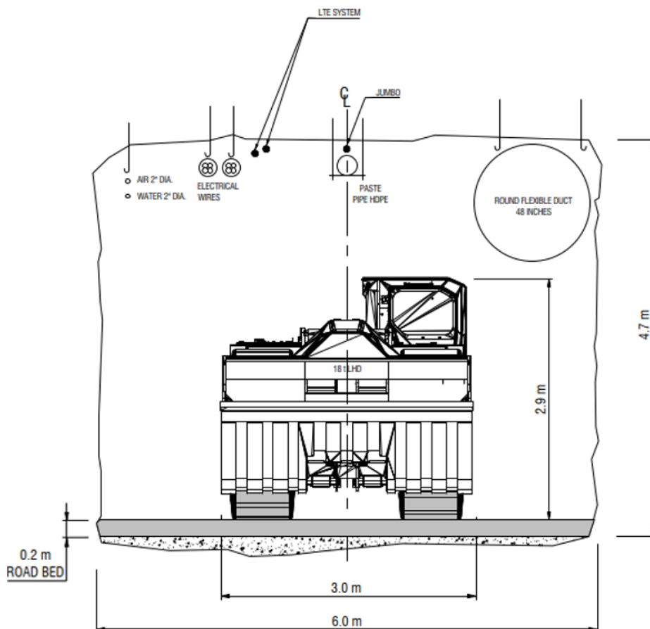
Figure 16.36: Typical Development Section of a Draw Point
