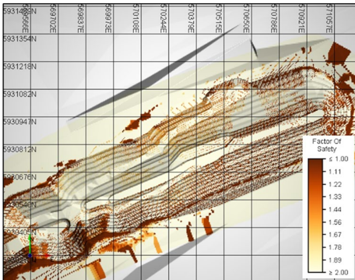
Figure 16.4: Static Factor of Final Pit Slopes' Safety from 3D Model
