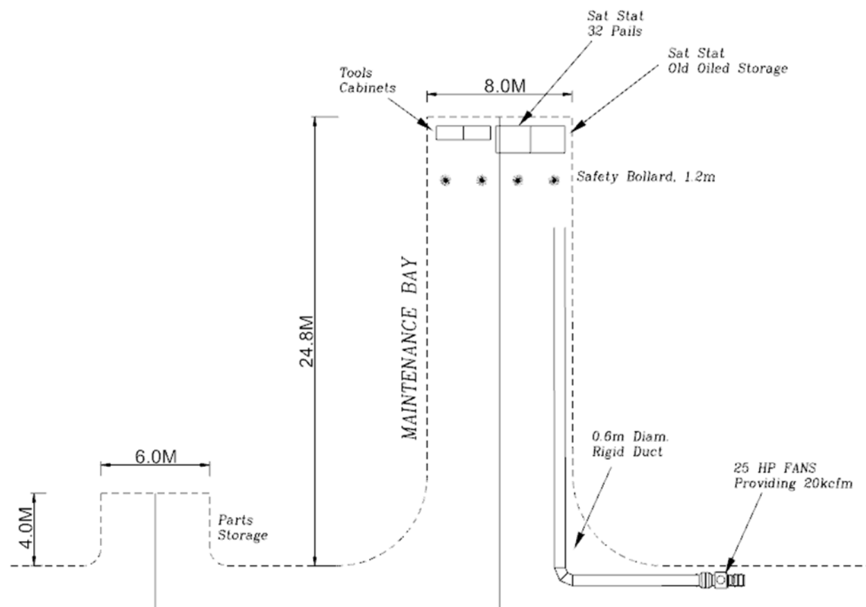
Figure 16.69: Typical Maintenance Bay
