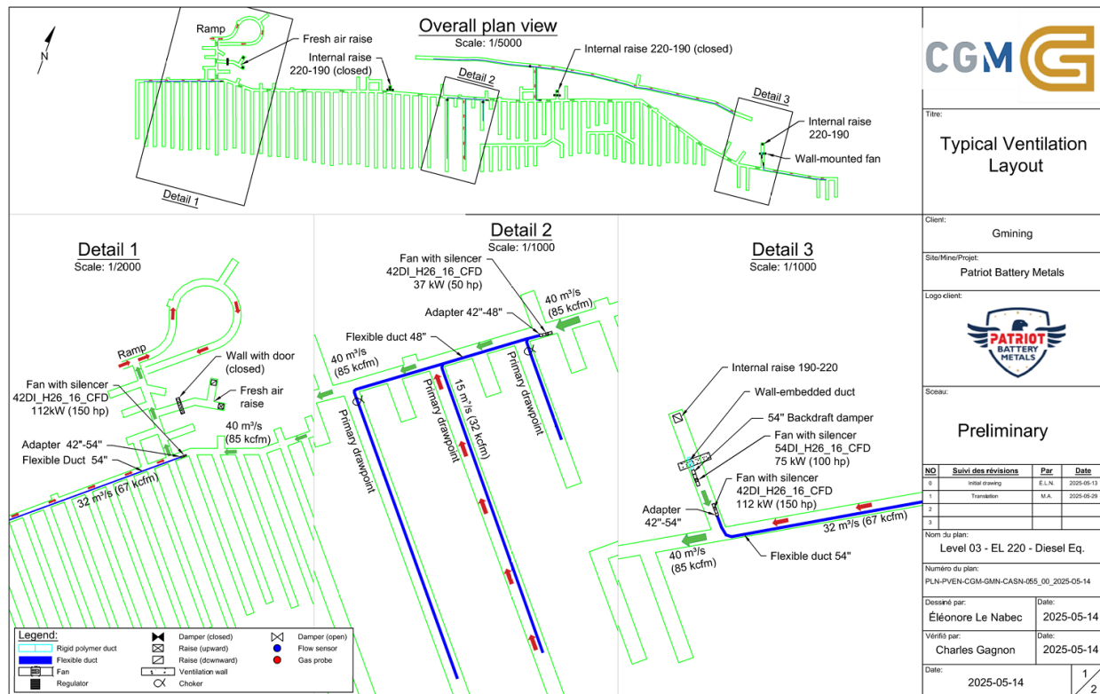
Figure 16.59: Typical Ventilation Layout
