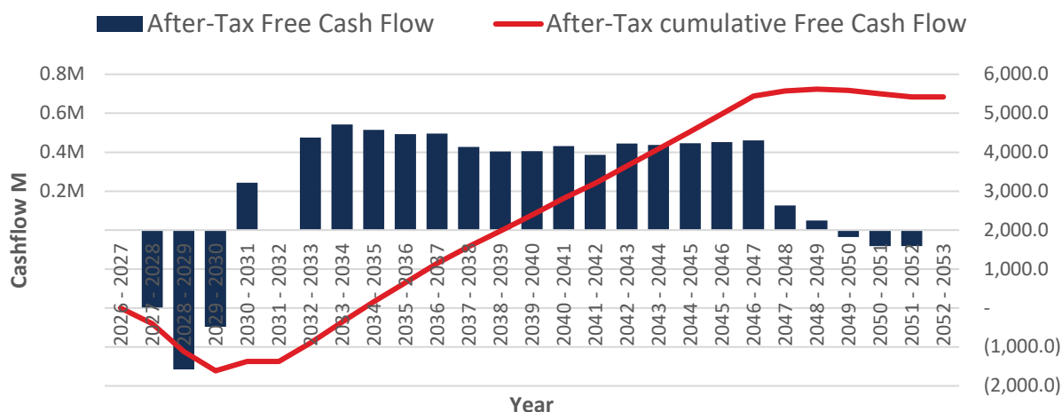
Figure 22.9: Life of Mine After-Tax Cumulative Cash Flow Projection
