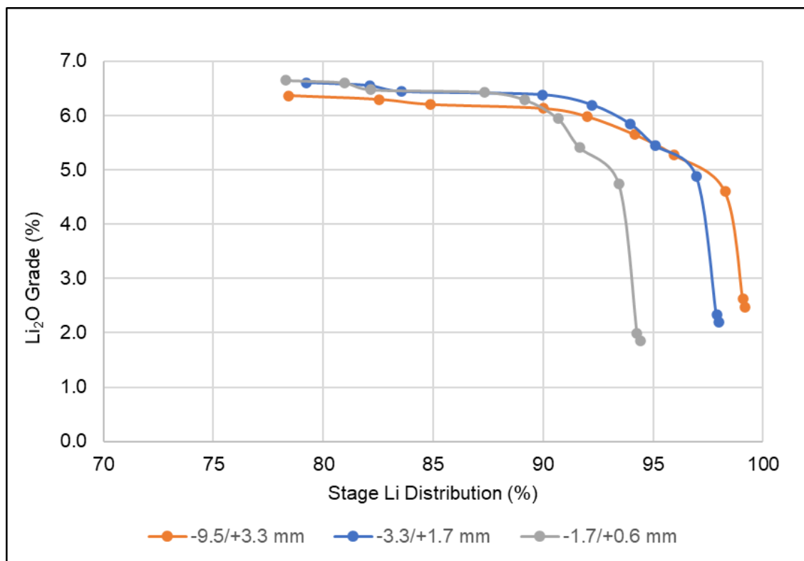
Figure 13.9: Stage HLS Results
