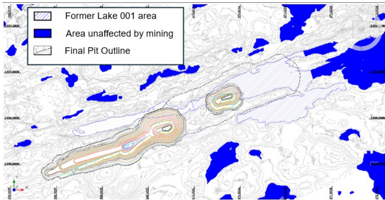
Figure 16.12: Phase 3B Open Pit Design – Plan View
