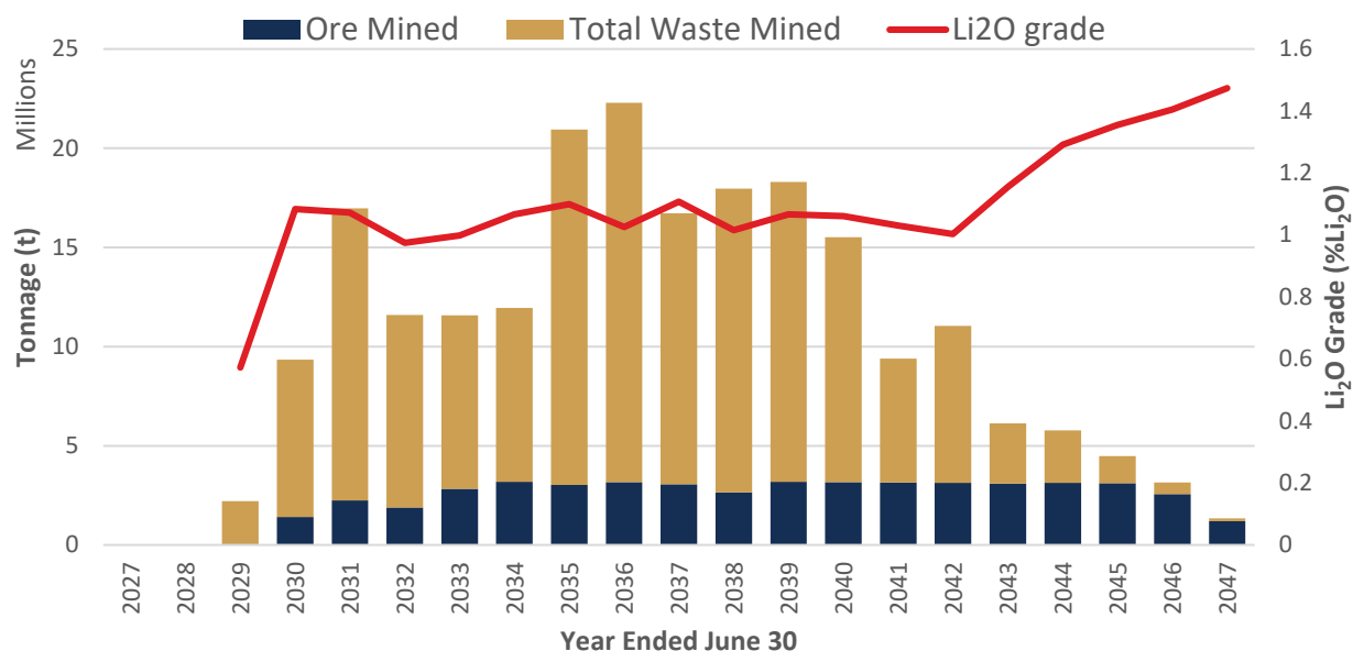
Figure 22.5: Open Pit Mine Production Profile
