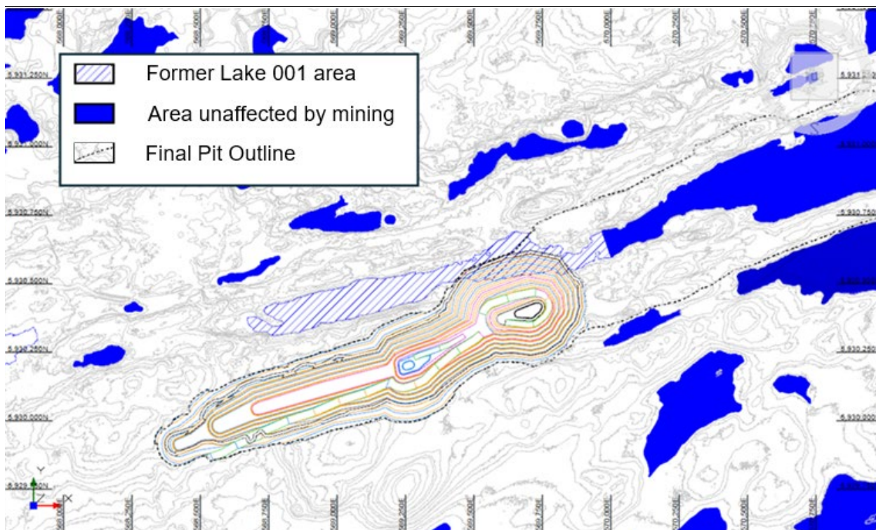
Figure 16.10: Phase 2 Open Pit Design – Plan View
