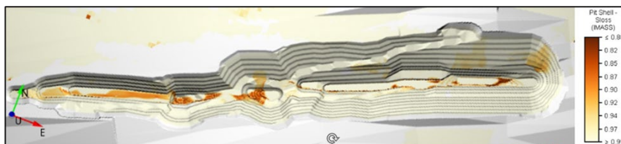
Figure 16.5. Damage Indicator (Sloss) on Final Pit Slopes from 3D Model
