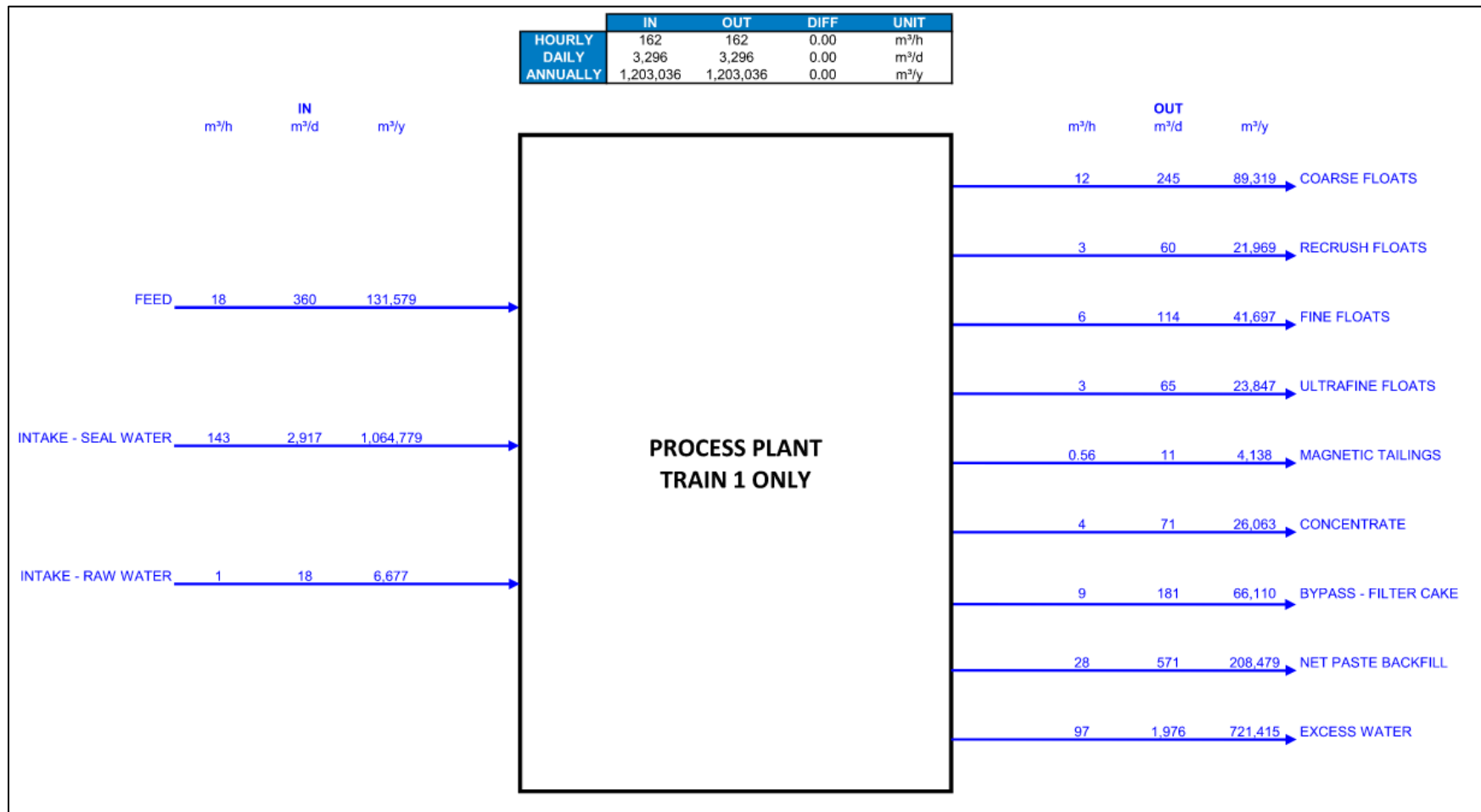
Figure 17.2: Mineral Processing Facility Simplified Water Balance
