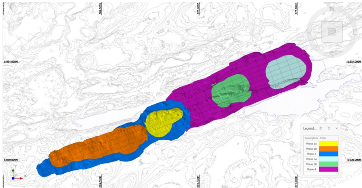
Figure 1.4: Open Pit Phase Limits – Plan View
