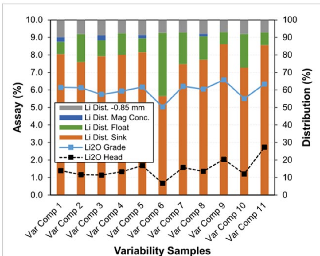
Figure 13.6: Global HLS Results for Variability Composite Samples
