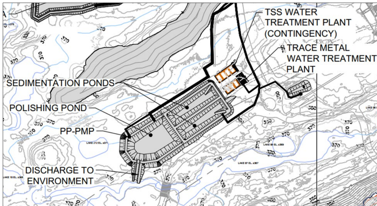
Figure 18.43: Water Treatment Pond and Plants
