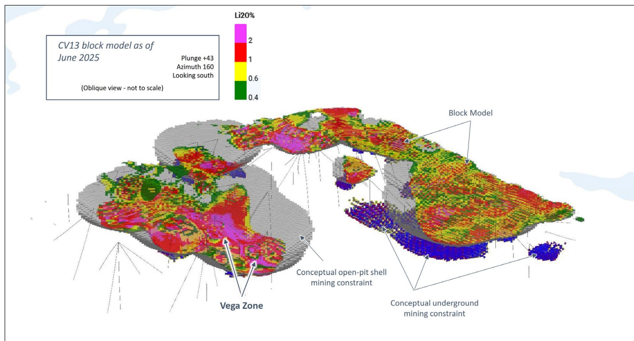
Figure 14.10: CV13 Open Pit and Underground Constraints to MRE Block Model
