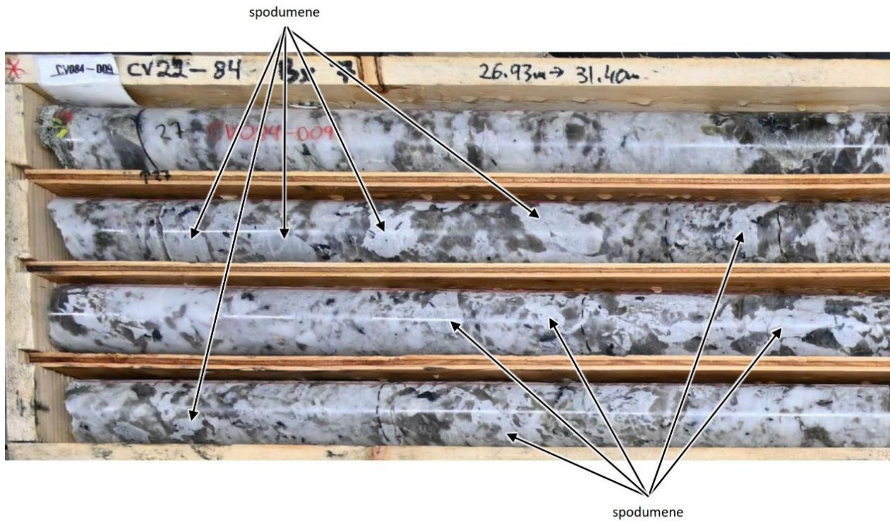
Figure 7.19: Coarse-grained Spodumene Crystals in Drill Core from CV13
