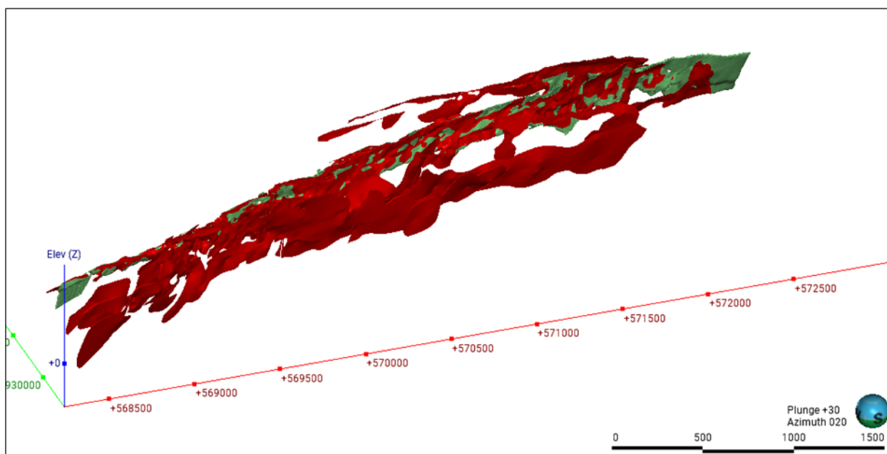
Figure 14.4: CV5 Mineralized Zones
