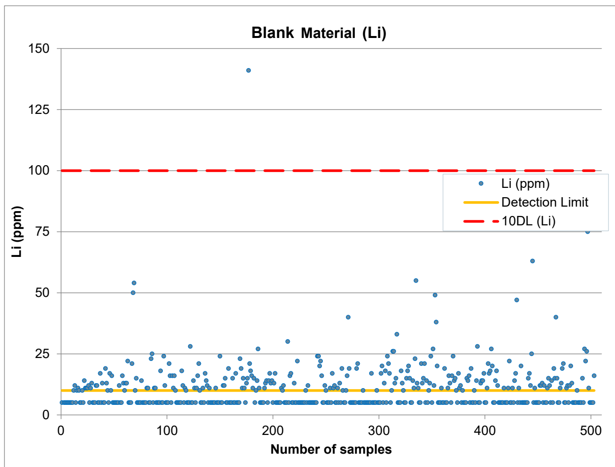
Figure 11.1: Blank Sample Results (Li) from the 2024 Drilling Campaign
