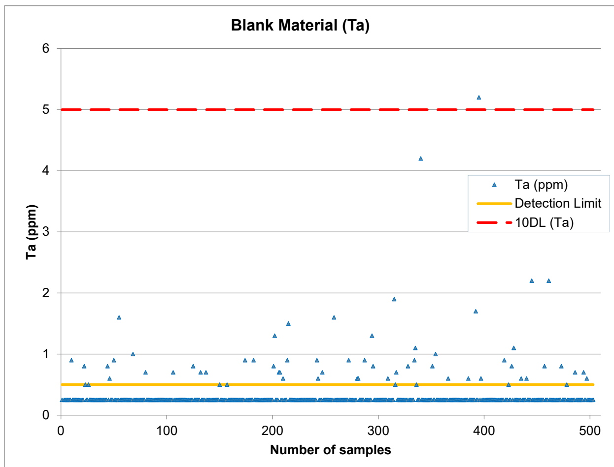
Figure 11.2: Blank Sample Results (Ta) from the 2024 Drilling Campaign
