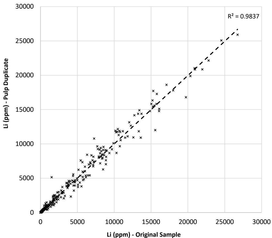
Scatterplot Between Pulp Duplicates and Original Samples
