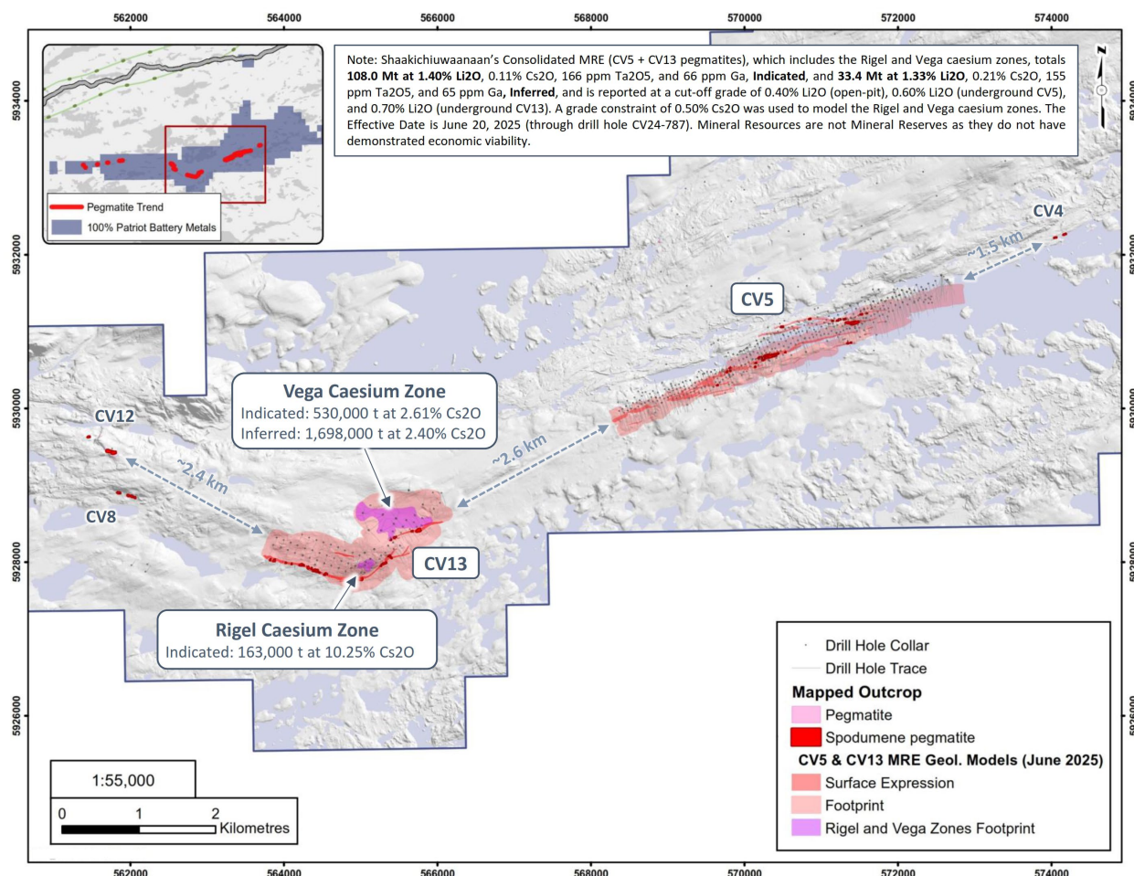
Figure 10.4: Drill Holes Completed Through 2024 at the CV5 and CV13 LCT Pegmatites
