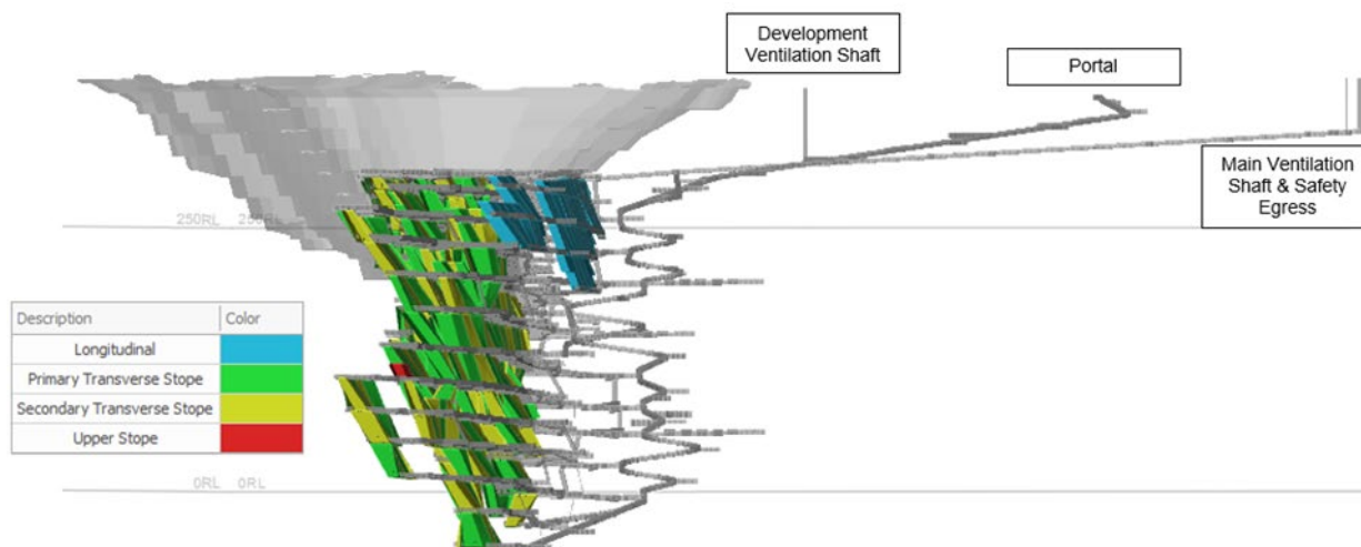
Figure 16.43: Underground Mine Longitudinal View by Mining Method - Looking 289° W
