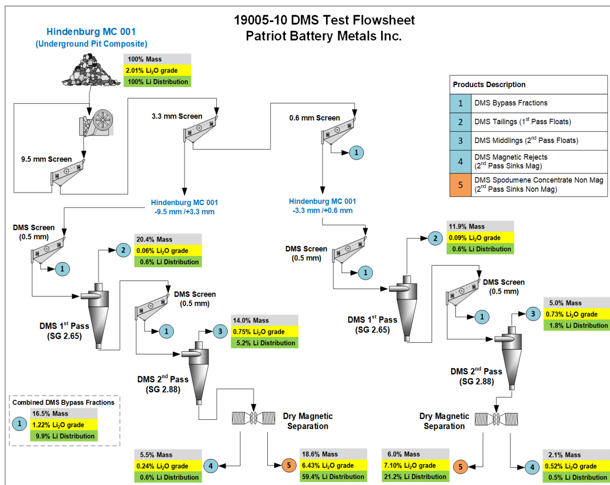
Figure 13.13: DMS Testwork Flowsheet
