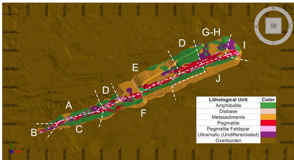
Figure 15.1: Geotechnical Domains by Lithology and Orientation (from Alius, 2025)
