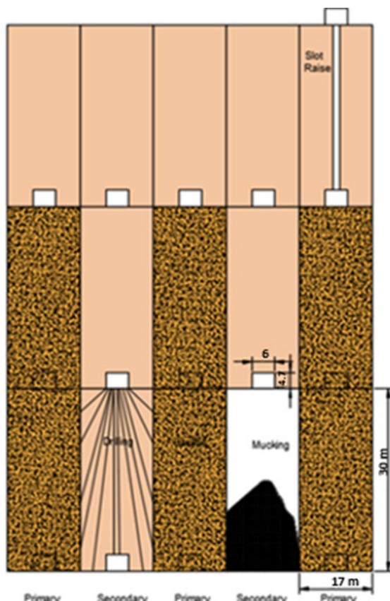
Figure 16.29: Representation of Transverse LHOS Mining Method
