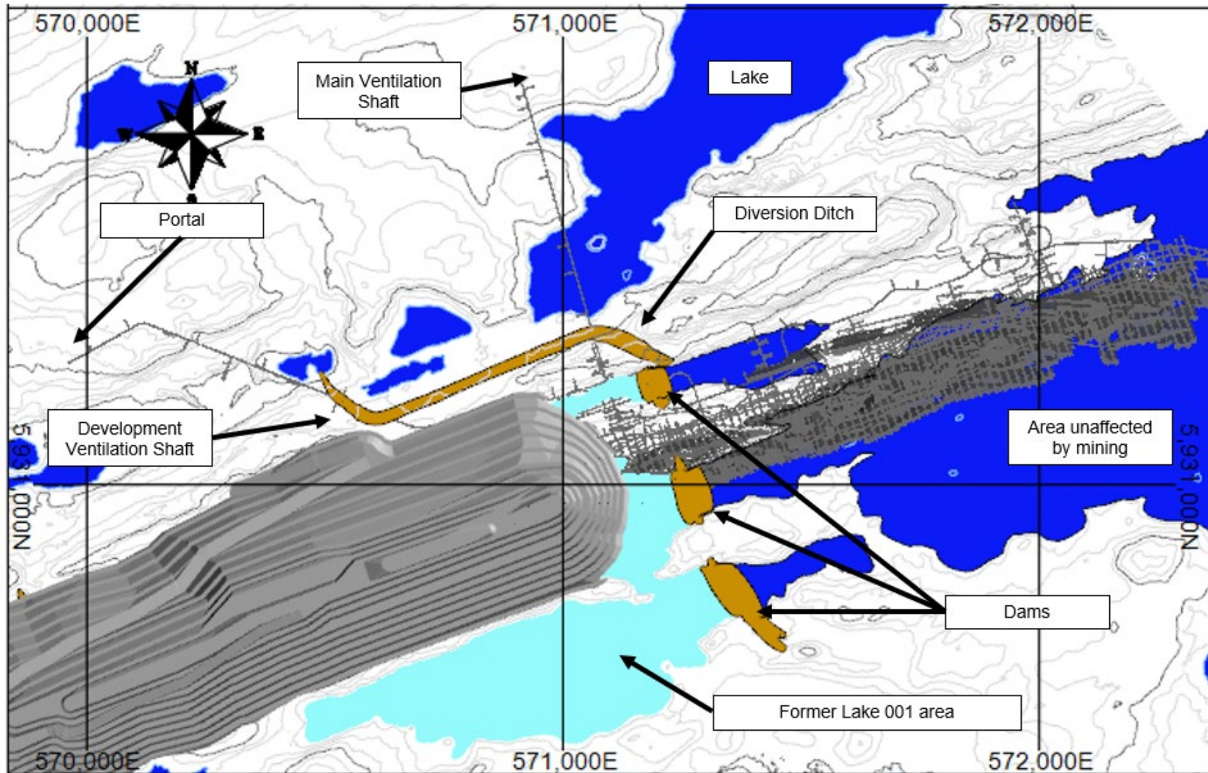
Figure 16.41: Underground Mine and Surface Constraints – Plan View
