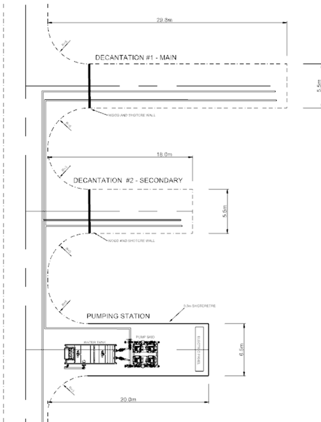
Figure 16.63: Typical Underground Decantation and Pumping Bays
