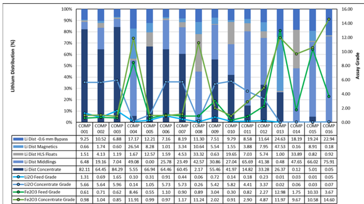
Figure 13.7: Test Program 19005-02A HLS Testwork Results
