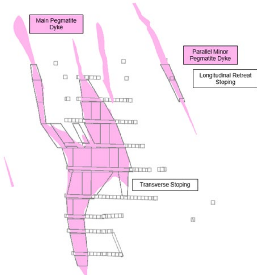
Figure 16.42: Stopping and Pegmatites - Looking West - Section at Easting 571,647
