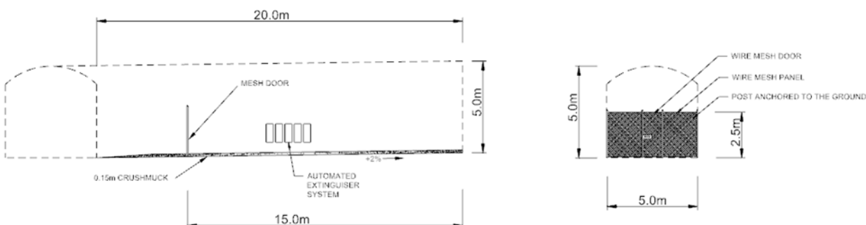
Figure 16.67: Typical Cross-section of Bulk Emulsion Truck Parking
