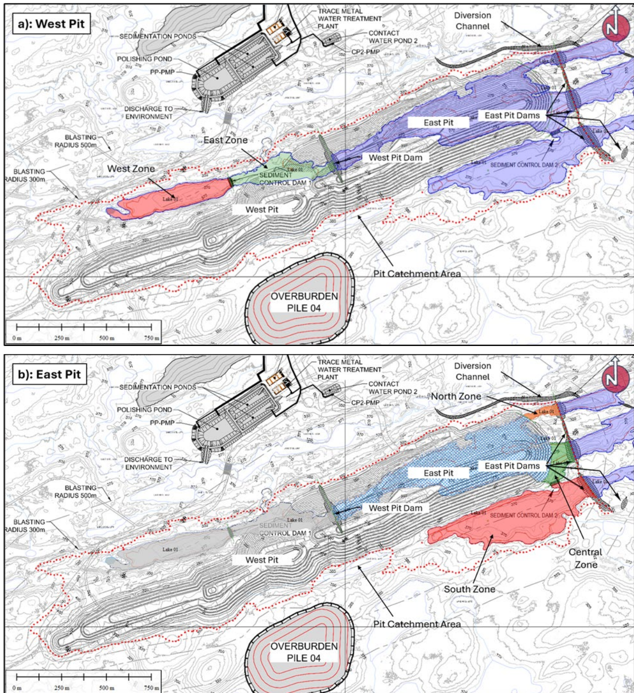
Figure 18.42: Open Pit (West Pit and East Pit) Sediment and Water Management Layouts
