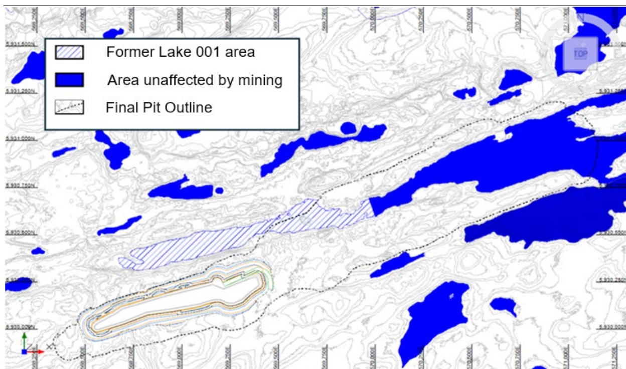
Figure 16.9: Phase 1B Open Pit Design -Plan View
