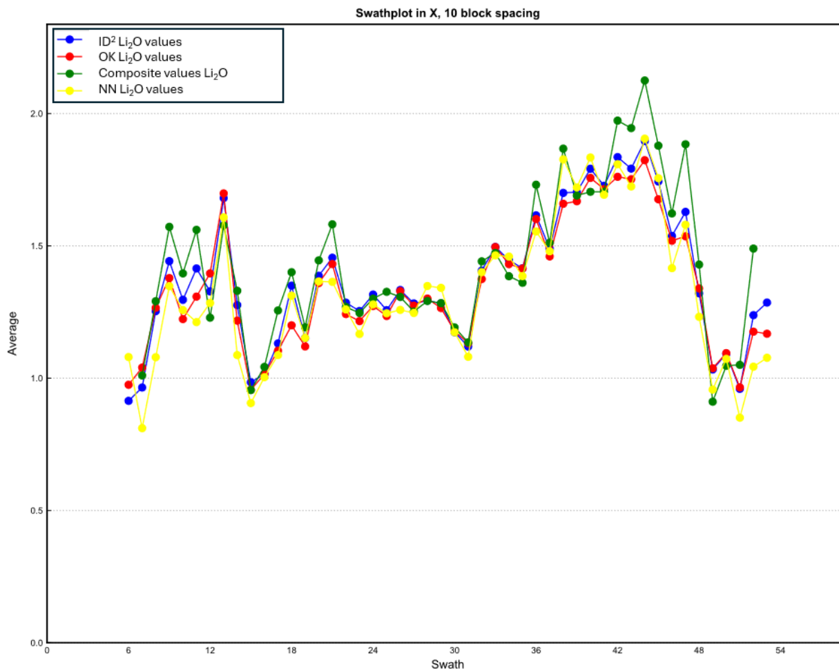
Figure 14.16: Li 2 O Swath Plot in X Direction (CV5 Zone 100)
