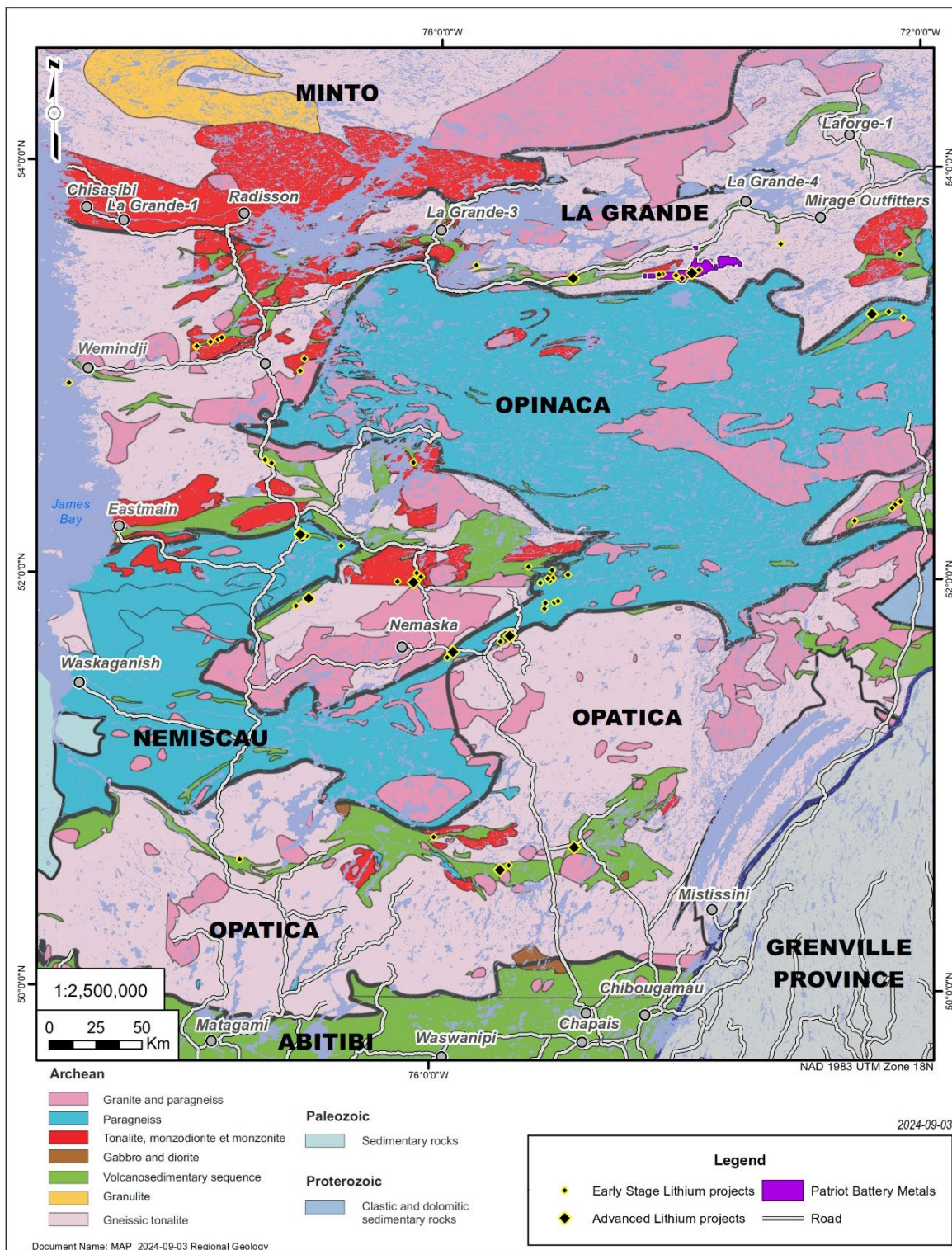
Figure 7.1: Regional Geology
