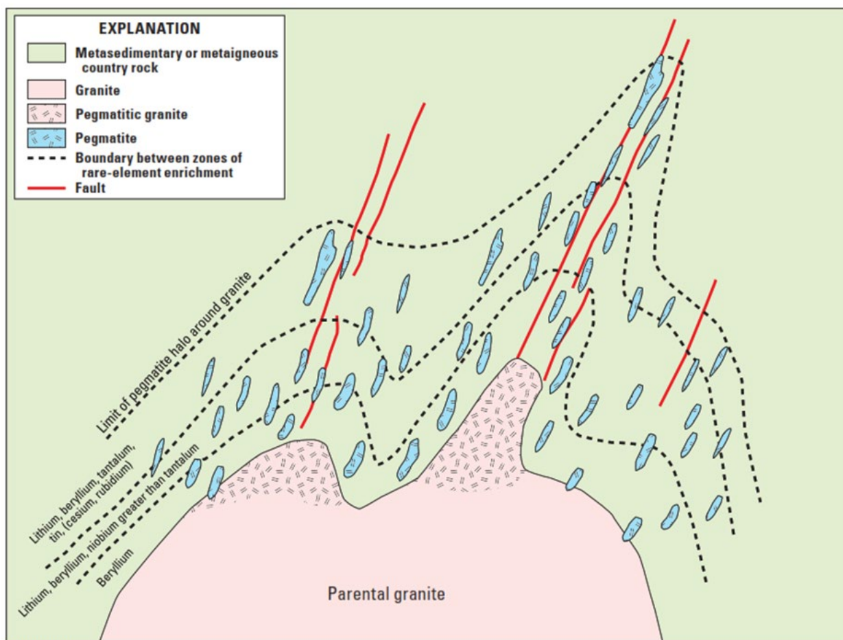
Figure 8.1: LCT Pegmatite Deposit Model
