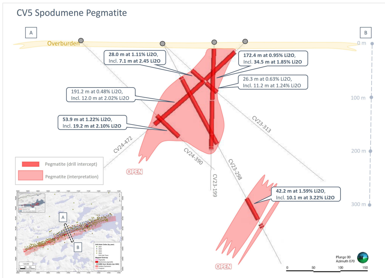
Figure 7.15: Simplified Cross-Section of CV5 Pegmatite Geological Model
