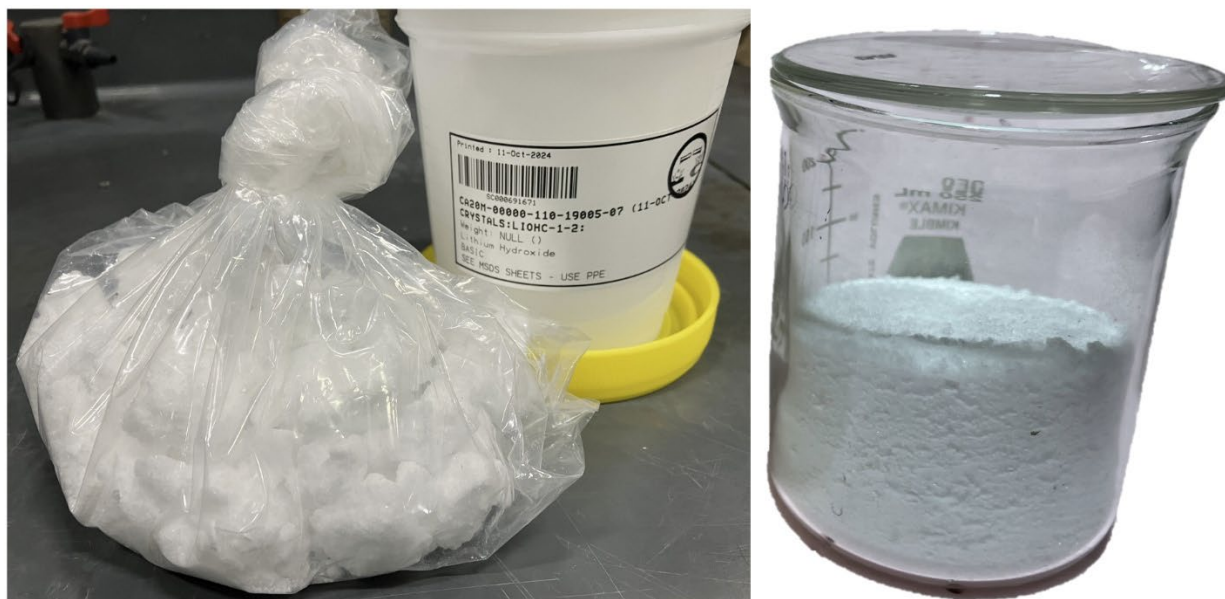
Figure 13.19: On Spec Battery-Grade Lithium Hydroxide Monohydrate Product
