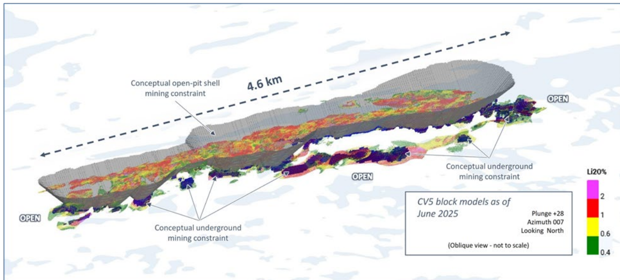
Figure 14.9: Oblique View of the CV5 Spodumene Pegmatite Block Model with Respect to Applied OP and UG Conceptual Mining Constraint Shapes
