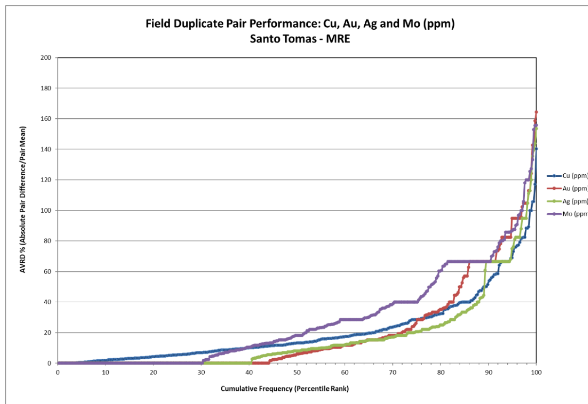
Figure 11-10: FDUP Cumulative Frequency vs. AVRD Plot for Cu, Au, Ag, and Mo
