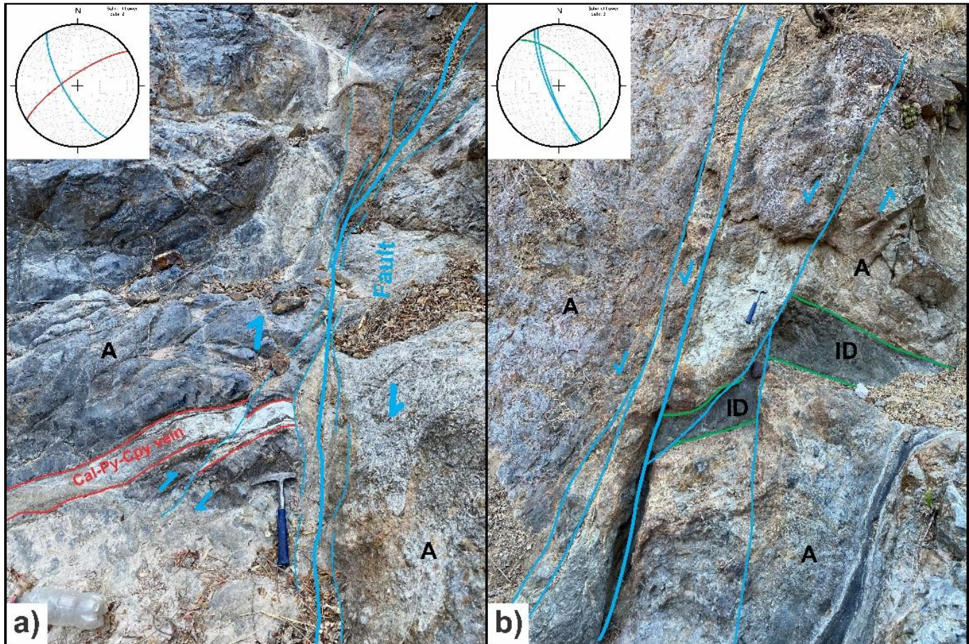
Figure 7-12: a) Plan view of dextral fault cutting and displacing vein mineralized with calcite-pyrite-chalcopryrite. b) Section view looking NNE of normal fault cutting and displacing intermediate-mafic dike and andesitic rocks. ID: intermediate-mafic dike; A: andesite. The structures measured on the faults, contact and vein are plotted in the stereonet. The color of the lines in the stereonets represents the color of the structure on the image
