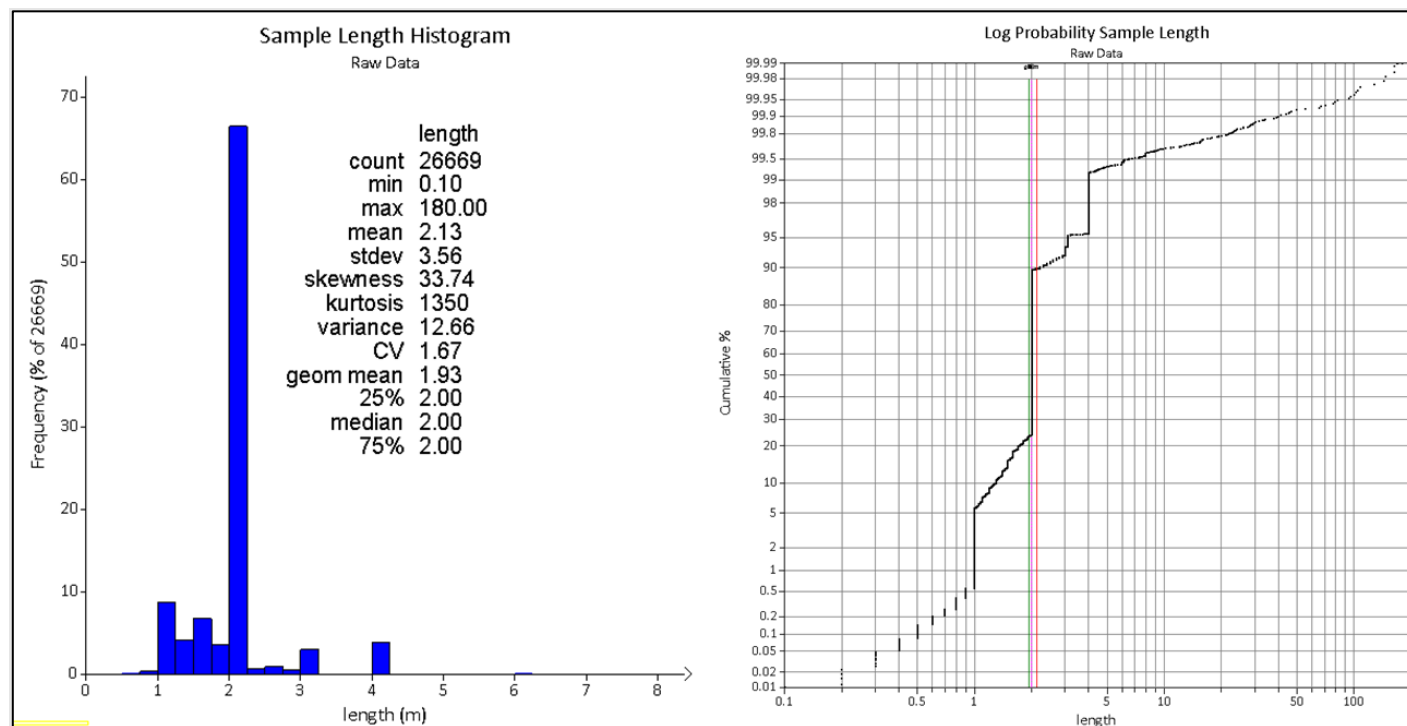
Figure 14-10: Raw Sample Interval Histogram (left) and Log-Probability (right)
