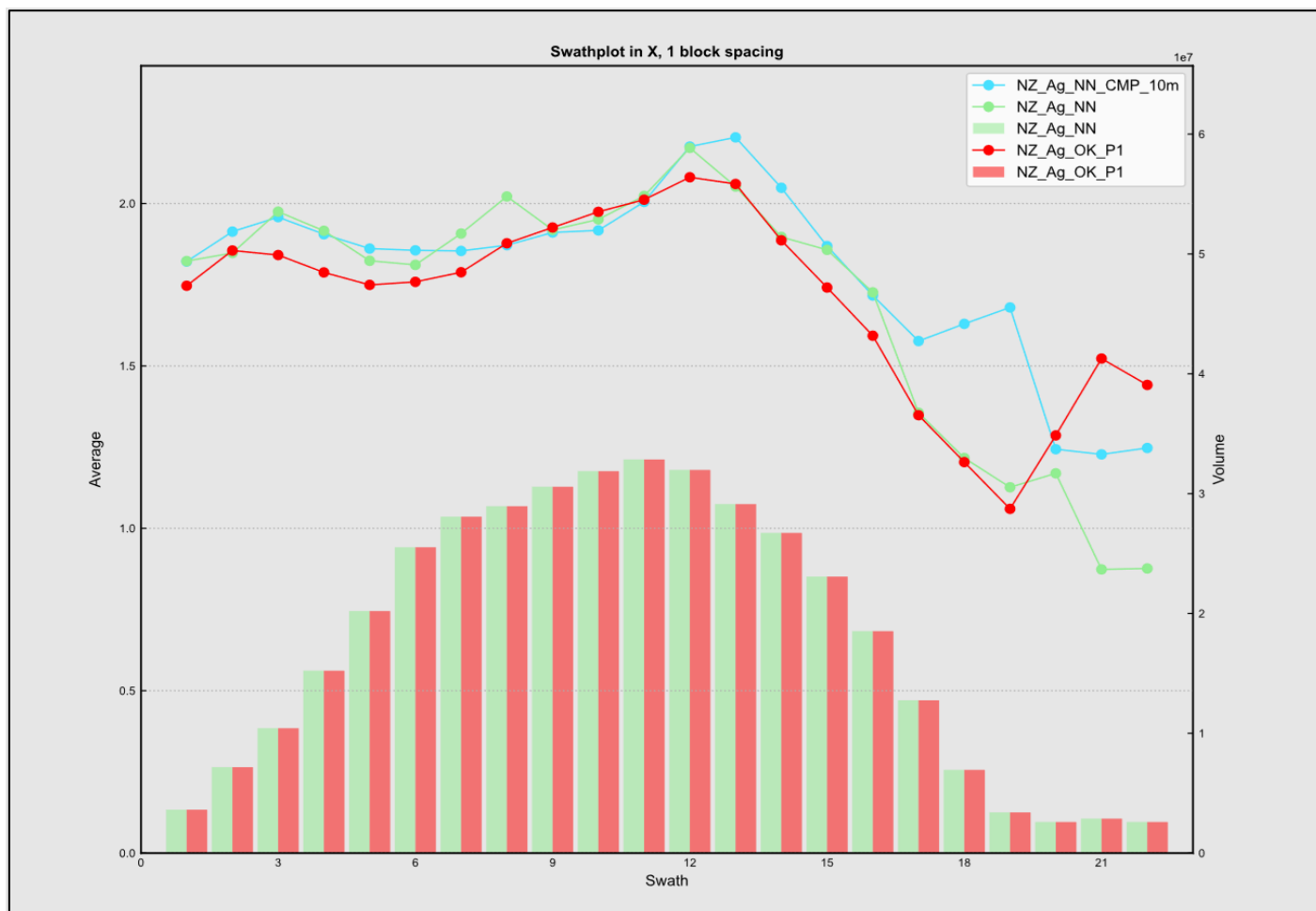
Figure 14-37: Swath plot in X direction - North Zone Ag
