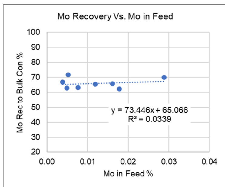
Figure 13-5: Molybdenum Recovery vs. Head Grade
