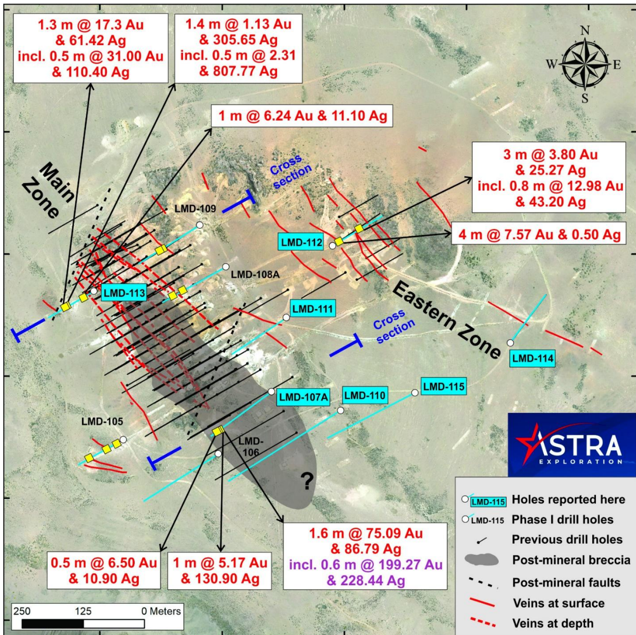
Figure 1: Plan map of Phase I drill results for seven holes (107A, 110, 111, 112, 113, 114, & 115) at La Manchuria. Gold and silver results are in grams per tonne (g/t).
