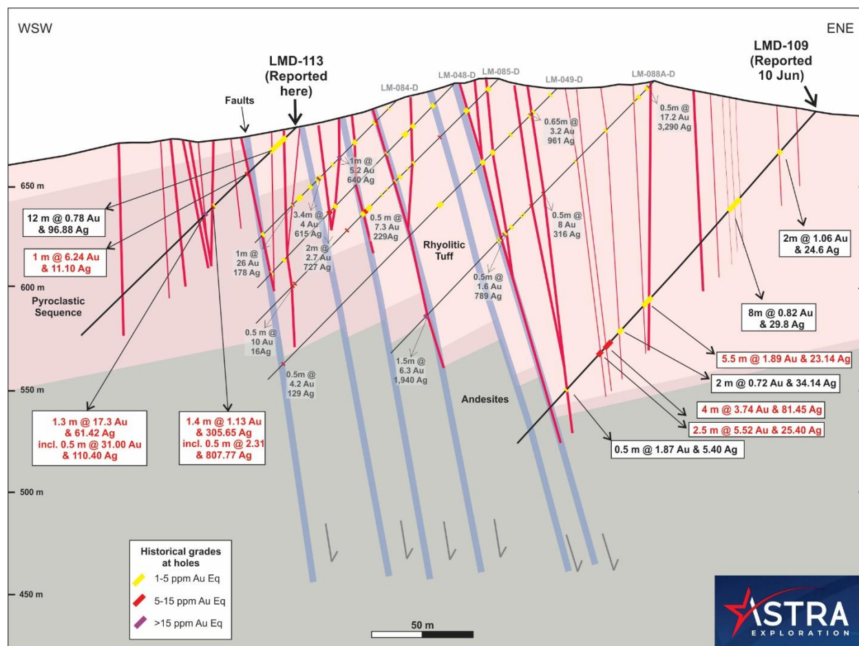
Figure 3: Schematic cross section through the Main zone at La Manchuria showing hole LMD-113 (and previously reported LMD-109) drill results.
