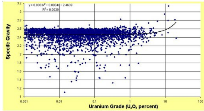
Figure 8-1: Logarithmic Plot of Dry Bulk Density versus Uranium Grade in Corresponding Geochemical Samples
