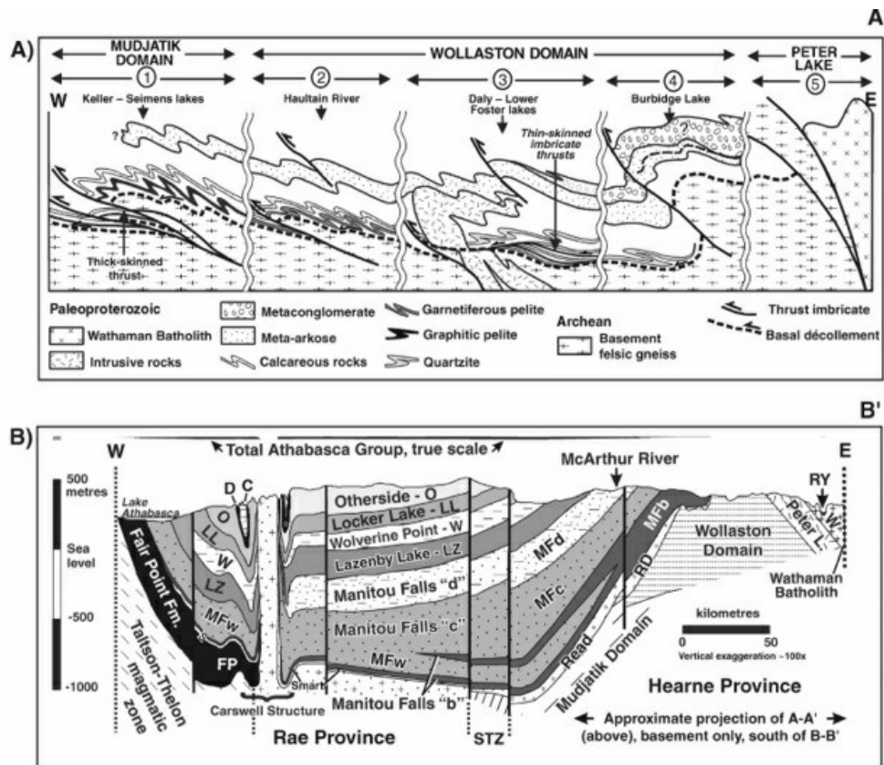
Figure 6-4: A) Idealized cross-section through the eastern Cree Lake zone, suggesting the possible structural relationship between Archean basement and Paleoproterozoic metasedimentary cover during the early stages of Hudsonian deformation (after Tran, 2001); B) Geological cross-section through the Athabasca Basin (after Ramaekers, 1990; Ramaekers et al. 2007). For location see Figure 6-3.
