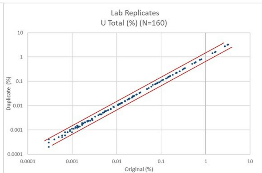
Figure 8-11: XY Chart for Lab Replicates Analyzed for Uranium at SRC 2009
