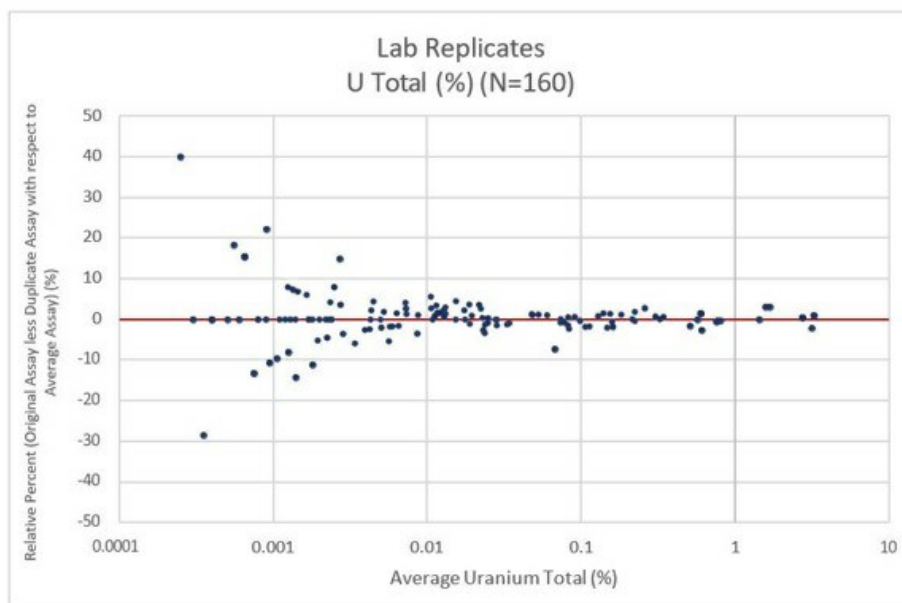
Figure 8-12: RPD Chart for Lab Replicates Analyzed for Uranium at SRC 2009
