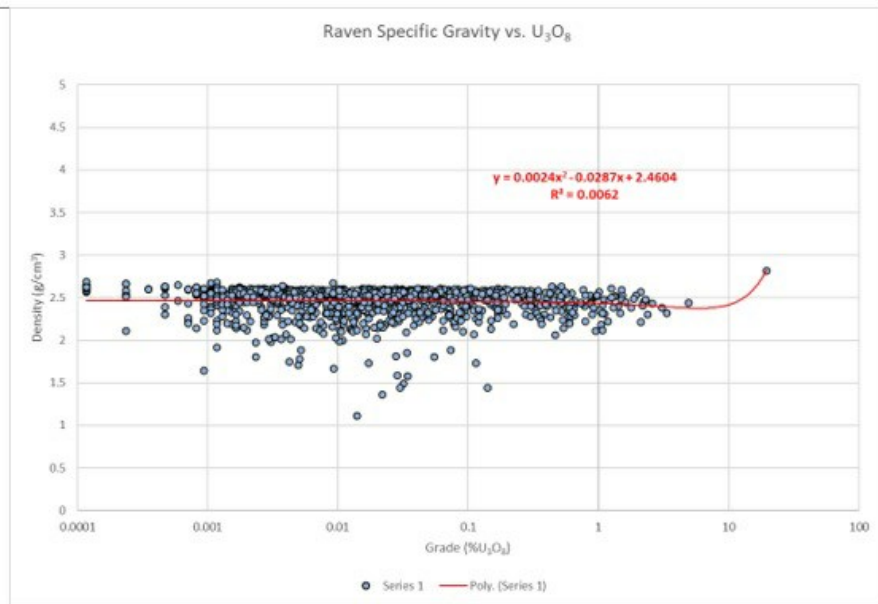
Figure 11-6: Raven Density vs U 3 O 8
