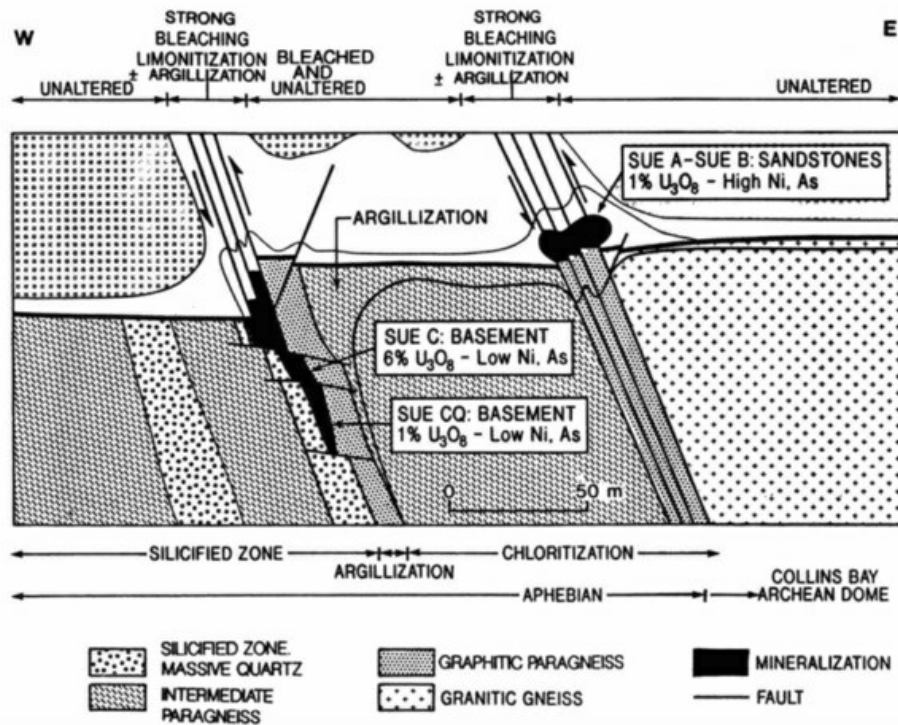
Figure 6-6: Types of Unconformity-Type Uranium Deposits
