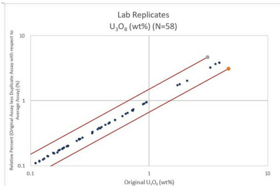
Figure 8-13: XY Chart for Lab Replicates Analyzed for Uranium SRC 2011
