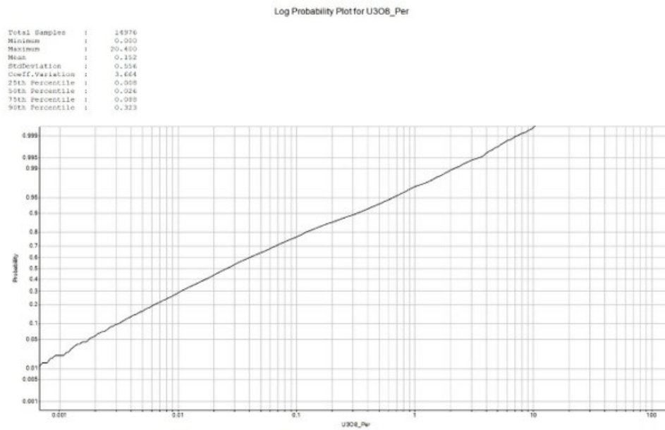
Figure 11-7: Log Probability Plot for Horseshoe Composite and Trimmed Assays
