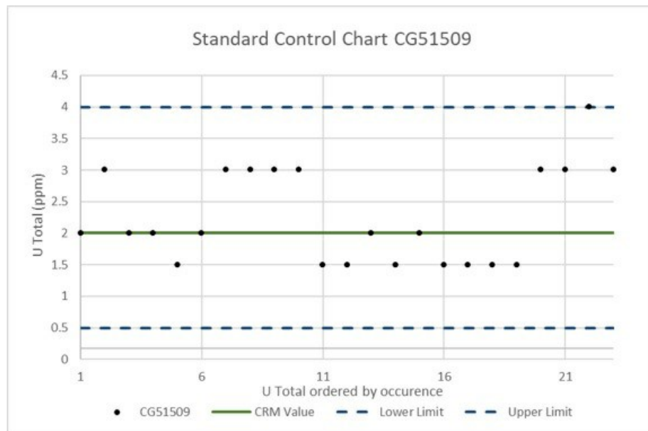
Figure 8-4: Control Chart for Reference Material CG51509* analyzed for Uranium at SRC
