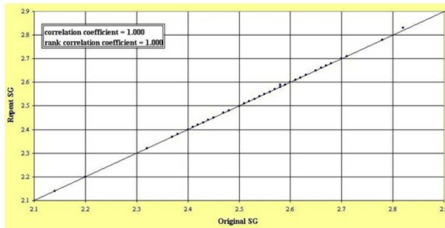
Figure 8-3: Quantile - Quantile Plot of Laboratory Bulk Density Replicated for Batches Submitted between September 2008 and June 2009
