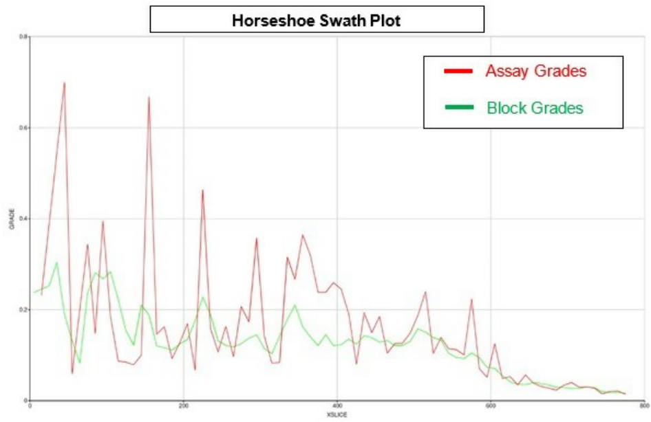
Figure 11-11: Horseshoe Swath Plot in the X Direction
