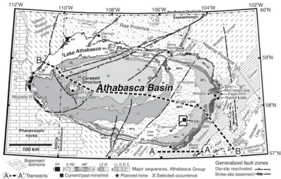
Figure 6-3: Geological Sketch Map of the Athabasca Basin. The eastern Athabasca Basin is defined as that part of the basin east of the Snowbird tectonic zone and is shown in reference to the major basement domains and stratigraphy of the Athabasca Basin, after Card et al. 2007, Portella and Annesley (2000), Ramaekers et al. (2007) and Thomas et al. (2002).
