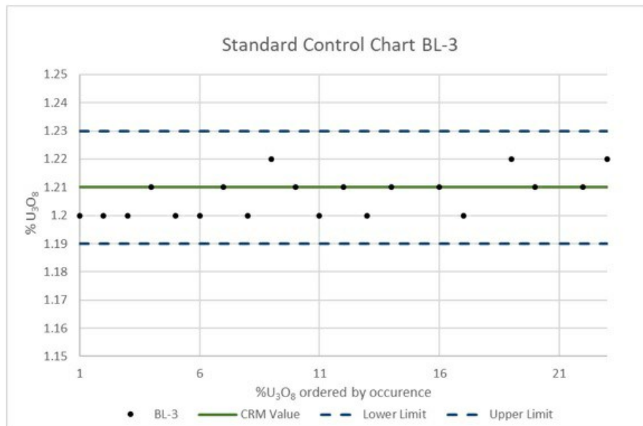
Figure 8-7: Control Chart for Reference Material BL-3* analyzed for Uranium and %U 3 O 8 at SRC
