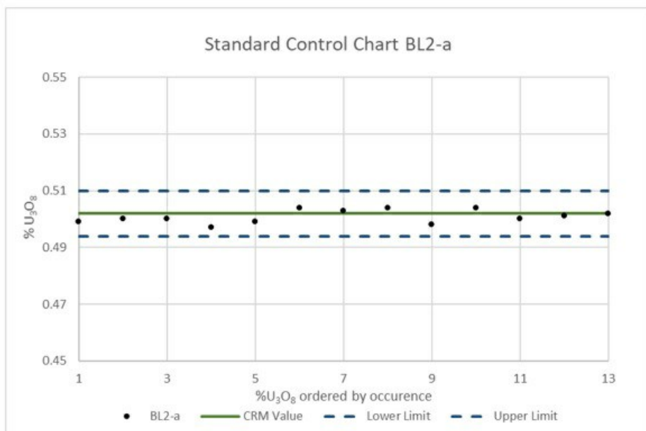
Figure 8-6: Control Chart for Reference Material BL-2a analyzed for %U3O8 at SRC
