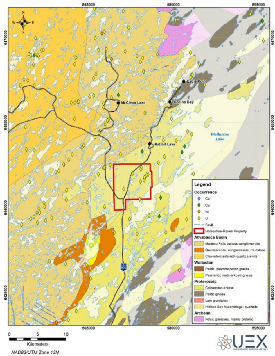
Figure 6-5: Horseshoe-Raven Property Local Geology
