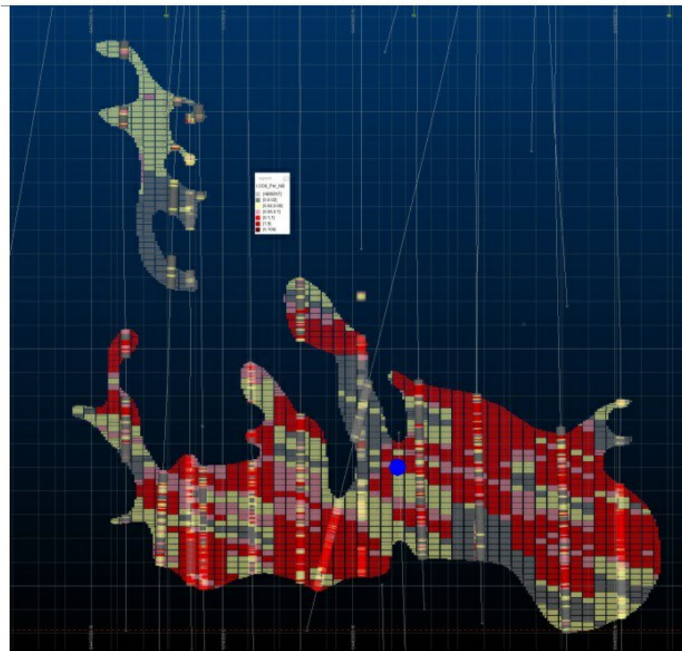
Figure 11-9: Horseshoe Visual Check of Drillhole Grades against Block Grades (Section Orientation of 335°)
