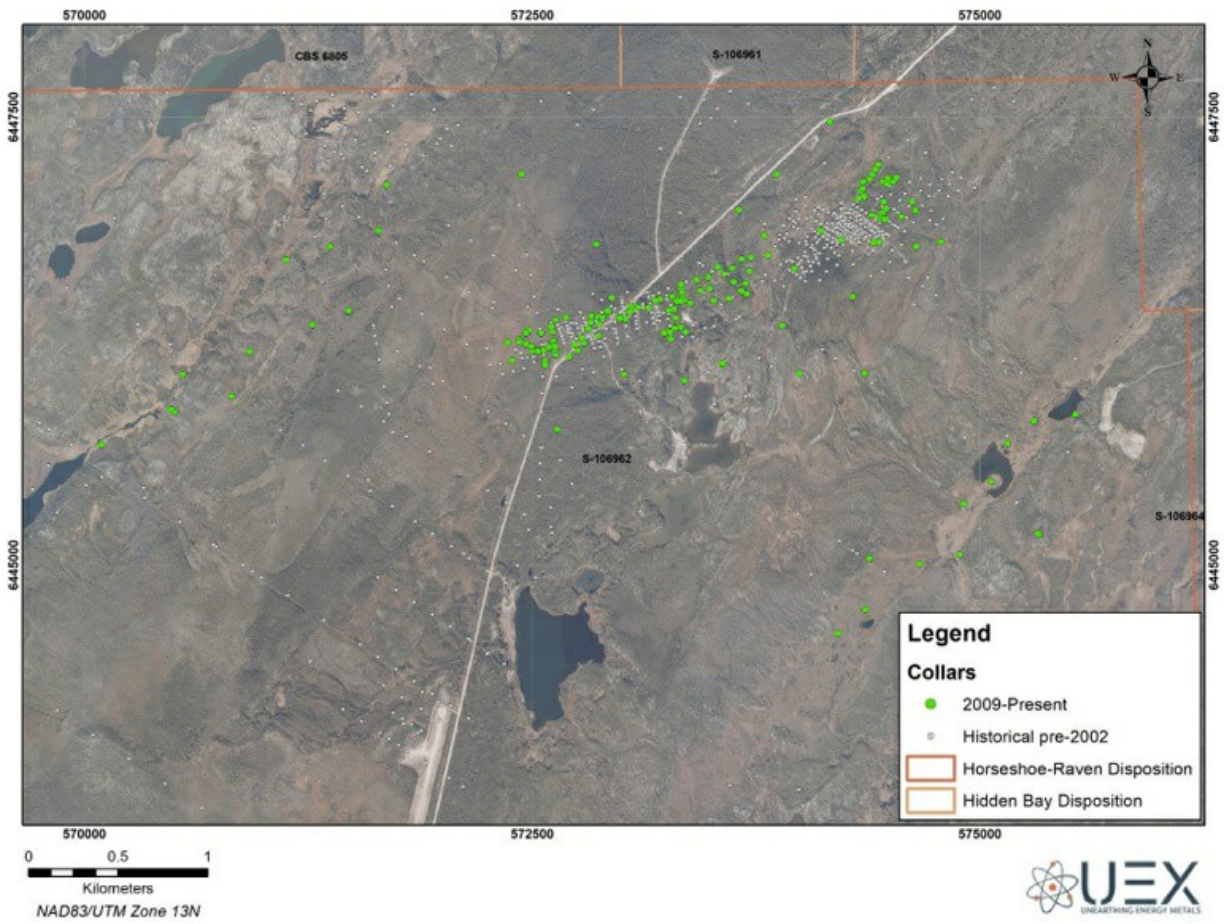
Figure 7-2: Recent Historical Drilling on the Horseshoe-Raven Property
