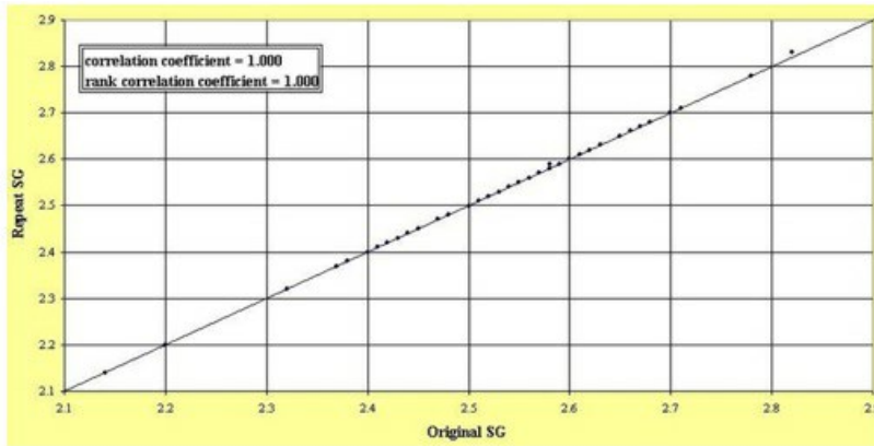
Figure 8-2: Quantile - Quantile Plot of Laboratory Bulk Density Replicated for Batches Submitted for all Seasons Prior to September 2008
