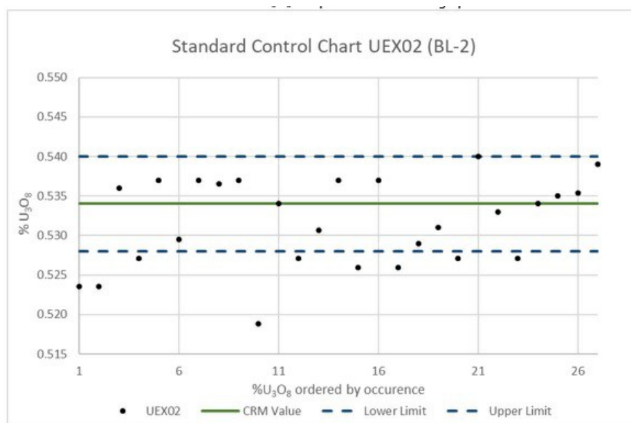
Figure 8-10: Control Chart for Reference Material UEX02* analyzed for Uranium and %U3O8 at SRC
