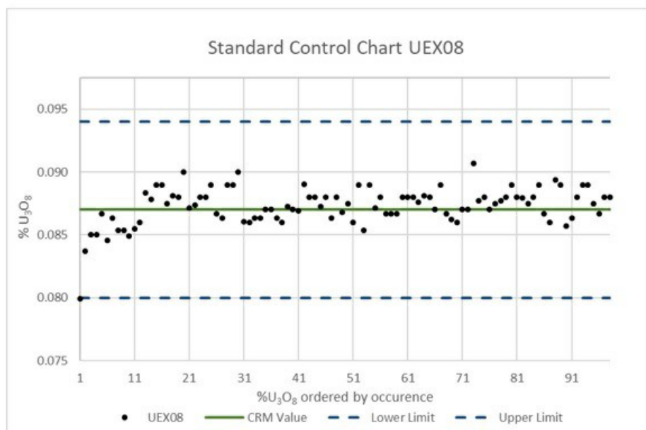
Figure 8-9: Control Chart for Reference Material UEX08* analyzed for Uranium and %U3O8 at SRC
