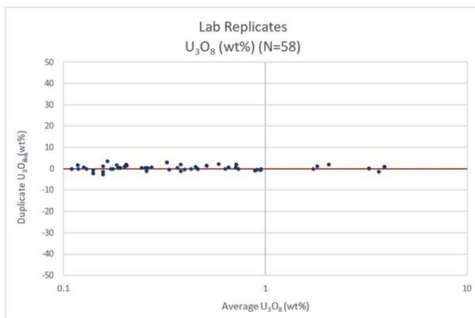
Figure 8-14: RPD Chart for Lab Replicates Analyzed for Uranium SRC 2011
