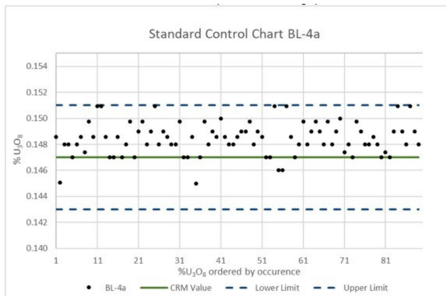
Figure 8-8: Control Chart for Reference Material BL-4a* analyzed for Uranium and %U 3 O 8 at SRC
