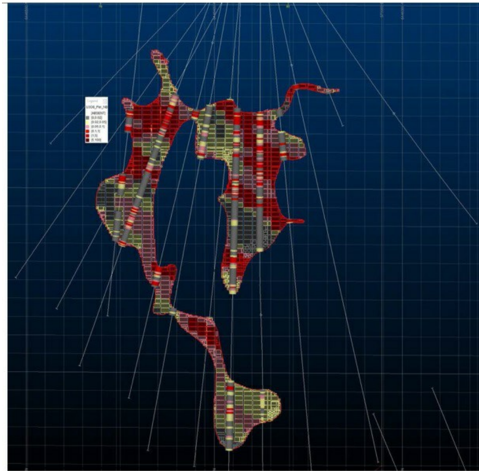
Figure 11-10: Raven Visual Check of Drillhole Grades against Block Grades (Section Orientation of 345°)
