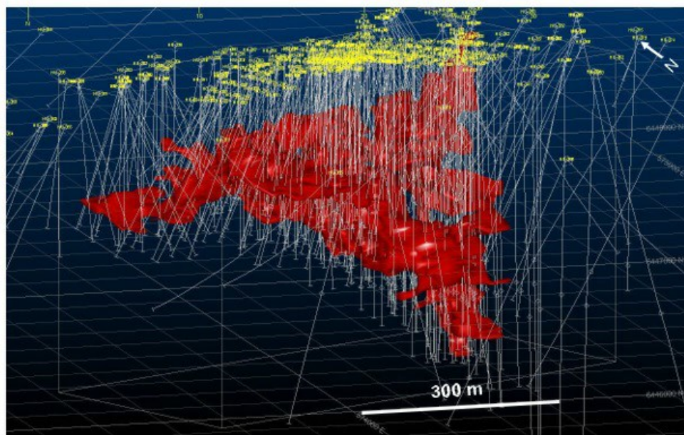
Figure 11-2: Horseshoe Wireframe Isometric View (Looking NNE)
