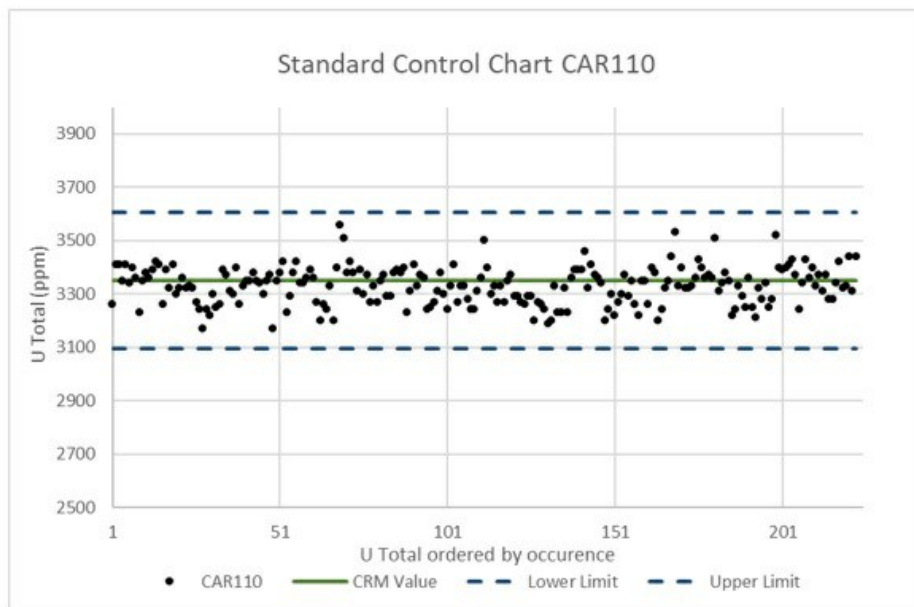
Figure 8-5: Control Chart for Reference Material CAR110 analyzed for Uranium at SRC
