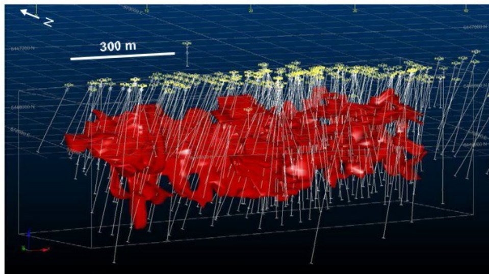
Figure 11-4: Raven Wireframe Isometric View (Looking NNE)
